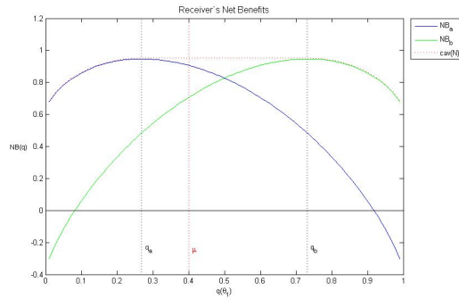
Figure 3.3 – Net Benefits and cav(N)(p)
