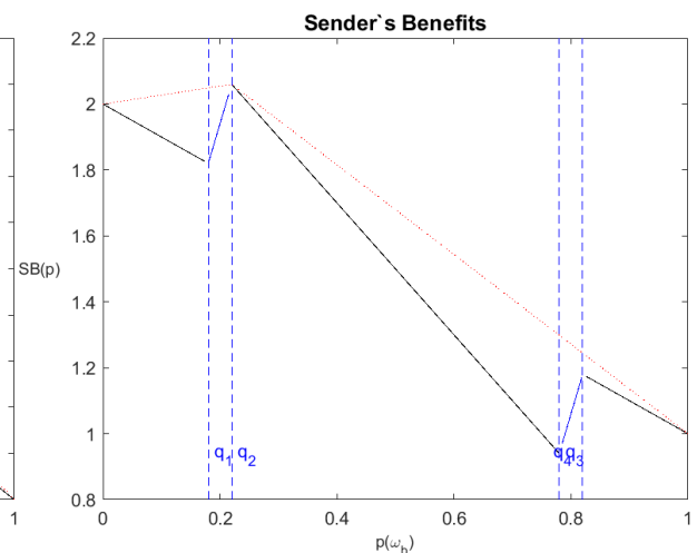
Figure 3.6 – Sender's Solution for \lambda' < \lambda
