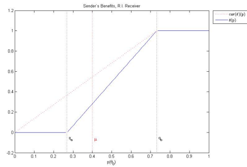
Figure 3.4 – Functions \hat{v}(p) and cav(\hat{v})(p)
