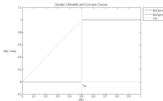
Figure 3.2 – Sender's Expected Benefits
