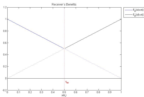
Figure 3.1 – Receiver's Expected Benefit
