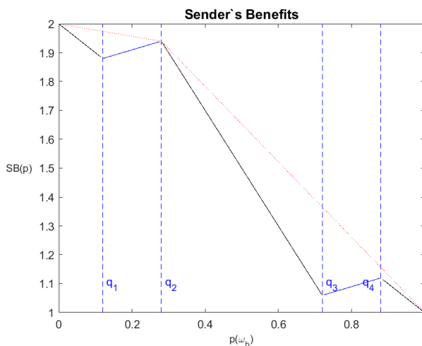
Figure 3.5 – Sender's Solution for \lambda
