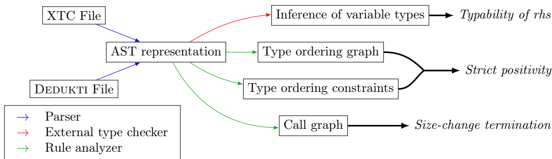
Figure 7.1: SIZECHANGETOOL Workflow
