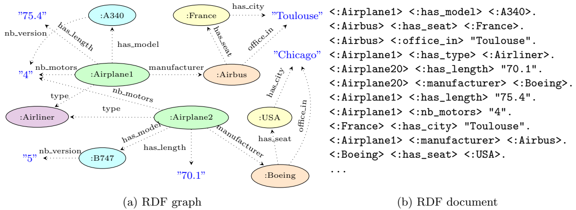
Figure 2.10: RDF example
