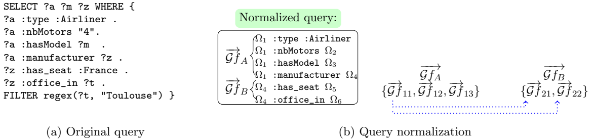
Figure 4.19: Normalization process
