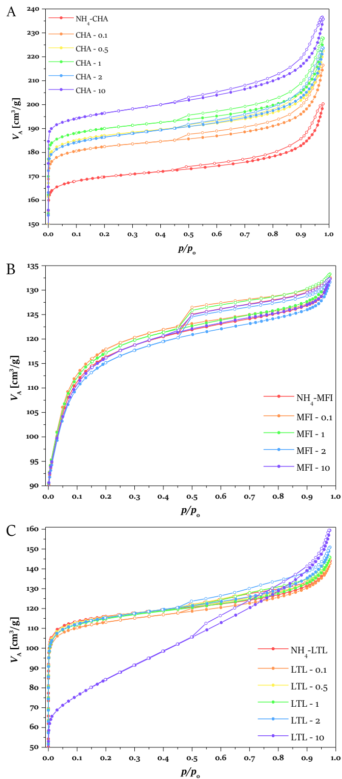
Figure 6.4. N_2 physisorption isotherms of A) \text{NH}_4 -CHA, B) \text{NH}_4 -MFI, and C) \text{NH}_4 -LTL with their etched derivatives. Note: the y-axis starts at higher values of V_A to highlight the changes in the micropore area.
