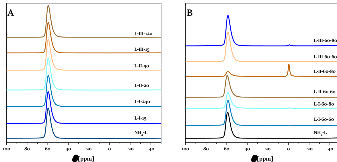
Figure 4.6. The ^{27}\text{Al} MAS NMR of the parent zeolite and derivatives treated at A) room temperature and B) 60 and 80 °C, with 20 (L-I), 40 (L-II) wt/% \text{NH}_4\text{F} , and 1 wt/% \text{NH}_4\text{HF}_2 (L-III) solutions.
