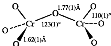
Figure 6.1. Structure of the dichromate ion found in \text{Rb}_2\text{Cr}_2\text{O}_7 (from [15]).
