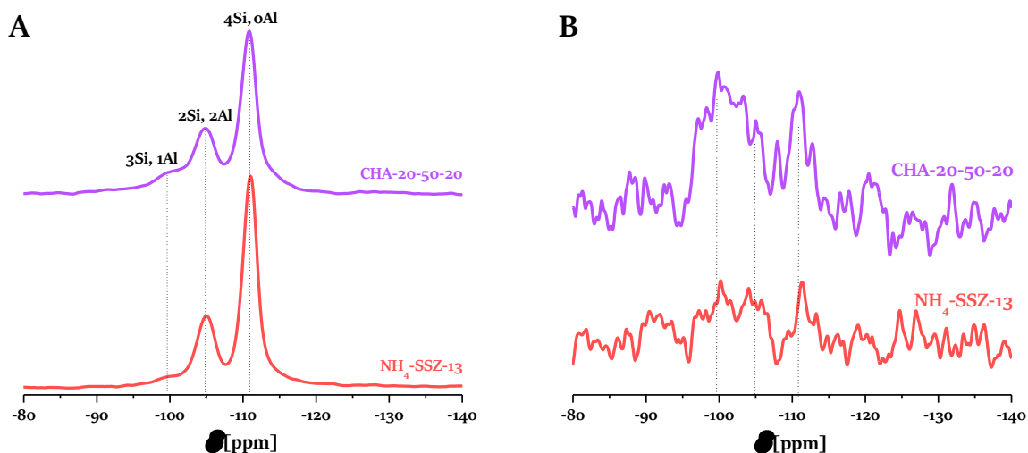
Figure 5.8. ^{29}\text{Si} MAS NMR spectra (A) and ^{29}\text{Si}\{^1\text{H}\} cross-polarization spectra (B) of \text{NH}_4\text{-SSZ-13} and one derivative, \text{CHA-20-50-20} .
