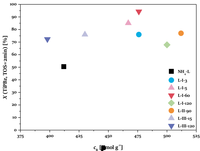
Figure 4.12. TiPBz initial conversion ( X ) as a function of Brønsted acid sites ( c_B ) concentration over hierarchical catalysts and the parent sample ( \text{NH}_4\text{-L} ) after 2 min TOS.
