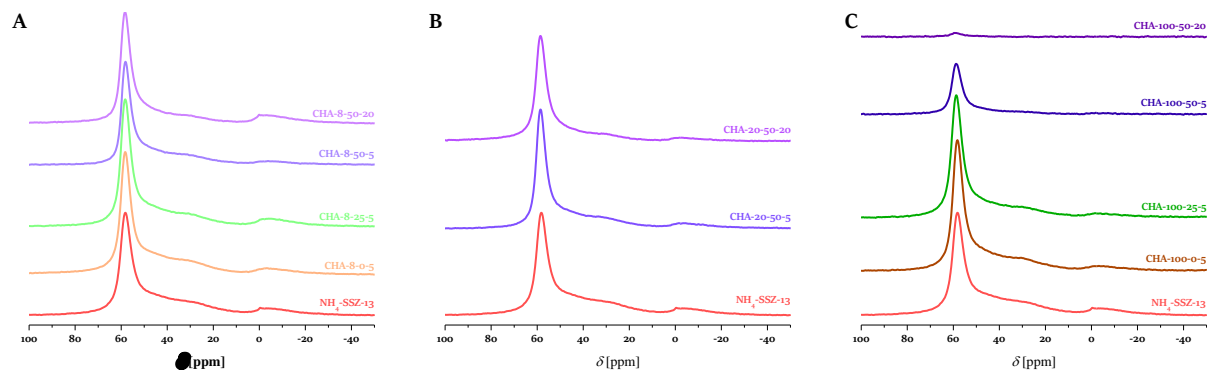
Figure 5.7. 27 Al MAS NMR spectra of the non-calcined samples from (A) series I, (B) series II, and (C) series III.
