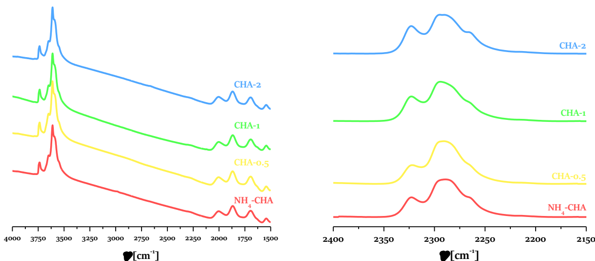
Figure 6.12. The room temperature IR spectra of the hydroxyl groups in activated parent CHA and etched derivatives (left). IR spectra of acid sites perturbed by interaction with d_3 -acetonitrile after RT diffusion (right).
