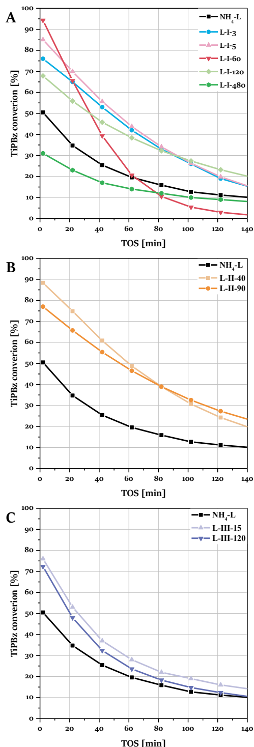
Figure 4.11. Conversion of 1,3,5-triisopropylbenzene (TiPBz) for the parent and some etched derivatives: 20 wt/% NH 4 F (A), 40 wt/% NH 4 F (B), 1 wt/% NH 4 HF 2 (C) solutions.
