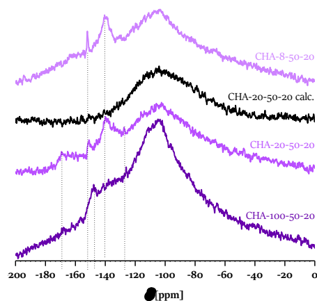
Figure 5.9. ^{19}\text{F} MAS NMR spectra of samples \text{CHA-100-50-20} , \text{CHA-20-50-20} , \text{CHA-20-50-20} calcined, and \text{CHA-8-50-20} .
