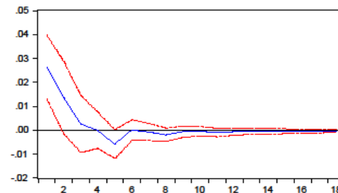
Response of D(LOG_FRENCH_IMPORTS) to MONEY_MARKET_RATE
