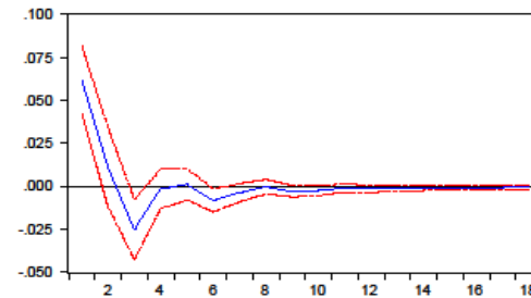
Response of DLOG(PORTFOLIO_TOT) to MONEY_MARKET_RATE
