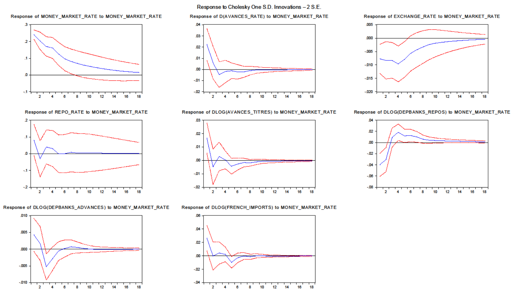
Figure 24 - Responses to a shock in the money market rate (monthly data, period October 1891 – July 1904). The impulse-response functions are based on OLS-VAR results where variables are in the following order: 1) Money market rate 2) First difference of the BoF's advances rate 3) Exchange rate with London 4) Repo rate 5) First difference of the logarithm of BoF's advances portfolio 6) First difference of the logarithm of the sum of commercial banks' repos portfolios 7) First difference of the logarithm of the sum of commercial banks' advances portfolios 8) First difference in logarithm of imports.
