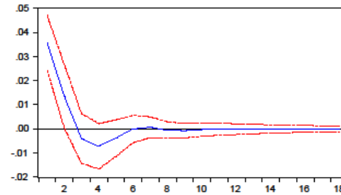
Response of D(BANQUE_RATE) to MONEY_MARKET_RATE
