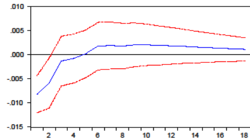
Response of EXCHANGE_RATE to MONEY_MARKET_RATE
