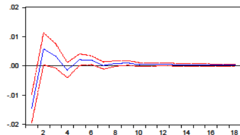
Response of DLOG(DEPBANKS_PORTFOLIO) to MONEY_MARKET_RATE
