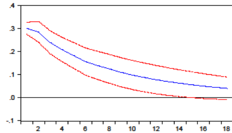
Response of MONEY_MARKET_RATE to MONEY_MARKET_RATE
