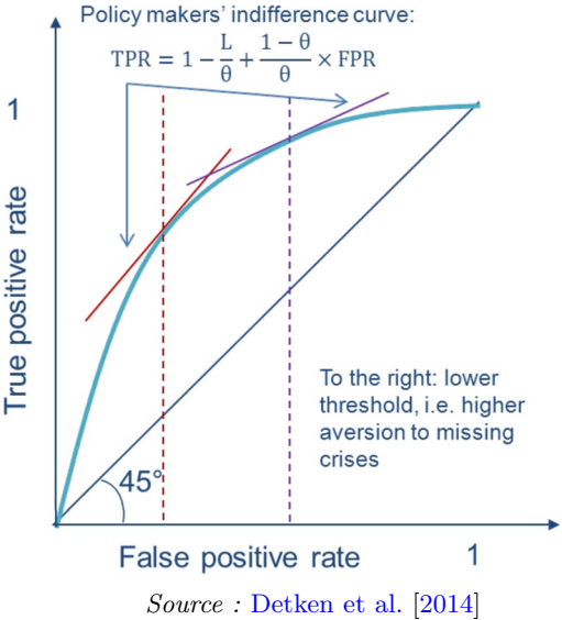
FIGURE 2.4 – AUROC methodology
