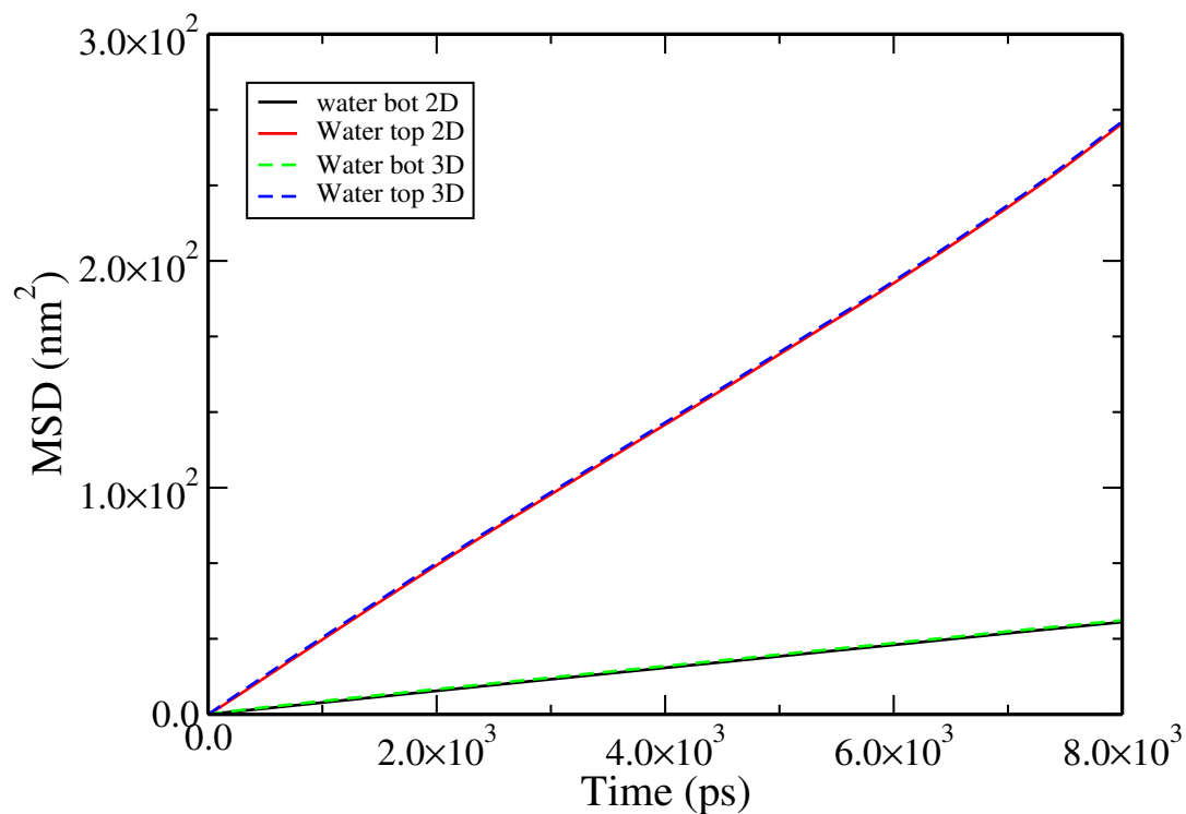
FIGURE 4.6 – Comparison of the 2D and 3D water MSD in a supported DSPC bilayer.
