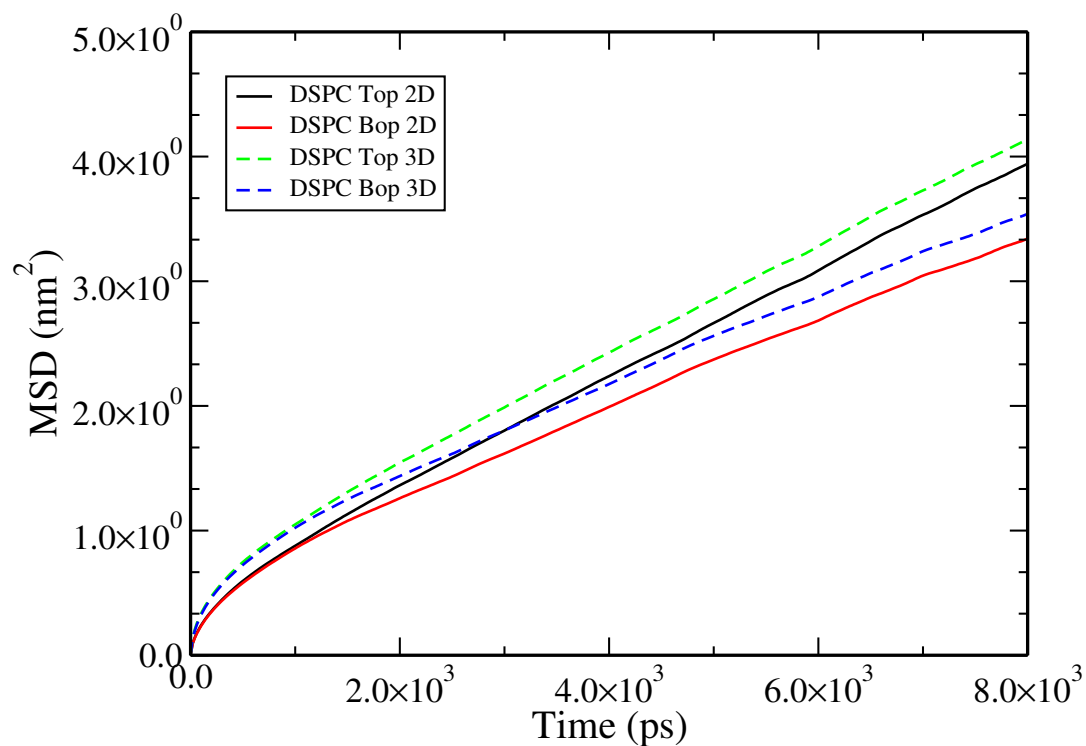
FIGURE 4.5 – Comparison of the 2D and 3D lipid MSD in a supported DSPC bilayer.
