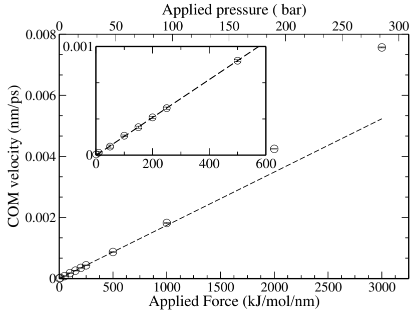
FIGURE 3.7 – Averaged drift velocities vs applied forces (lower horizontal scale bar) or stresses (higher horizontal scale bar). A shear thinning deviation is seen at \tau > 100 bars. Inset: focus on the linear regime region.
