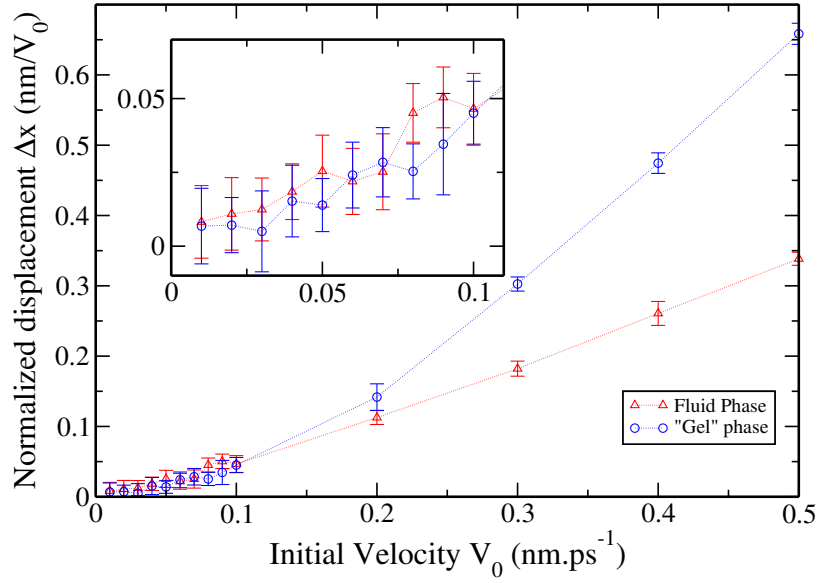
FIGURE 3.13 – Normalized averaged displacements \langle \mathcal{X}_u \rangle(t)/V_0 for a set of increasing impulses 0.01 and 0.03, ..., 0.1 and sample size 1 \leq \alpha < 200 .
