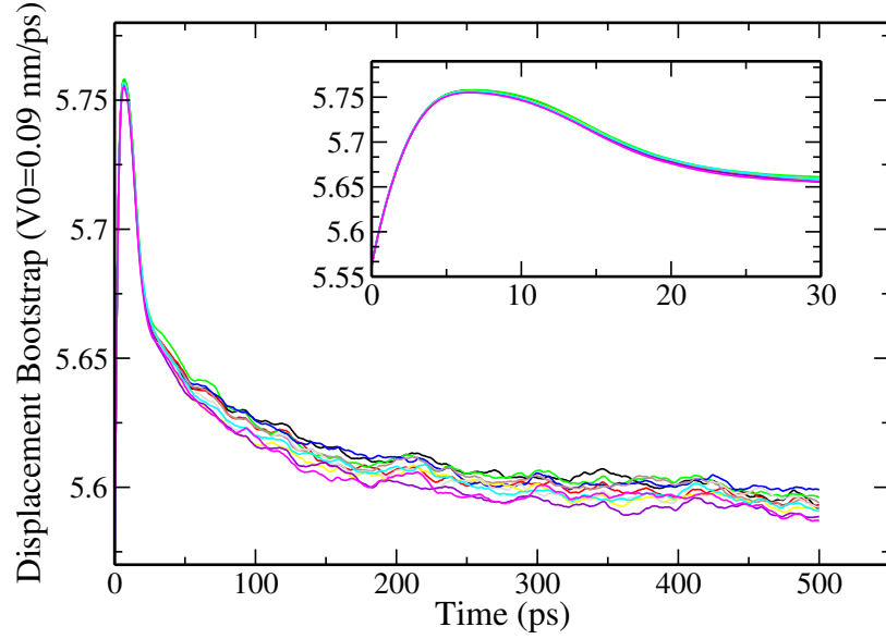
FIGURE 3.11 – Ten different bootstrap realizations of the displacement \langle \mathcal{X}_u \rangle(t) for an initial kick impulse V_0 = 0.09 \text{ nm.ps}^{-1} in the gel phase (upper leaflet). Inset: close-up look at the first peak.
