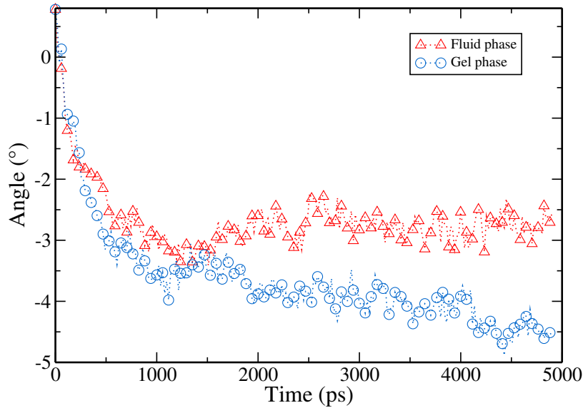
FIGURE 3.20 – Evolution of the average tilt angle \langle\theta\rangle during a constant pull force experiment with a force F = 250 \text{ kJ.mol}^{-1}.\text{nm}^{-1} (stress \tau = 24 bars).
