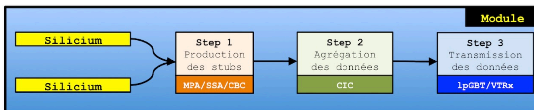
Figure 3.1: Readout: basic principle
