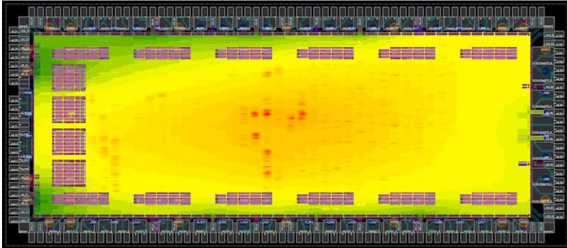
Figure 4.13: CIC2 IR drop analysis. Scale of the largest IR drop (in red) is 10mV.
