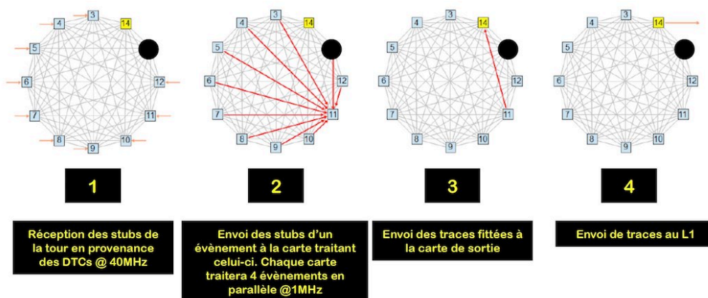
Figure 5.3: Data distribution, time multiplexing
