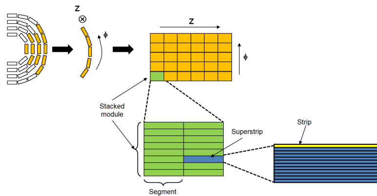
Figure 6.4: Geometric definition of a superstrip.
