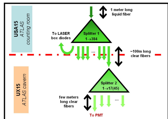
Figure 1.13: LASER system light distribution scheme
