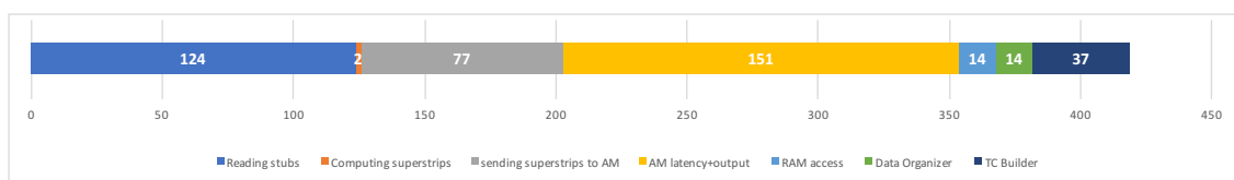
Figure 7.14: Average clock cycles spent in the various steps of the firmware for PU140 t\bar{t} events
