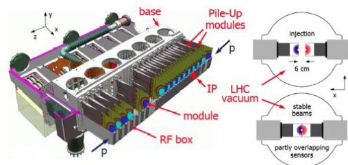
Figure 1.4: VELO working principle
