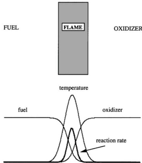
Figure 2.4: Structure of a laminar diffusion flame [32].
