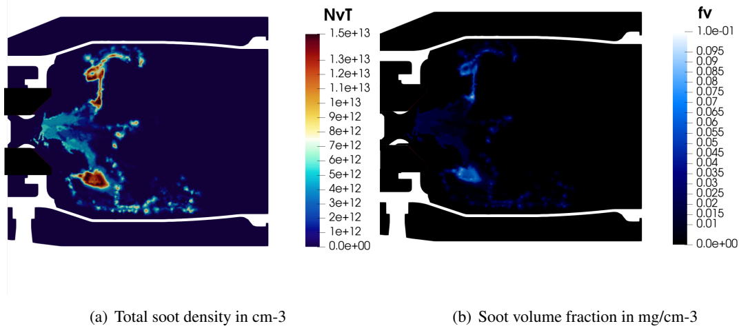
Figure 6.35: Instantaneous soot (a) density and (b) volume fraction field in the middle plane.
