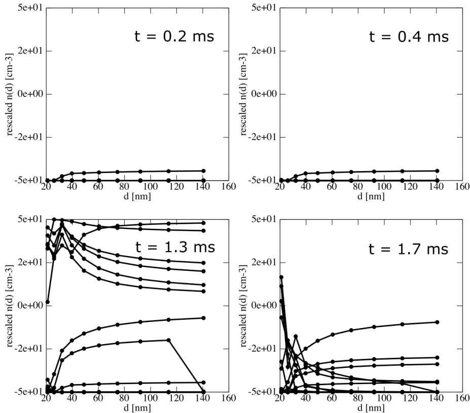
Figure 6.23: PSD database rescaled through equation 6.3 before entering the neural network, at different times.
