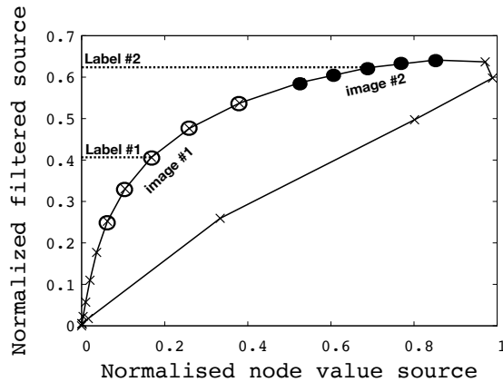
Figure 3.15: \langle \overline{\dot{\omega}^+}(c) | \tilde{c} \rangle vs \dot{\omega}^+(\tilde{c}) . Sketch of the construction of images and labels for training a CNN. Filter size: 0.3 mm.
