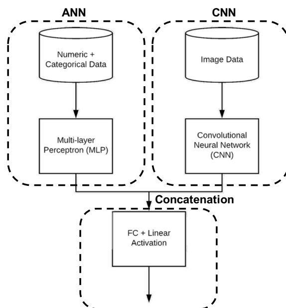
Figure 6.1: Example of a functional API used here with two sub-models.
