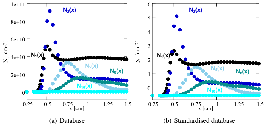
Figure 6.5: Standardisation of the database before entering the CNN. Example with a PSD discretised into M = 10 sections, among which 5 are presented. PSD mean diameters d_1 = 0.87 \text{ nm} , d_3 = 2.02 \text{ nm} , d_5 = 4.66 \text{ nm} , d_6 = 7.08 \text{ nm} , d_{10} = 37.63 \text{ nm} .
