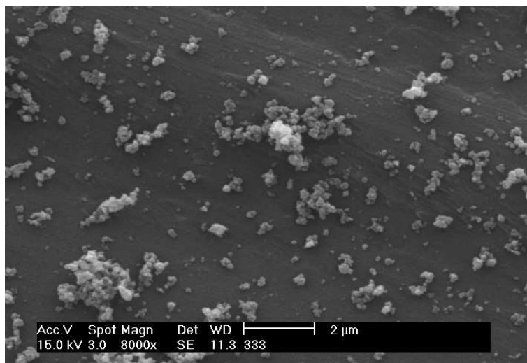
Figure 5.5: Soot formed by wood chip pyrolysis observed under a microscope [183].
