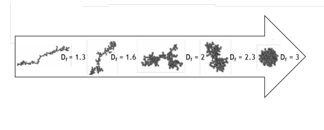
Figure 5.7: Different soot morphologies linked to their fractal dimension [187].
