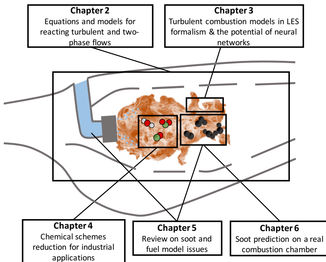
Figure 1.14: Manuscript content
