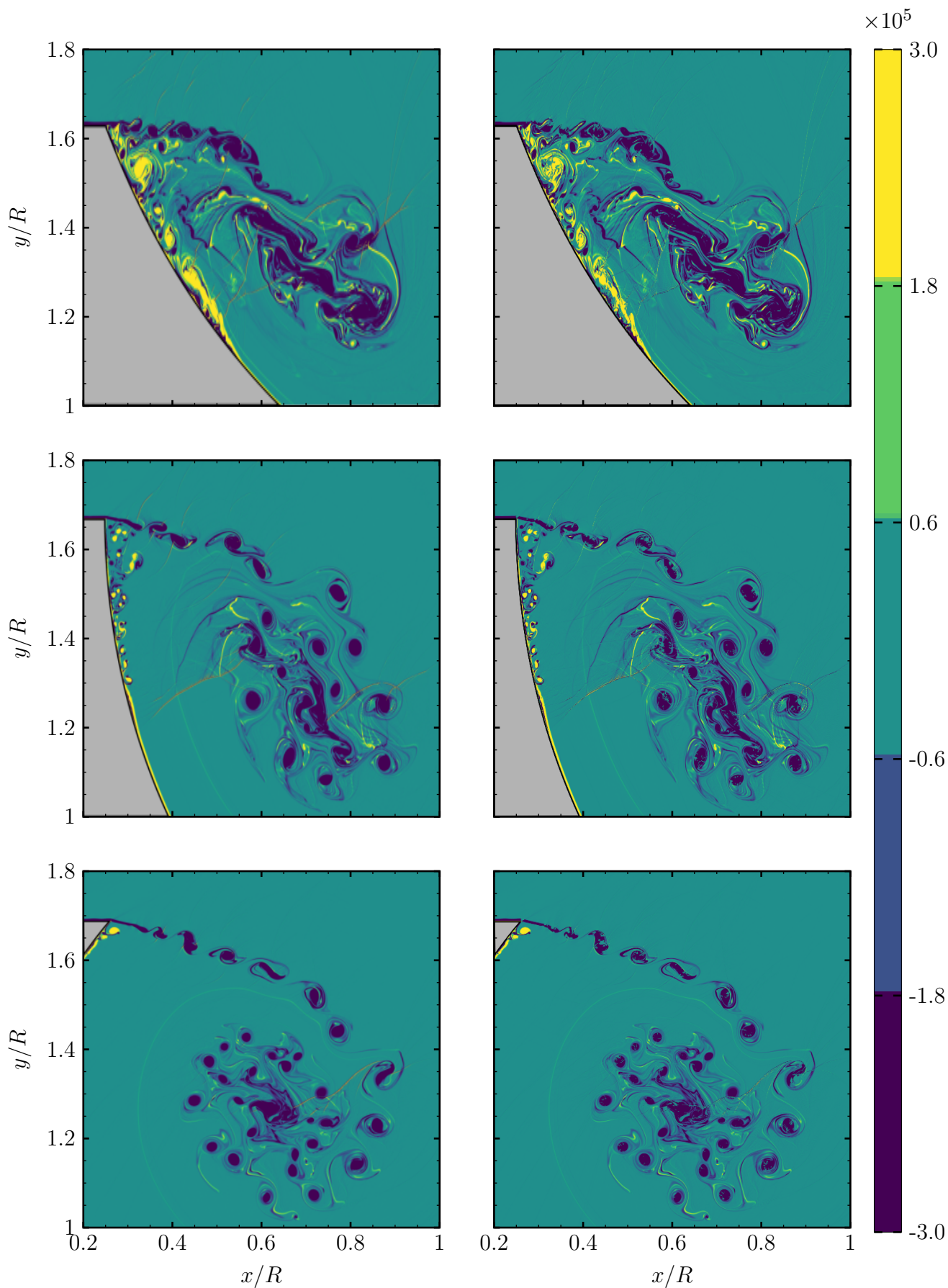
Figure C.7: Vorticity contours at t = 228 \mu s . Column-wise (left-to-right): Ducros sensor deactivated and Ducros sensor activated. Row-wise (top-to-bottom): \theta_w = 60^\circ , \theta_w = 90^\circ , \theta_w = 140^\circ
