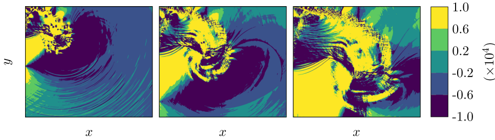
FIG. 17. TKE budget—advection term. Column-wise (left-to-right): t = 339.75, 537.75, \text{ and } 757.75 \mu\text{s} .
