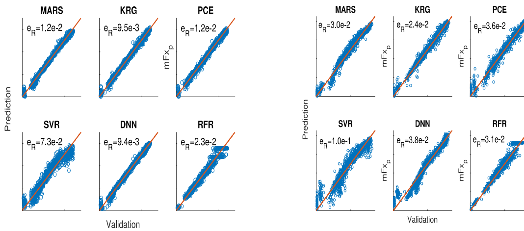
Figure 3.11: Comparison of surrogate prediction of load responses
