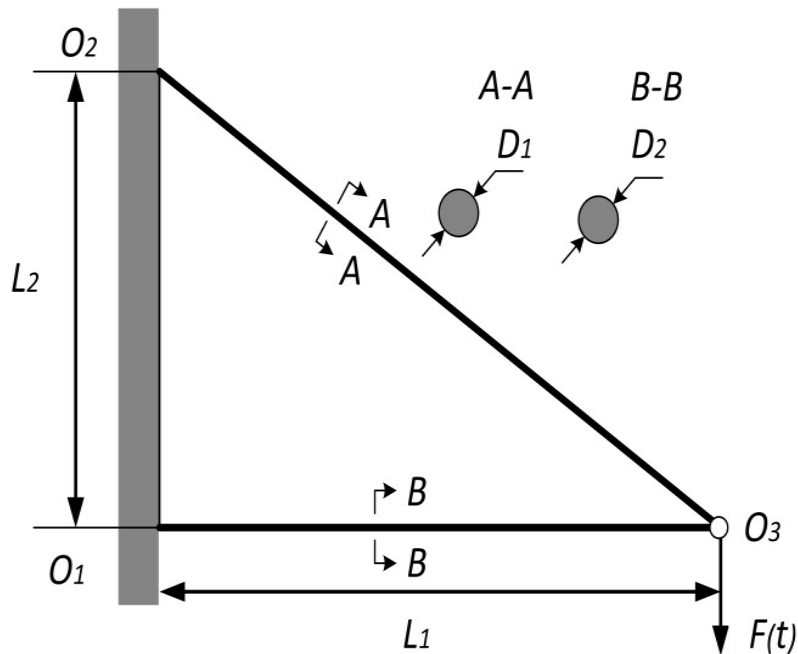
Figure 5.2: A two-bar frame structure
