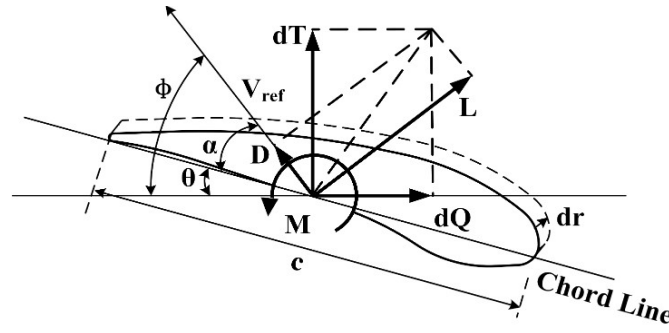
Figure A.3: Blade element geometry
