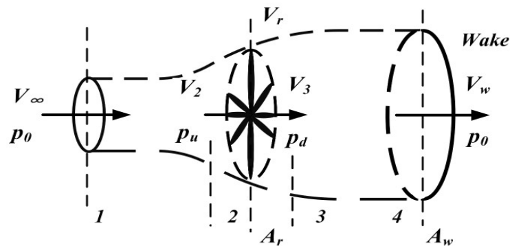
Figure A.1: Idealized flow through a wind turbine modeled by an actuator disc
