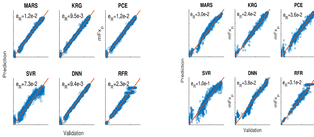
(a) Surrogate prediction for mean Fx
