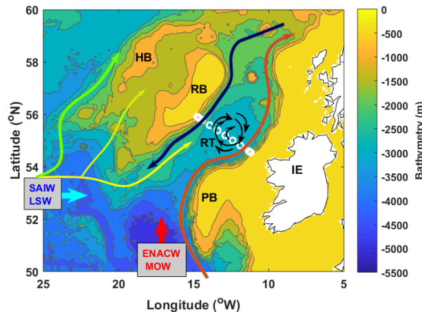
128 129 Fig. 1 Study area bathymetry map (500 m level step) with survey transect line stations (white circles) shown. 130 Subarctic Intermediate Water (SAIW) and Labrador Sea Water (LSW) subpolar waters enter the Rockall 131 Trough (RT) from the west, whereas East North Atlantic Water (ENACW) and Mediterranean Overflow 132 Water (MOW) subtropical waters flow into the channel from the south. Currents pathways in the area are 133 represented by coloured arrows, where yellow to green pathways show pathways of North Atlantic current 134 (NAC) sub-branches. Orange and dark blue arrows represent the slope current (SC) and Wyville-Thomson 135 Overflow Water (WTOW) pathways, respectively. The black curved arrows, turning clockwise, locate the 136 surface expression of the central RT at depth. Currents pathways after Holliday et al. [2015], surface imprint 137 of the deep central RT anticyclone annotated after tentative schematics in Ellett et al. [1986]. Bathymetry 138 data courtesy of USA National Geophysical Data Centre (NGDC), freely obtainable at: 139 http://www.ngdc.noaa.gov/mgg/global/relief/ETOPO2/ETOPO2v2-2006/ETOPO2v2g/ .
