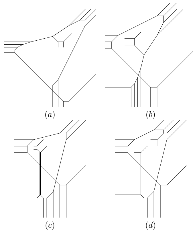
Figure 5.9 – Different examples of sextics with a loop : in (a) and (b) the degree of the remaining curve is not a standard triangle, in (c) it is a degree 2 curve, in (d) it is two lines.
