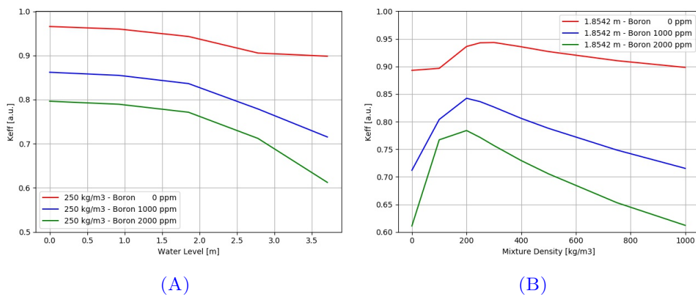
FIGURE 5.35 – Multiplication factor k_{eff} as a function of the water level (A) with a fixed water-air mixture density of 250 kg/m 3 and (B) liquid water level was set to 1.8542 m. The FAs have a burn-up 12 MWd/kg. The following boron concentrations were used: 0, 1000 and 2000 ppm.
