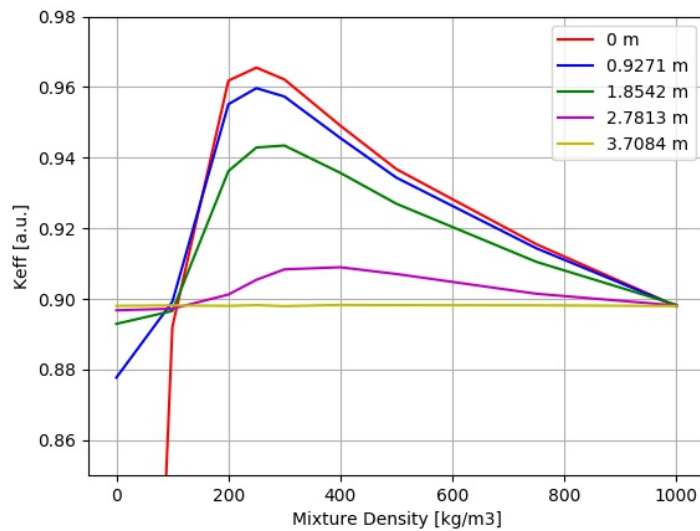
FIGURE 5.32 – Multiplication Factor k_{eff} as a function of the mixture density in the rack-pool system. The water level varies from 0-3.7084 m. The FAs have a fuel burn-up of 12 MWd/kgU^{-1} . Boron concentration was set to zero.
