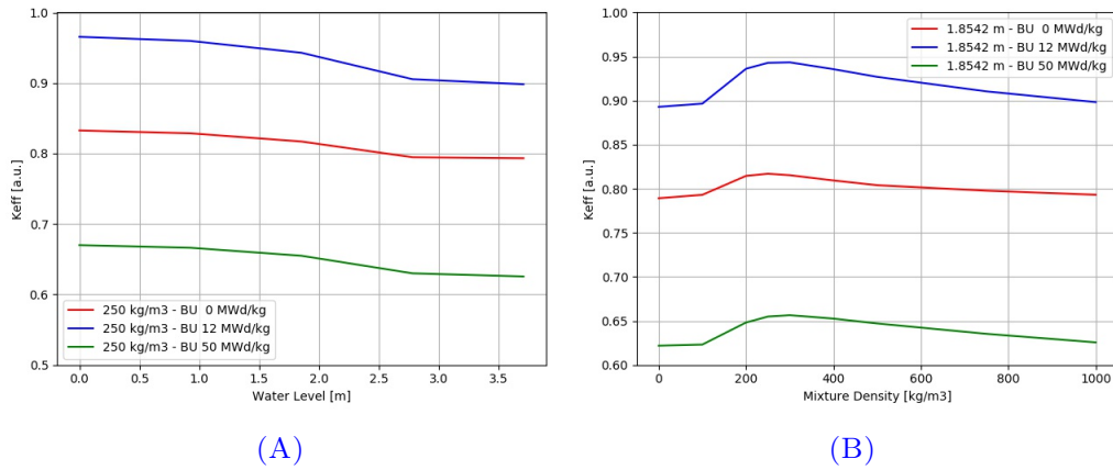
FIGURE 5.33 – Multiplication factor k_{eff} as a function of the water level (A) with a fixed water-air mixture density value of 250 kg/m 3 and (B) water level set to 1.8542 m. The FAs have a burn-up of 0, 12 and 50 MWd/kg respectively. Boron concentration was set to zero.
