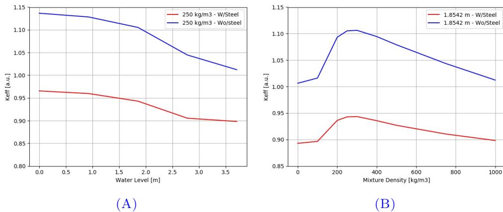
FIGURE 5.34 – Multiplication factor k_{eff} as a function of the water level (A) with a fixed water-air mixture density of 250 kg/m 3 and (B) liquid water level set to 1.8542 m with and without the SS304 rack. Boron concentration was set to zero.
