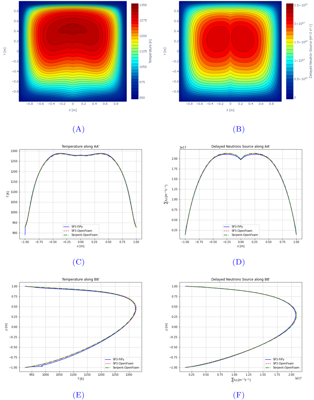
FIGURE 5.21 – Step 1.3: Temperature (A) inside the cavity, (C) along AA' and (E) along BB'. Delayed neutron source (B) inside the cavity, (D) along AA' and (F) along BB' for SP_3 (in FiPy and OpenFOAM) and Serpent-OpenFOAM internal coupling models.
