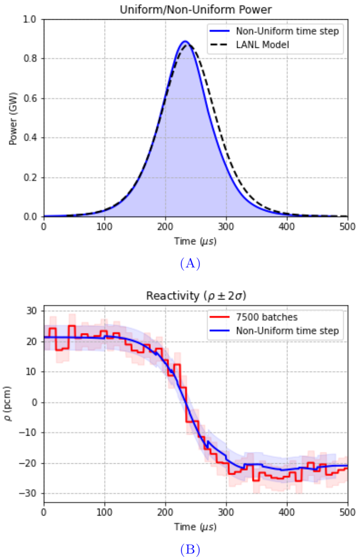
FIGURE 5.6 – (A) Power and (B) reactivity distribution with uniform and non-uniform time stepping.
