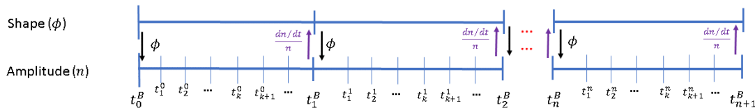
FIGURE B.1 – Time Step Scheme.
