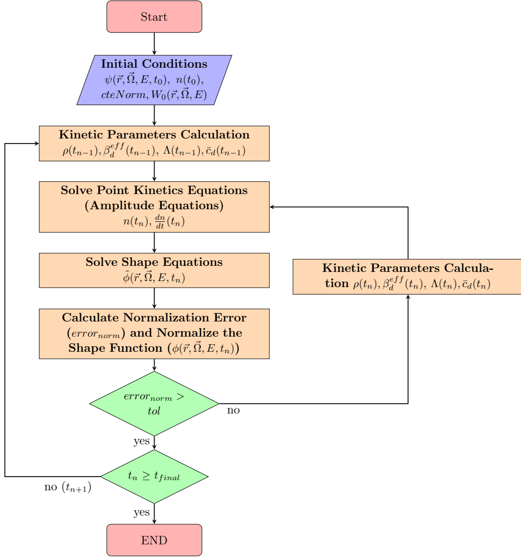
FIGURE 4.5 – Improved Quasi-Static Method scheme.
