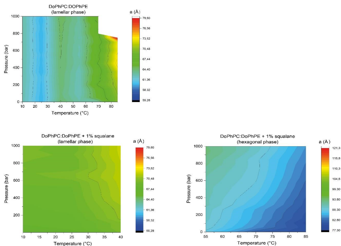
Figure S1. Lattice parameters of lipid phases are modulated by temperature and pressure. Two-dimensional pressure-temperature colour maps of lattice parameters ( d -spacing) for lamellar phases of DoPhPC:DoPhPE (9:1) (top left) and with 1 mol% squalane (bottom left) and for hexagonal phases of DoPhPC:DoPhPE (9:1) + 1 mol% squalane (right). In the absence of squalane, the membrane is highly unstructured at extreme conditions (70°C – 85°C), and it was not possible to determine its d -spacing in the most extreme conditions (85°C and 700 bar). However, in the presence of squalane, the membrane is highly structured under extreme conditions and presents non-lamellar phases, such as the hexagonal phase.
