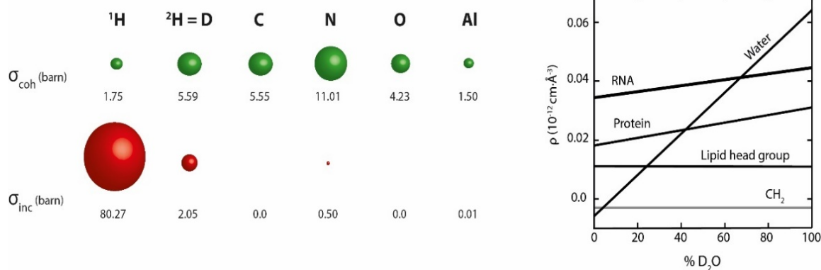
Figure 2.2. Left, neutron scattering cross sections \sigma for some elements (Sears, 1992). Right, average scattering length density of common biological macromolecules as a function of %D 2 O in the solvent. From (Harroun et al., 2006).
