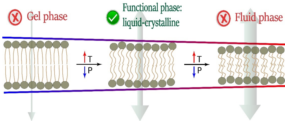
Figure 1.2. Phase transition in lipid bilayer. In functional cell membranes, lipid bilayer is found in the liquid-crystalline phase, however, variations of temperature (T) or pressure (P) may shift the membrane to non-functional phases. Grey arrows represent membrane permeability.
