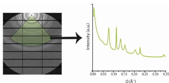
Figure 2.4. Circular average of a SAXS diffraction pattern.
