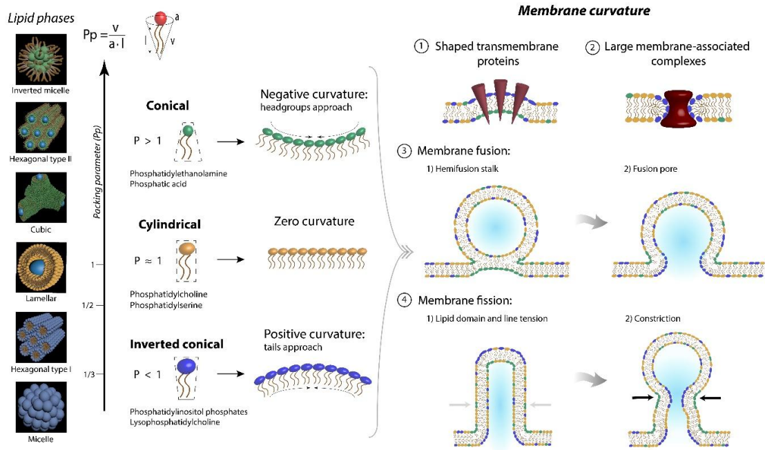
Figure S2. Sketch of different lipid phases that can be detected by SAXS and their significance for cell membranes. Membrane curvature and relationship with lipid phases detected by SAXS. Left, different lipid phases detected by SAXS and ordered by their packing parameter ( Pp = v/a \cdot l , where v is the molecular volume, l is the molecular length, and a is the molecular area at the hydrocarbon-water interface). Molecules with high packing parameter (i.e., small head groups) have a conical geometry and tend to bend to negative curvatures (green), contrary to molecules with little P , which have an inverted conical geometry and bend to positive curvatures (blue). Right, clusters of conical or inverted conical lipids indicate the different curvatures of the membrane: negative (green) and positive curvatures (blue). 1-2: Different proteins anchor to membrane that require characteristic curvatures to be functional. 3: process of membrane fusion, figures represent the two main steps where non-zero curvatures are needed. 4: process of membrane fission, this process also needs characteristic membrane curvatures.
