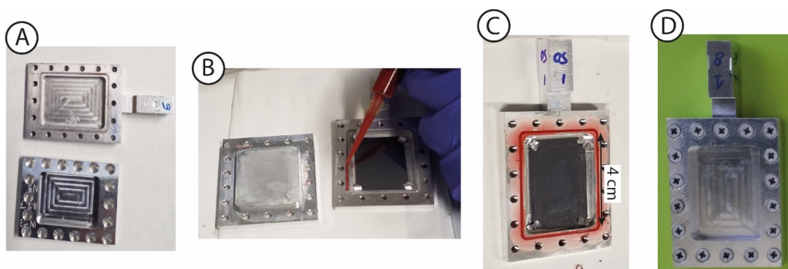
Figure 2.14. A) HT cell opened. B) Filling the joint with silicon. C) Picture of the HT cell with the wafer and four pieces of aluminium foil. D) Closed HT cell.
