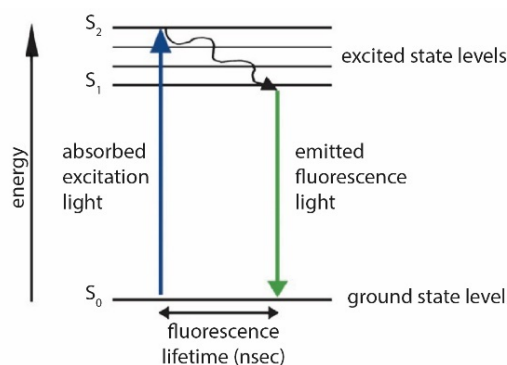
Figure 2.6. Fluorescence phenomenon represented in the Jablonski diagram (Llères et al., 2007)
