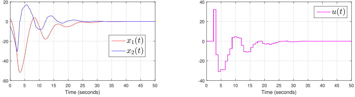
(a) State evolution of system (3.80) under control law (3.82)-(3.83).
