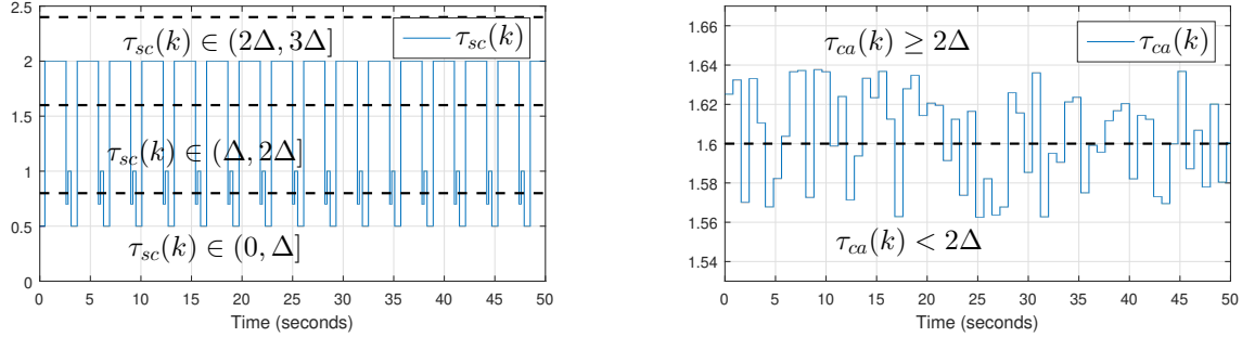
(c) Sensor-to-controller time-varying delay versus time.
