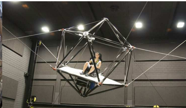
Figure 1.15: The CableRobot motion simulator with a large translation workspace, [Mie+16]
