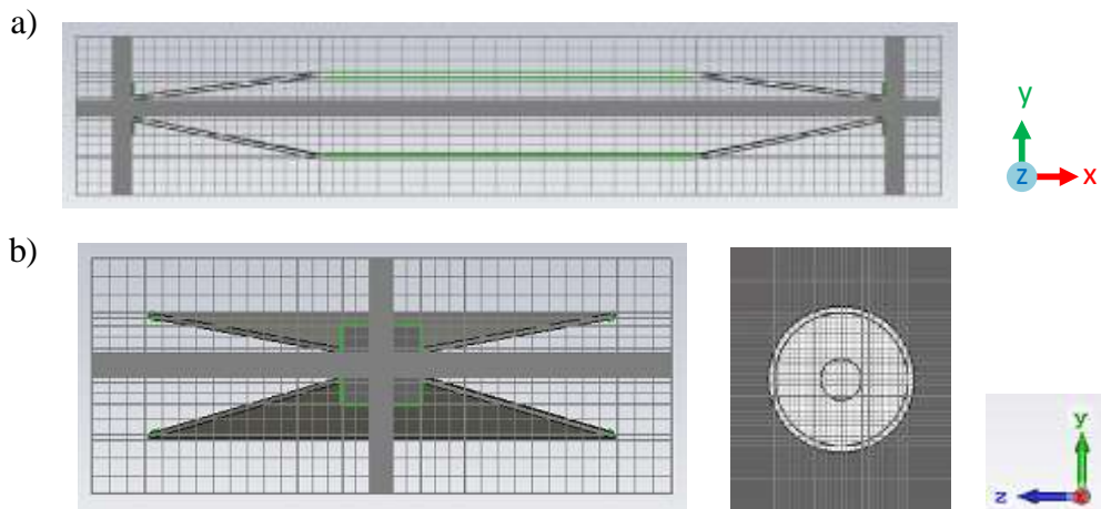
Figure 33 : Schematics of the non-uniform meshing of the TEM cell.
