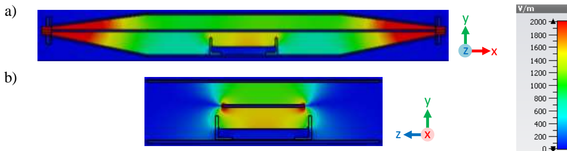
Figure 37 : E-field distribution at 1.8 GHz of the TEM cell containing Fluorodish filled with 3 mL of HBSS, a) longitudinal and b) transversal plane cuts.
