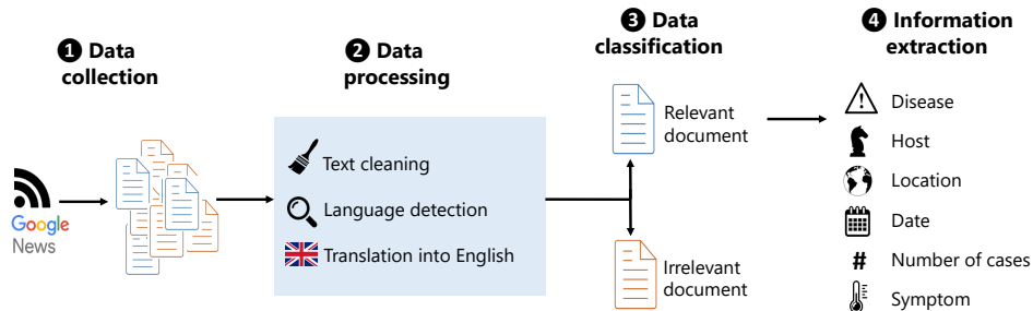
Figure 40 PADI-web pipeline.
