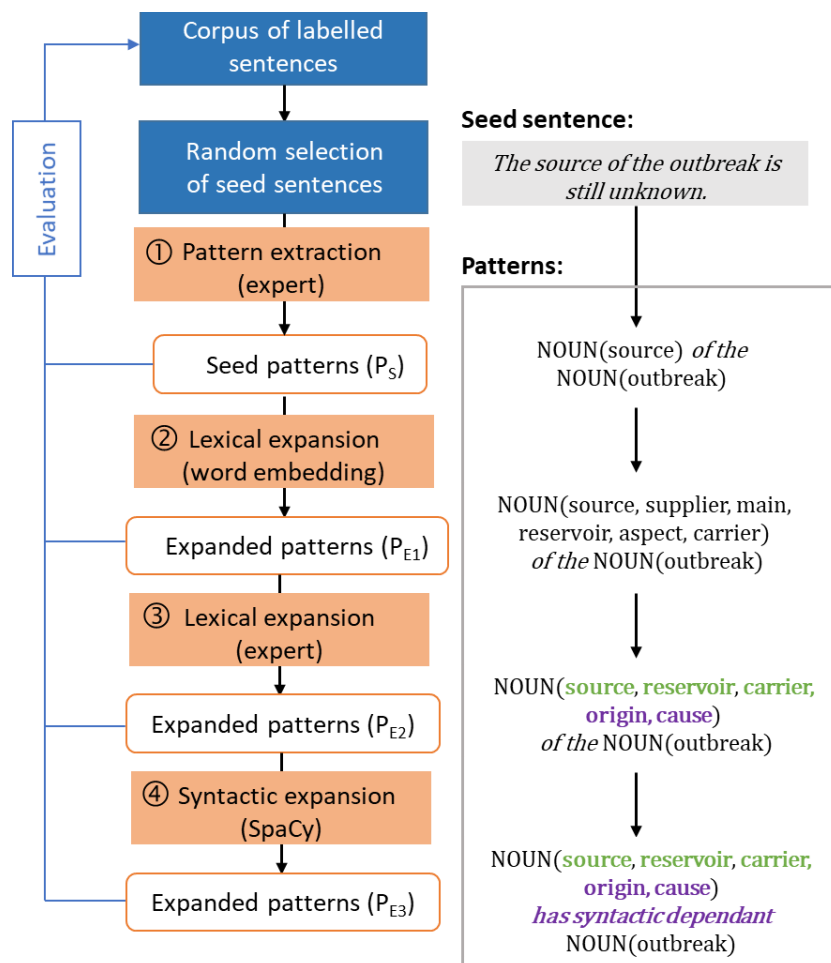
Figure 16 Incremental pattern expansion.
