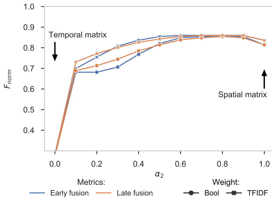
Figure 32 Comparison of fusion methods to combine disease and host features. The arrows correspond to the use of unimodal matrices.
