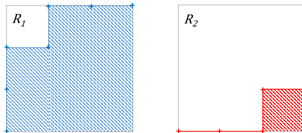
Figure 22 ROC curves obtained by two different rankings, R_1 and R_2 . The dashed areas correspond to the AUC.
