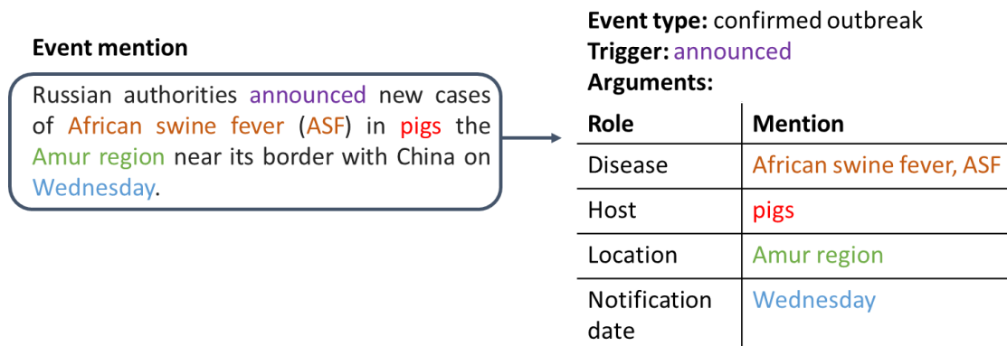
Figure 6 Illustration of the extraction results of three event extraction subtasks, i.e. event mention/trigger detection and event type identification, argument detection and argument role identification.
