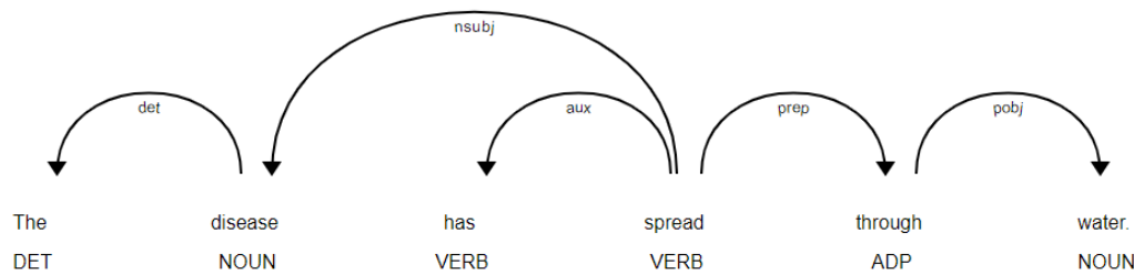
Figure 17 Dependency tree of sentence (1), generated with spaCy dependency parser.
