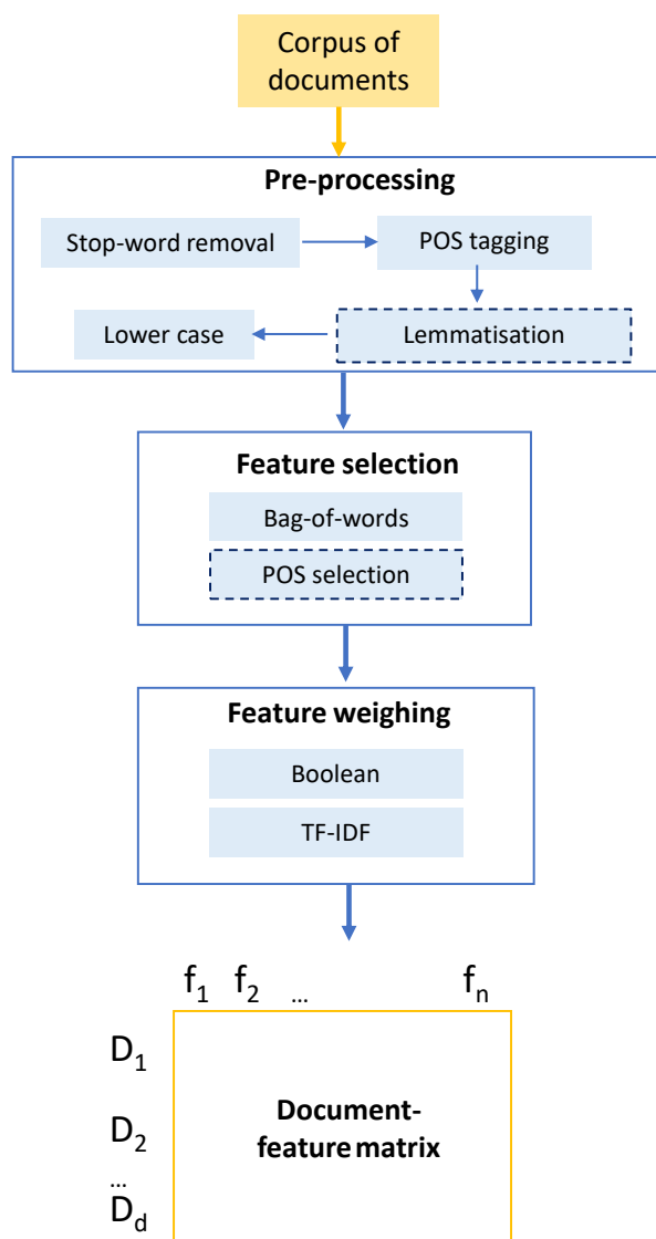
Figure 29 Steps to create the document-features matrix based on morphosyntactic features. Dashed steps corresponds to optional preprocessing steps.
