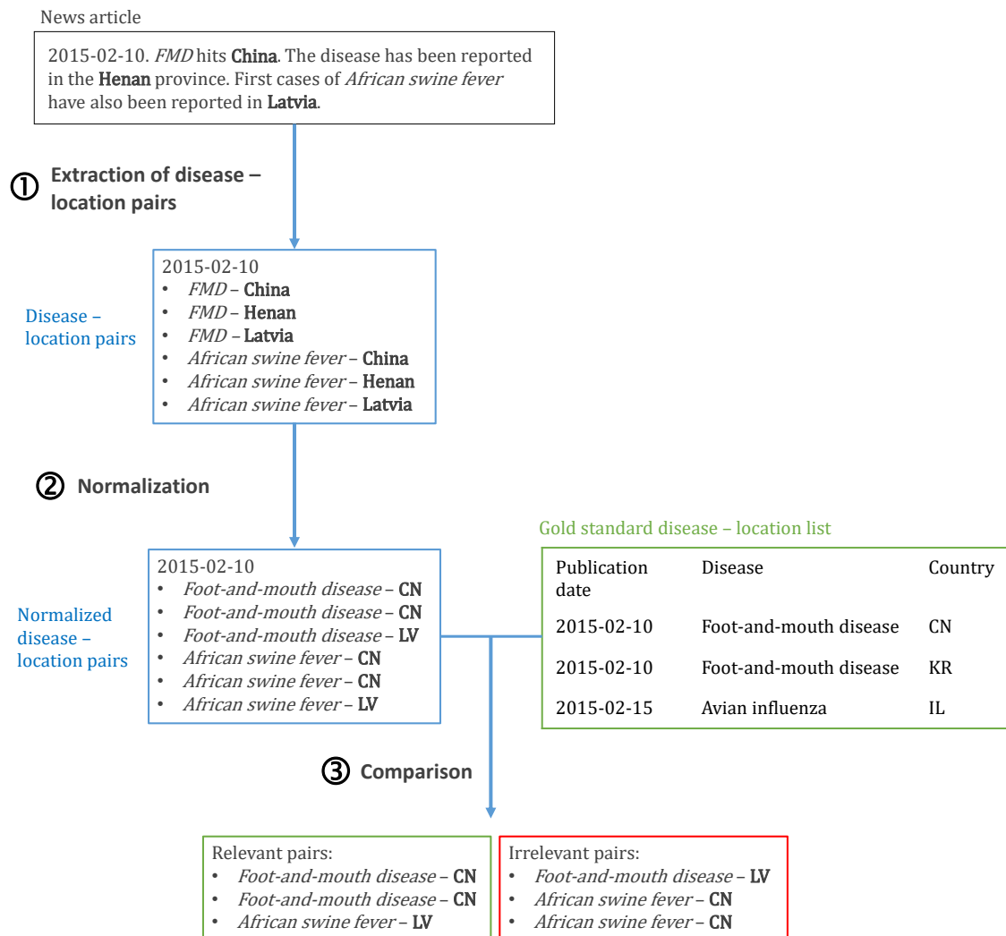
Figure 21 Steps to evaluate the relevance of the disease-location pairs extracted from a news article.
