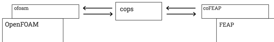
Figure 5.13: Software component architecture for code coupling (ofoam and coFEAP) with control component (cops) (Kassiotis et al., 2011b)
