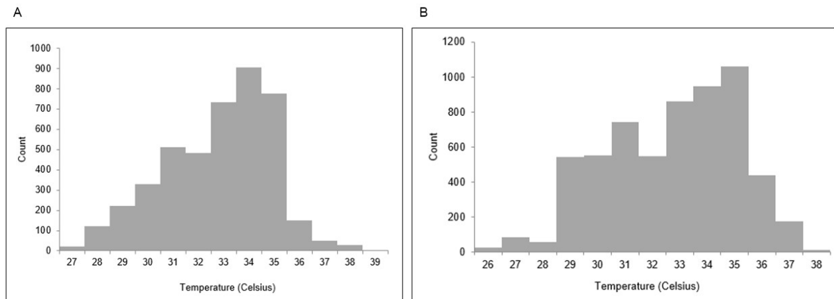
Supplementary information S7. Temperature histogram for 12 Carcharhinus melanopterus (A) and 14 Negaprion acutidens . Temperature data were collected during manual tracking in a one-minute interval.
