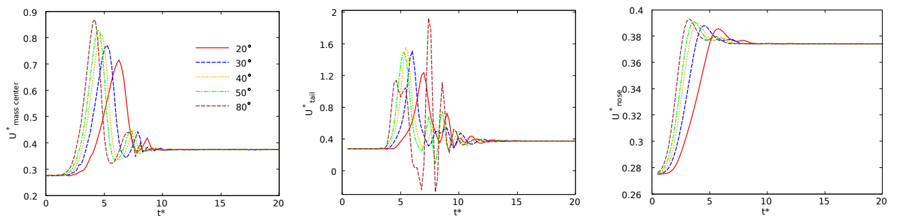
FIGURE 5.20: Evolution of the dimensionless bubble velocity as a function of dimensionless time for different parabolic concave expansions.
