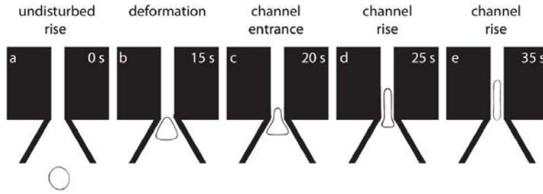
FIGURE 2.16: Video recording experiment to describe bubble rise and deformation through an inverted shallow flaring geometry (from Qin et al. (2018) ).
