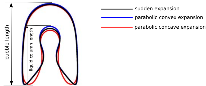
FIGURE 5.25: The liquid column length for different types of expansions.
