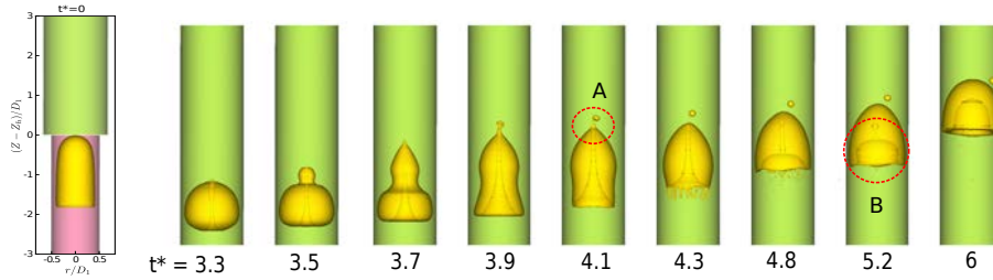
FIGURE 4.39: Penetration of Taylor bubble rising through large expansion ratio ( G - W : 70\% , Mo = 1.96 \times 10^{-4} , Eo = 46.7 , \epsilon = 1.73 ).
