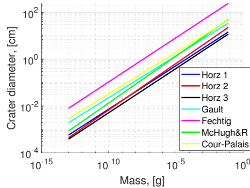
Figure 3.4: Calculated DCD with models listed above for micrometeoroids of mass 10^{-13} - 10^{-2} g, impact velocity of 20 km/s and micrometeoroid density 2.5 \text{ g/cm}^3 .
