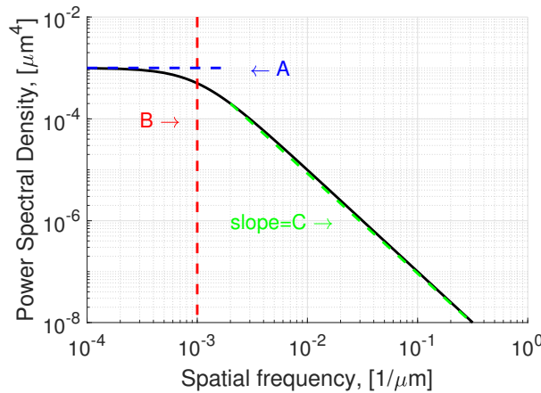
Figure 2.5: The PSD in K-correlation model: A = 1e - 3 \mu m^4 , B = 1e + 3 1/\mu m , C = 2 .
