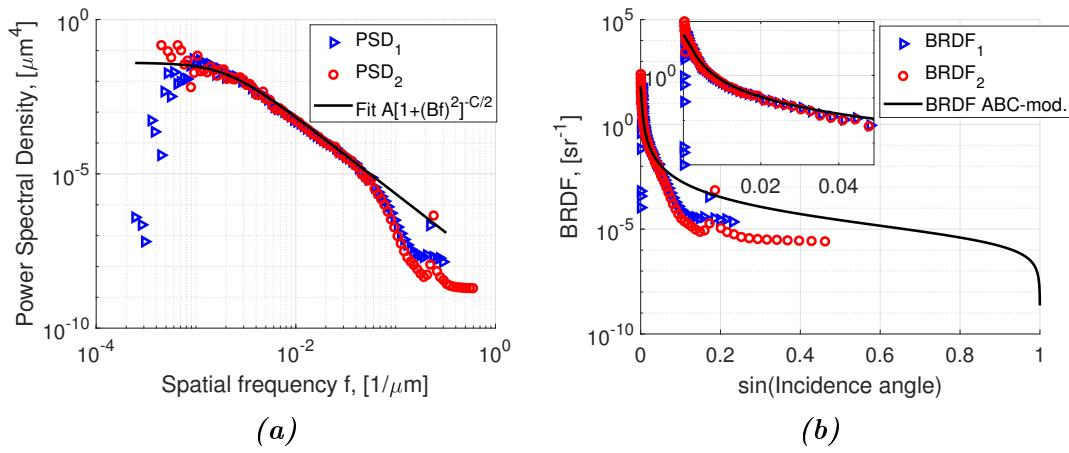
Figure B.1: The computed PSD (a) and corresponding BRDFs (b) for maps (b,c) given in Fig. 5.18 ( PSD_2 and PSD_1 respectively). The fit coefficients are A = 4 \times 10^{-2} \mu\text{m}^4 , B = 5 \times 10^2 \mu\text{m} , C = 2.5 (same for both figures). In the box of the figure (b) is zoom of near-normal incidence part of the BRDF.
