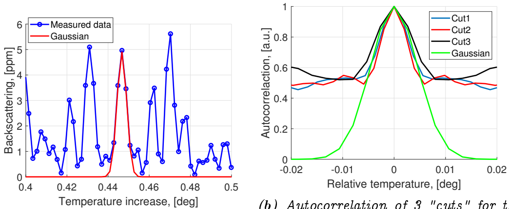
(a) Piece of the data sample (in blue) first measurements data set and Gaussian with a Gaussian of speckle size (in red). (b) Autocorrelation of 3 "cuts" for the Gaussian of appropriate speckle width (in green)
