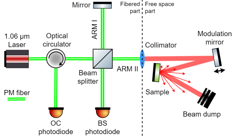
Figure 6.1: Schema of the interferometric setup for coherent backscattering measurements. Green: PM optical fibers. Red: free-space beams. Thin red arrows: scattered light from the sample.
