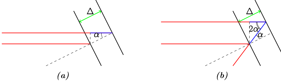
Figure 5.23: Path modulation for the case of backscattering from the mirror (a) and the beam dump (b). With PC 4 FL piezo (Thorlabs), which is used for the mirror modulation, 10 volts amplitude corresponds to \Delta = 0.2\mu\text{m} (green line).
