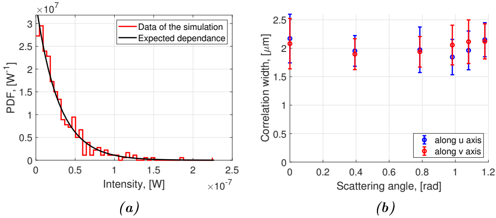
Figure 4.17: Distribution of scattering intensities near zero scattering angle given by the coherent scattering model (a) size of the autocorrelation function of the speckle in the image plane along u and v axes for different scattering angles \theta_s (b).
