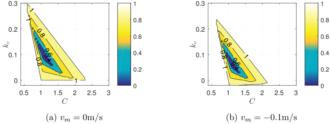
Figure 3.15 – Maximal norm of eigenvalues for different v_m as a function of C and k_v when k_S = 0, k_D = 0 .
