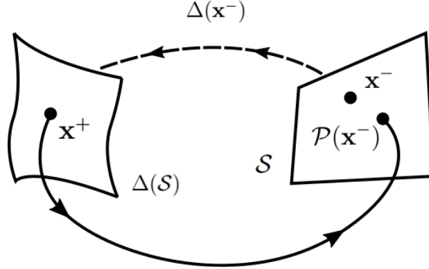
Figure 2.6 – The Poincaré return map
