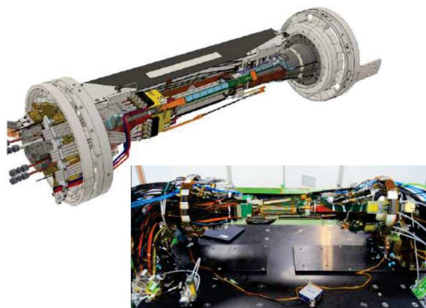
Figure 3.5: The CAD rendering and a real image of the vertex detector cartridge and BEAST II monitoring setup installed during Phase 2 at the interaction point.
