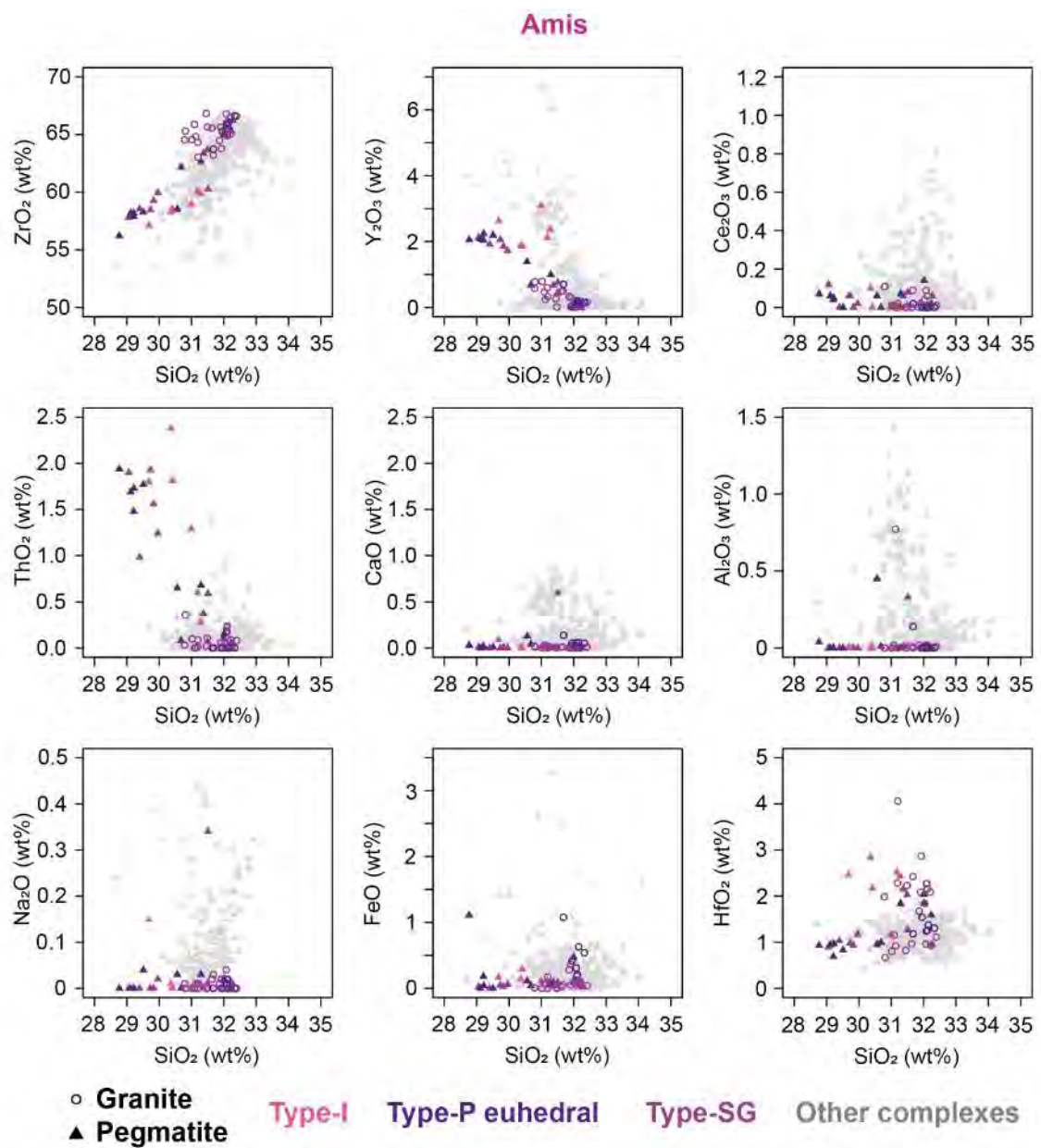
Figure 4.9 Binary diagrams highlighting the main major and trace composition of zircons from different rocks and types as a function of SiO 2 at Amis
