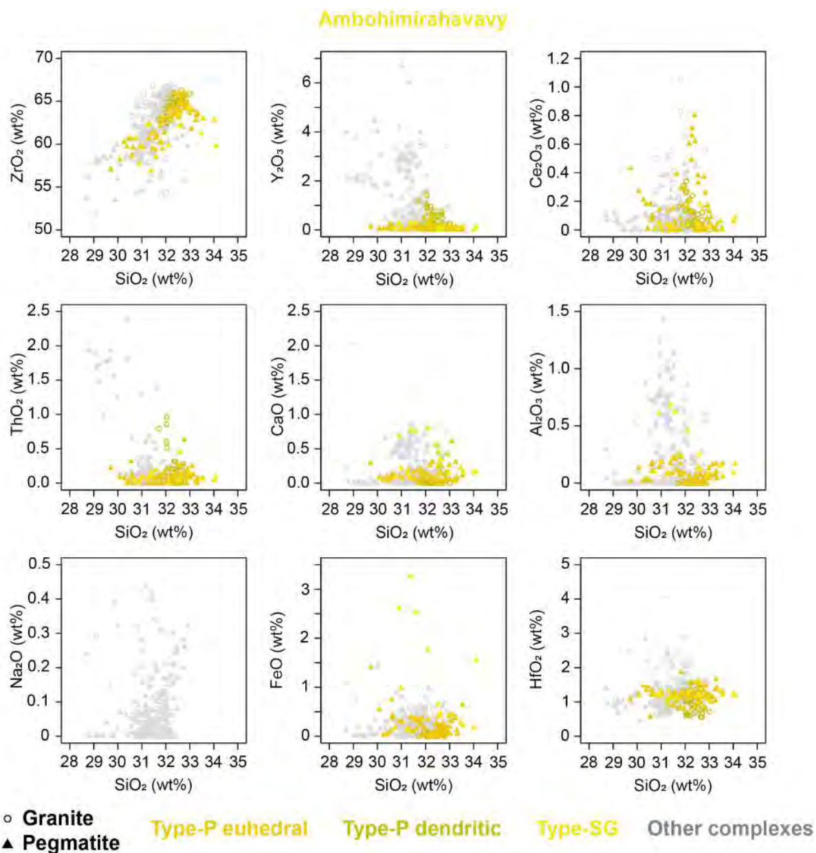
Figure 4.12 Binary diagrams highlighting the main major and trace composition of zircons from different rocks and types as a function of SiO 2 at Ambohimirahavy
