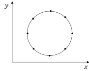
Figure 2.1: Ring of equidistant test particles.
