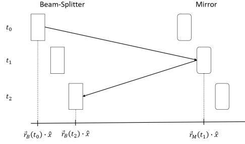
Figure 4.1: Schematic representation of the photon traveling path.
