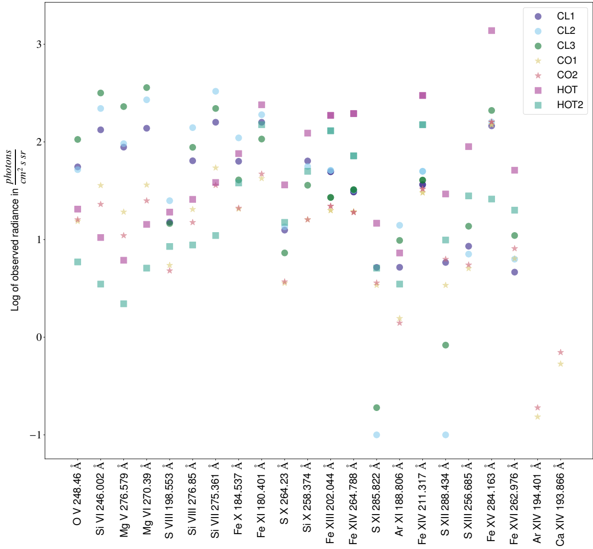
Figure 5.4.1: Logarithm of the observed radiances in photons \text{cm}^{-2} \text{s}^{-1} \text{sr}^{-1} for each spectral line listed in Table 5.2.1. The different markers and colors show the values in the different regions.
