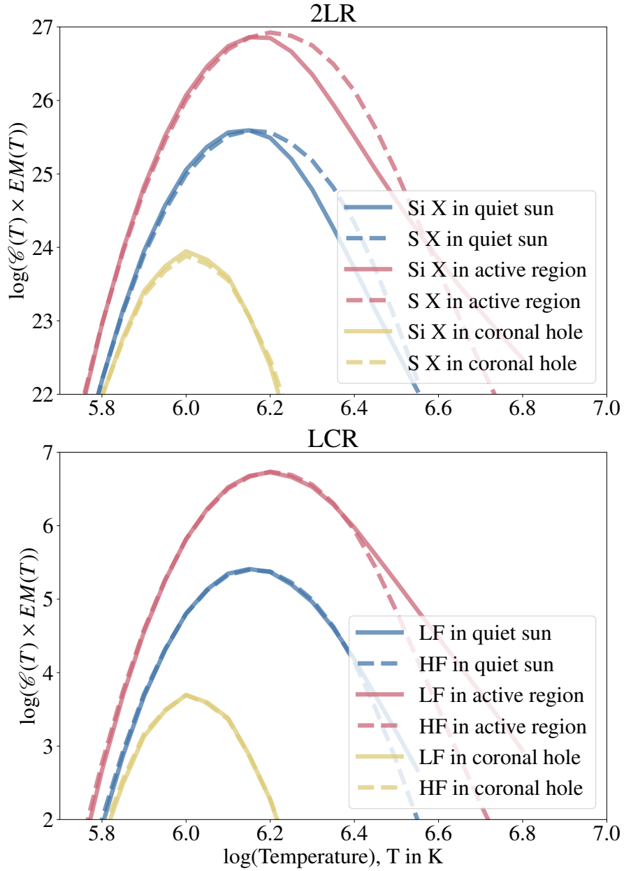
Figure 3.7: Products between the EM and the contribution functions ( \mathcal{C}_{\text{LF}} , solid lines, and \mathcal{C}_{\text{HF}} , dashed lines), as functions of the temperature for both methods, using the coefficients in Table 3.1. Different colours correspond to different EMs from CHIANTI.
