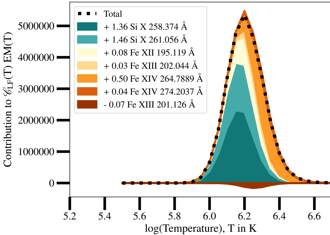
Figure 3.8: Contributions of the different spectroscopic lines to the \mathcal{E}_{LF}(T) EM(T) product as a function of temperature for the CHIANTI AR EM. The total (dotted line) corresponds to the full red line in the bottom panel of Fig. 3.7. Here, Fe and Si line contributions are shown in ocher-red and blue-green colours, respectively. We separate the positive and negative contributions to the total.
