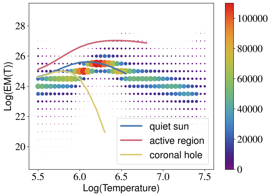
Figure 3.2: Histogram of the EM(T) values in the first region of interest (black square) of Fig. 3.1. The colour scale and the size of the points correspond to the number of pixels containing an EM of a given value at a given temperature. We have also traced in full lines the typical EMs from CHIANTI that we use to optimise the cost function (Eq. 3.11). The red line corresponds to an active region, the blue line to the quiet Sun and the yellow line to a coronal hole.
