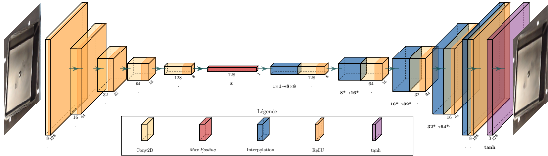
Figure 3.16 – Architecture d'un auto-encodeur.
