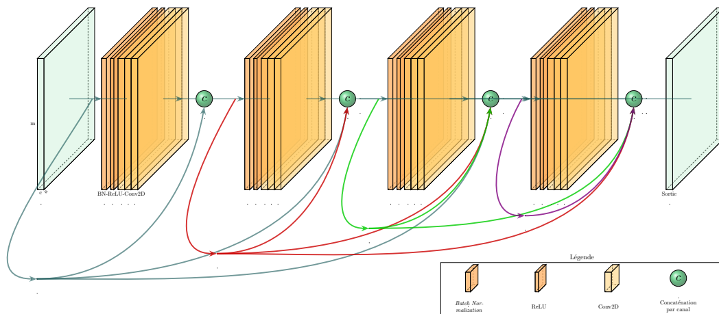
Figure F.1 – Architecture d'un bloc DenseNet.
