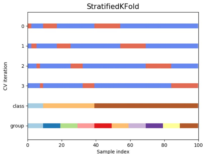
Figure E.2 – Stratified 4-Folds. Figure extraite de la doc SciKit-Learn , License BSD 3-clauses.
