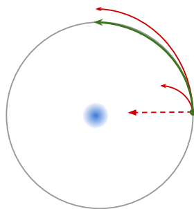
(a) Hamiltonian Monte-Carlo metaphor of gravity: for the sampler to efficiently cover all the space of interest (horizontal line at sphere height), it should not follow gravitational force towards higher probability (dotted or full red), neither drift away from it, but rather follow an orbit around it (green arrow). Each "orbit" remains at equal energy (Betancourt, 2017).
