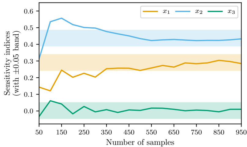
Figure 3.12 – Illustration of the convergence analysis of the sensitivity analysis of the Ishigami function: the analysis is carried out on sub-samples of growing size. If from a certain size and for all input variables the indices are stable within a \pm 0.05 band, convergence is achieved.
