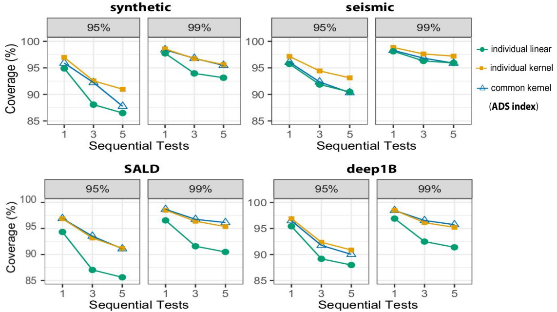
Figure 4.16.: Effect of multiple sequential tests on the coverage of 95% and 99% prediction intervals. We evaluate three (for 1, 16, and 256 visited leaves) and five sequential tests (for 1, 4, 16, 64, and 256 visited leaves).
