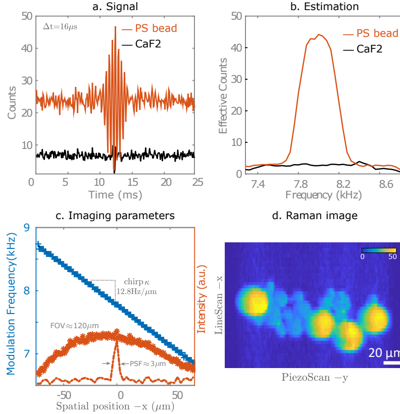
FIGURE 5.4: (a) Time trace of Raman signal of a 30 \mu\text{m} PS bead (red) and of the \text{CaF}_2 slide background (black) ( 16 \mu\text{s} sampling time). (b) Corresponding isolated sidebands of the Fourier transformed time traces (10x averaged). (c) In blue, the calibration between temporal modulation frequency and space - measured by translating an isolated 12 \mu\text{m} MR bead. In red, imaging system parameters - PSF and field of view (sample - MR beads). (d) Line scanned Raman image of a beads mixture (PS, PMMA, MR) on a \text{CaF}_2 slide with no spectral filtering.
