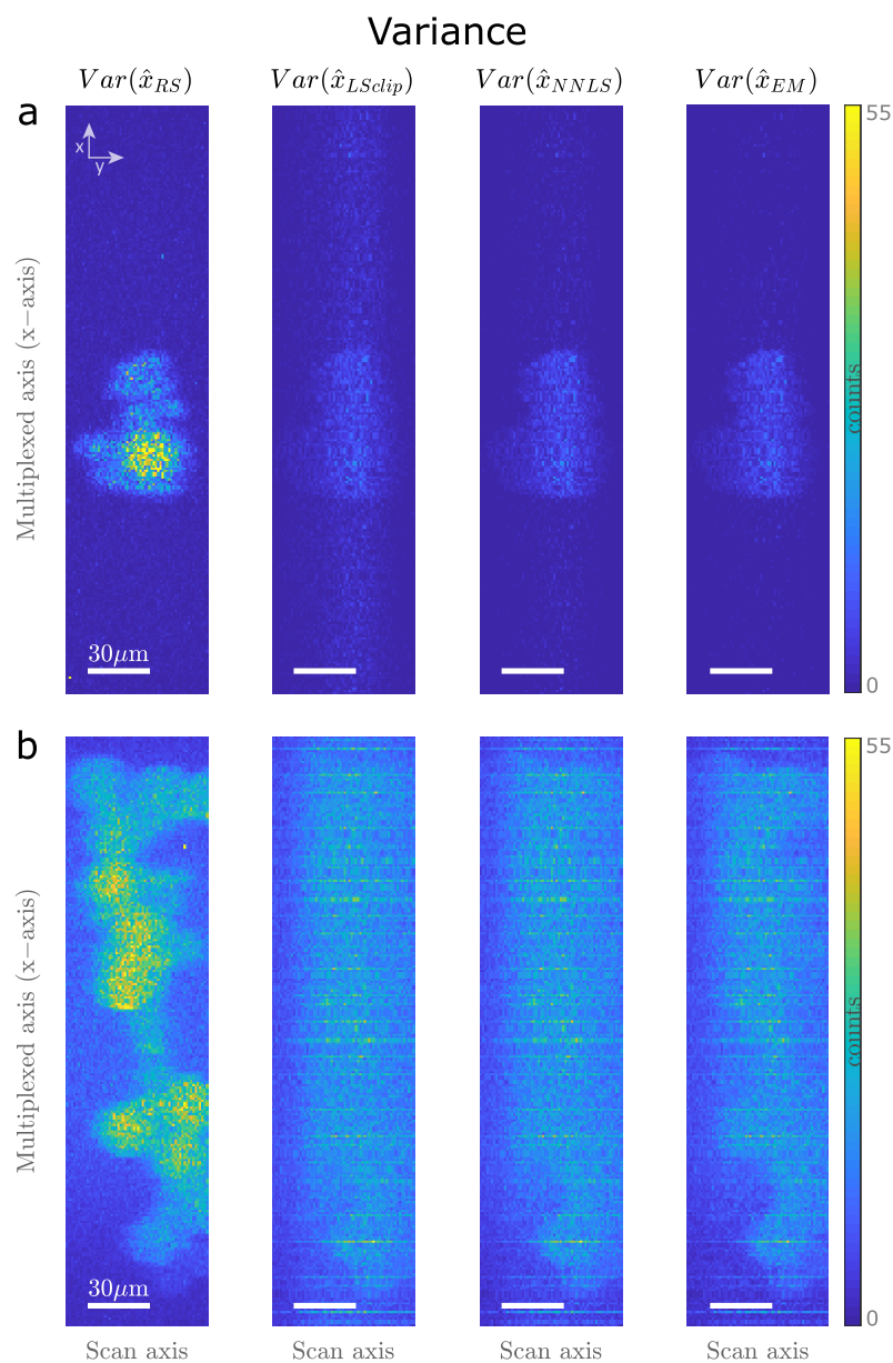
FIGURE 6.18: Estimation variances calculated from 50 measurements. Only 270 \mu\text{m} out of 511 are shown along the multiplexed axis. (Top - sparse sample): S-multiplexing decreases the variance on the beads and LS estimation spreads the noise along the multiplexing axis. The object shape is slightly retrieved with LS-clip because the zeros are removed, but we retrieve a uniform variance along each multiplexed line with pure LS estimation (not shown). Estimators with positivity constraints mitigate this effect. (Bottom - denser sample): The variance is quasi-uniform though NNLS and EM help reducing it on null pixels at the object borders.
