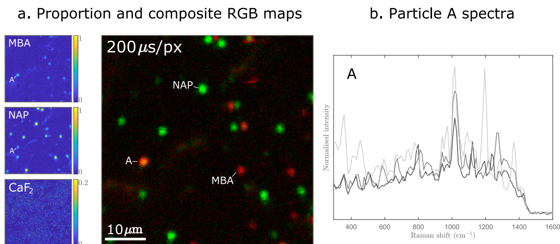
FIGURE 4.17: (a) Proportion maps and composite RGB map (form MBA and NAP proportion maps). Exposure time: 200 \mu\text{s} / pixel / filter. Most particles are clearly identified, but particle A is seen as a mixture of two species. (b) Three recorded spectra, in a row, on A show instability.
