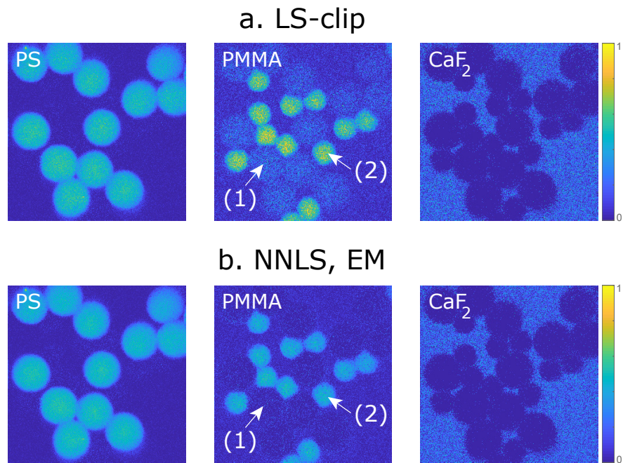
FIGURE 6.20: Estimated proportion maps of PS, PMMA and CaF 2 , obtained with CRT estimations based on (a) LS-clip and (b) NNLS. The results with LS-clip are the same as in Fig. 4.6. NNLS, that gives similar results that EM on this example, reduces the noise from residual PS estimation (1) on the PMMA map. The estimated proportion of PMMA beads (2) also seems to be slightly lower.
