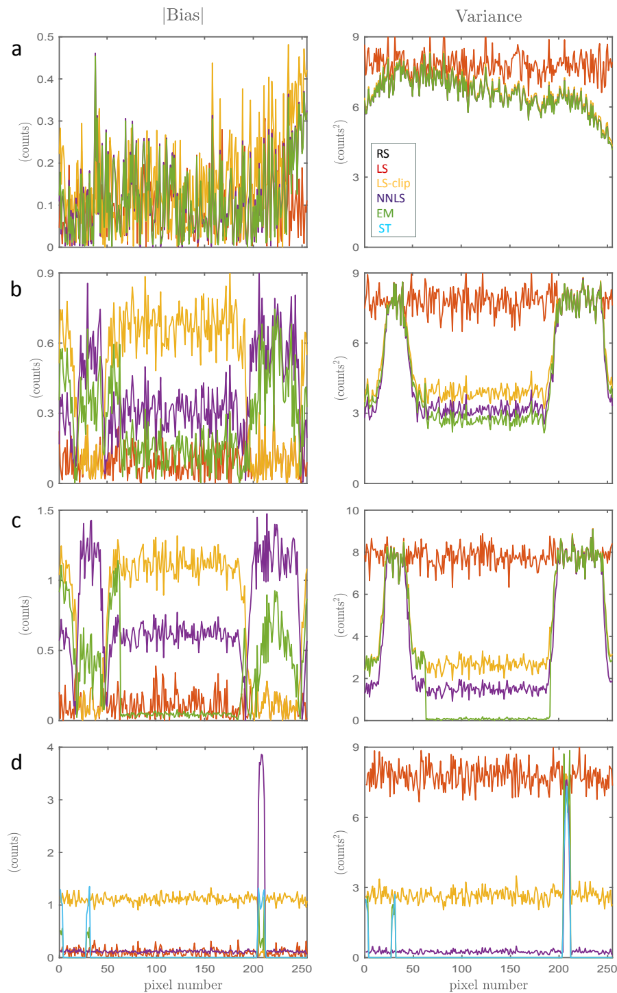
FIGURE 6.13: Effect of the estimators on the absolute bias and variance for the 4 objects (mean number counts / pixel = 4). Alternative estimators reduce the variance as compared to LS (right) but may introduce some bias. LSclip leads to a significant bias increase on the background. NNLS moderately increases the bias on the background but seems to increase it a lot on the peaks when the object is sparse (d). EM probably leads to the best compromise.
