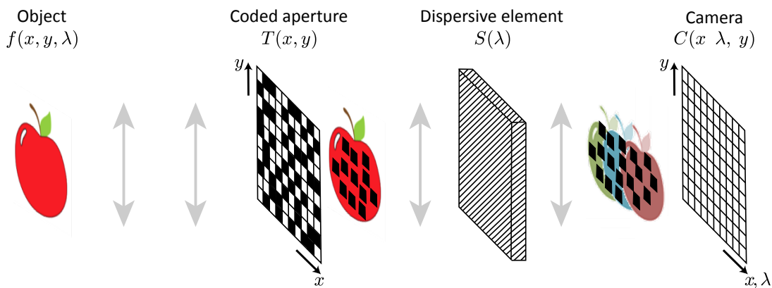
FIGURE 1.17: CASSI principle.
