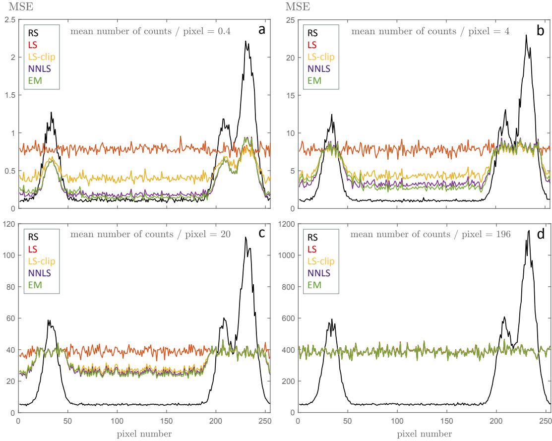
FIGURE 6.7: MSE per object pixel for object B and different signal levels. At low signal levels (a,b), the object background is close to zero so the least-square estimation leads to negative values and alternative algorithms improve the MSE on the background (compared to LS). At high flux, all estimators give similar MSE (d).
