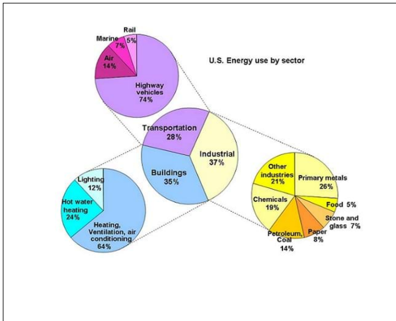
Figure I-7 : Relative energy use by sector (data from US DOE EIA)
