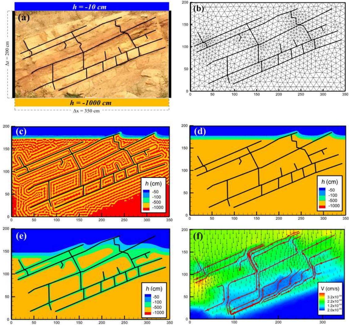
Fig. 5.6. The test case of infiltration in fractured dry soil: (a) synthetic description of the problem: Geometry, fracture network, and boundary conditions, (b) example of computational mesh, (c) pressure head map at t=3\text{h} with the MH-Cons-1D/2D code (without ML in fractures), (d) pressure head map at t=3\text{h} with the MH-Lump-1D/2D code (with ML in fractures), (e) pressure head map at t=9\text{h} with the MH-Lump-1D/2D code and (f) corresponding simultaneous representation of the velocity field, velocity magnitude and the streamlines in fractures.
