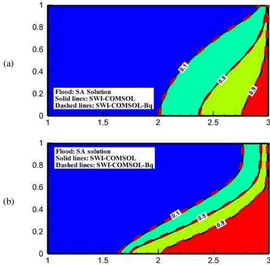
Fig. 4.3. Isochlors obtained using the semi-analytical solution (SA) and COMSOL model (with and without Boussinesq approximation) for the homogeneous test cases: (a) diffusive case and (b) dispersive case.
