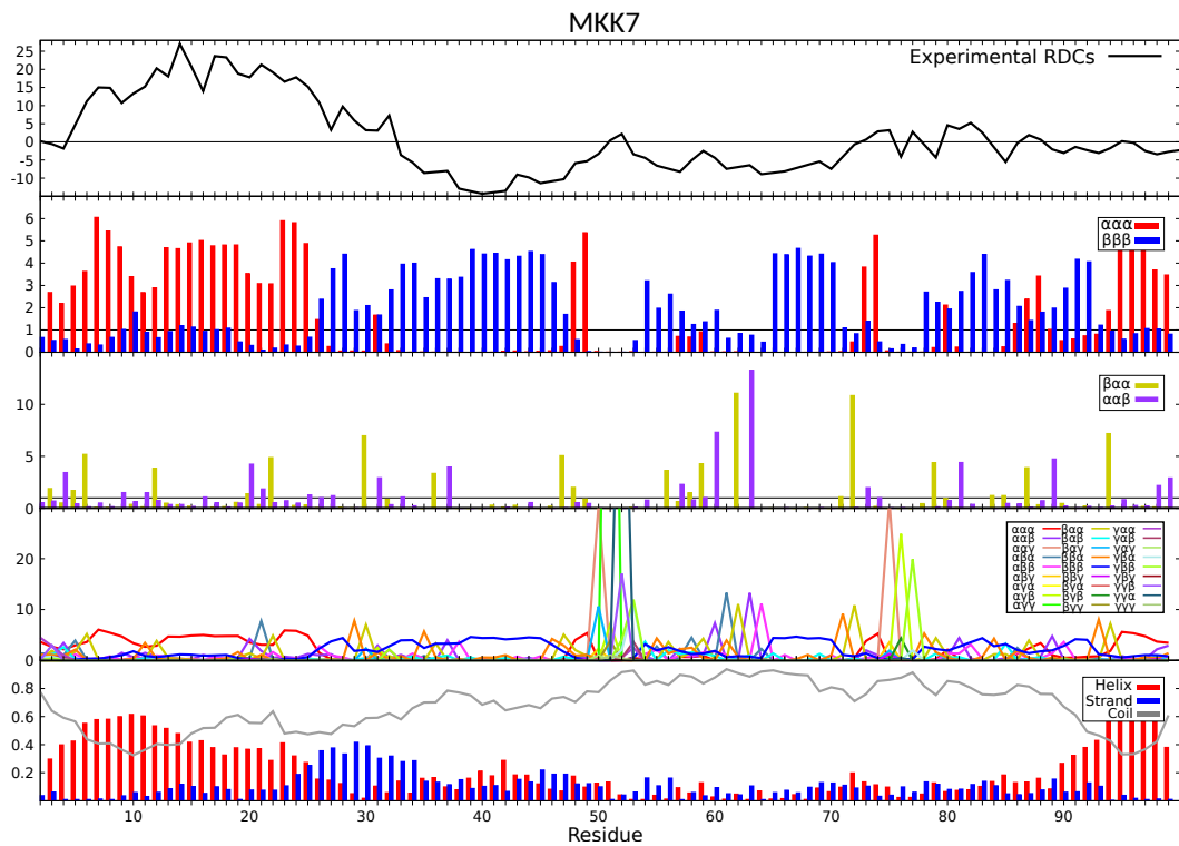
Figure 4.4. 5 panels with results for MKK7. From top to bottom: Experimental RDCs; \alpha\alpha\alpha and \beta\beta\beta propensity useful to identify helical and extended regions; \beta\alpha\alpha and \alpha\alpha\beta propensity useful to identify turns; The 27 structural classes propensities; s2D result.
