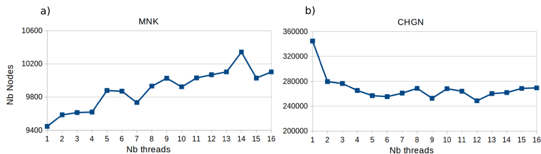
Figure 7.8. Evolution of the total number of nodes needed to solve the transition path-finding problem depending on the number of threads for the two peptides: a) MNK, b) CHGN.
