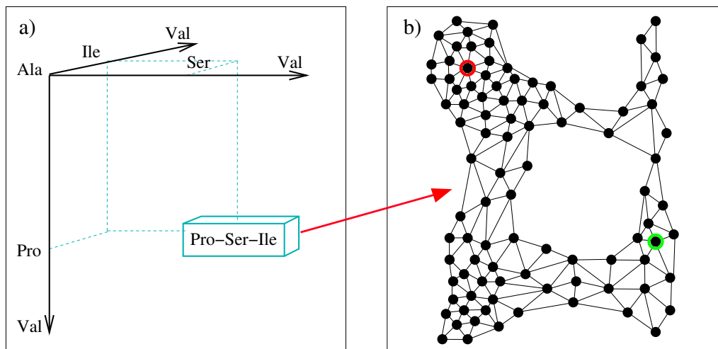
Figure 6.1. (a) Database containing one record for each tripeptide (8,000 in total). (b) For each tripeptide, the conformations recorded in the database are related with a proximity criterion and structured into an adjacency graph (the figure shows a simplified representation of this graph for tripeptide Pro-Ser-Ile).
