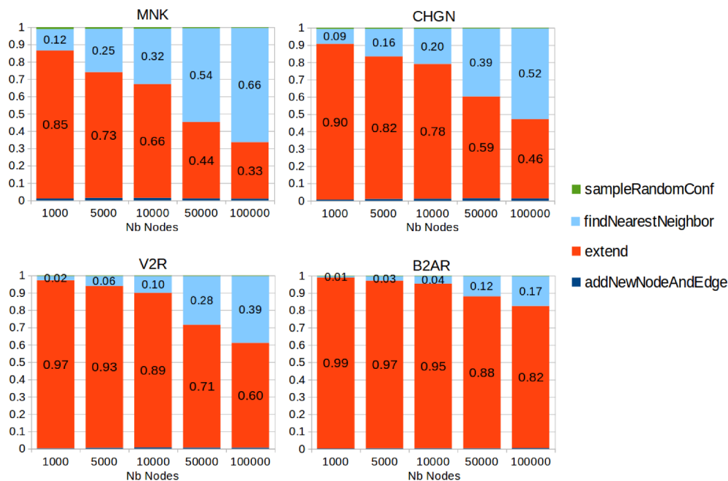
Figure 7.5. Computation time decomposition depending on the number of nodes in the trees for the four molecules under study.
