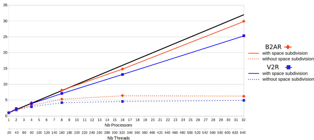
Figure 7.10. Evolution of the speed-up of the parallel algorithm with respect to the number of processors (working with 20 threads per processor). As a reference, the black line represents the linear speed-up.
