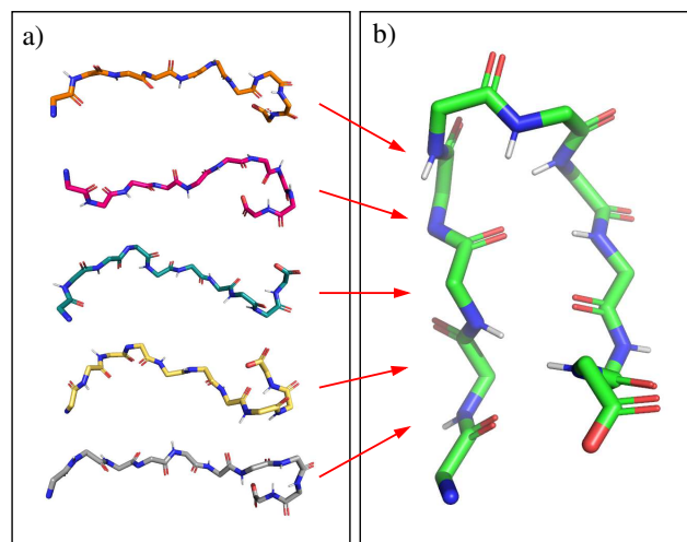
Figure 6.4. Structural representation of Chignolin. (a) A set of extended conformations involving the initial turn at the C-terminal side. (b) Folded conformation. Only the protein backbone is represented, using PyMOL [193].
