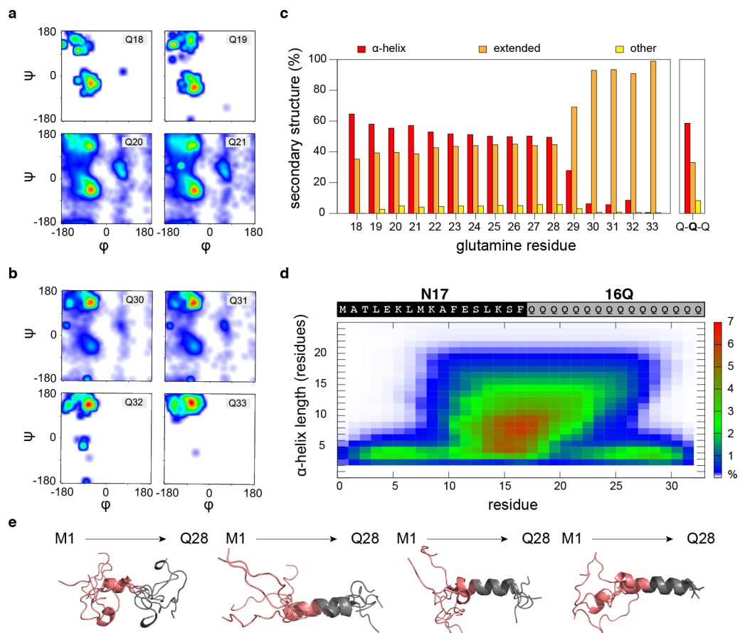
Figure 3. NMR-derived ensemble model of H16. Residue-specific Ramachandran plots for (a) Q18-Q21 and (b) Q30-Q33 obtained from the optimized ensemble. (c) Population of \alpha -helix, extended and other conformations calculated from the Ramachandran plot for all glutamines in H16 (see Figure S3). The side panel Q-Q-Q shows these populations for glutamine tri-peptides present in a coil database 49 . (d) Secondary structure map (SS-map) displaying the length and the residues encompassing the \alpha -helices found in the N-terminal region of the optimized ensemble model of H16. The color code (right) indicates the population of the \alpha -helices. (e) Representative conformations of the four ensembles used to describe the NMR CSs measured for H16. Only the region from M1 to Q28, optimized with the N \rightarrow C ensembles, is displayed. The SS-maps for these ensembles are displayed in Figure S4.
