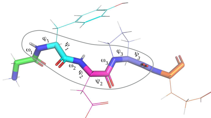
Figure 3.2. Illustration of a protein fragment involving 5 residues. Each residue is represented using a different color for the carbon atoms. The backbone is represented using thicker lines. Considering constant bond lengths, bond angles and peptide bond torsions, the protein backbone conformation can be defined from three angles ( \omega , \phi and \psi ) for each residue. The gray line indicates the tripeptide fragment.
