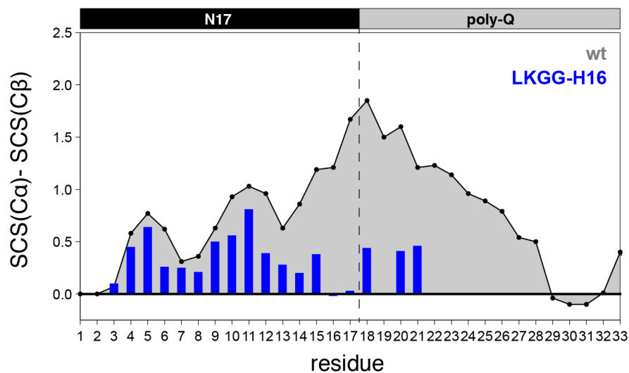
Figure S7. SCS analysis of LKGG-H16 in comparison with the wild-type. Secondary chemical shift analysis using experimental C \alpha and C \beta chemical shifts and a neighbor-corrected random-coil library POTENCI 46 for the wild-type (connected black points) and the LKGG-H16 mutant (blue histogram). Only residues belonging to N17 and the poly-Q tract are displayed. Data from Q18, Q20 and Q21 was obtained from SSIL samples; the other glutamines were not investigated.
