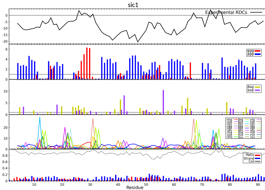
Figure 4.7. 5 panels with results for sic1 . From top to bottom: Experimental RDCs; \alpha\alpha and \beta\beta propensity useful to identify helical and extended regions; \beta\alpha and \alpha\beta propensity useful to identify turns; The 27 structural classes propensities; s2D result.
