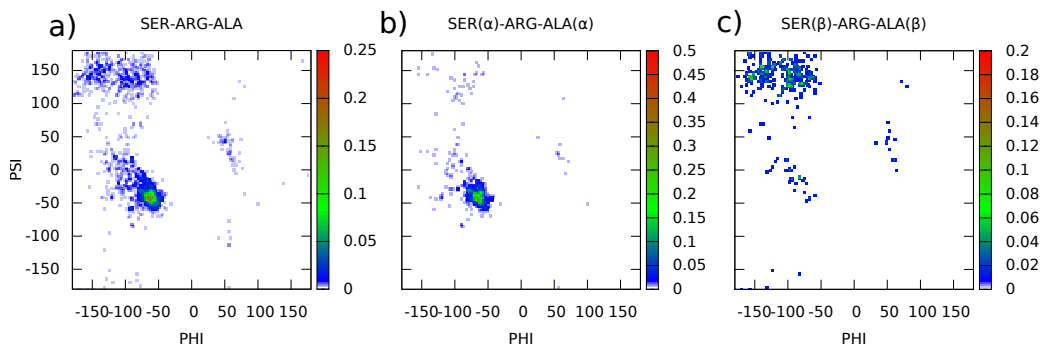
Figure 3.5. Distributions of the \phi - \psi angles of the central residue in a tripeptide, Ser-Arg-Ala, depending on the structure of the neighboring residues. (a) All the \phi - \psi angles for the central residue Arg, independently on the structure of Ser and Ala. (b) Angles for Arg when Ser and Ala are in the \alpha region. (c) Values for Arg when Ser and Ala are in the \beta /polyproline-II region.
