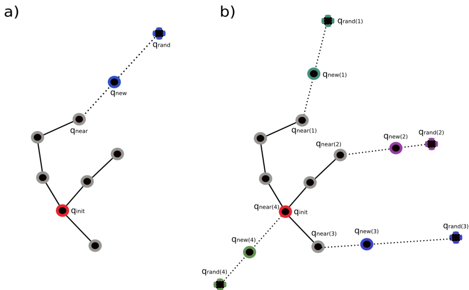
Figure 7.1. Illustration of the TRRT expansion process (for a single tree). The red node is the initial configuration and grey nodes have been generated in previous iterations. A new node q_{\text{new}} is created by the extension of the nearest node in the tree q_{\text{near}} toward a randomly sampled configuration q_{\text{rand}} . a) Mono-thread extension. b) Multi-thread extension, where k new nodes are generated in parallel.
