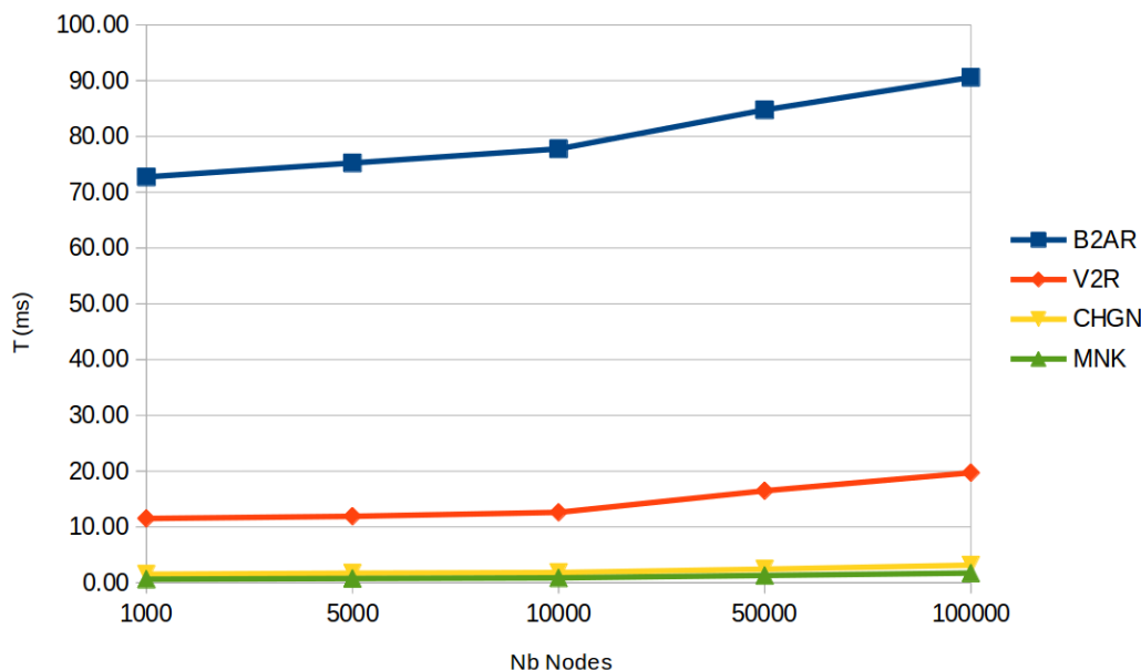
Figure 7.6. Evolution of the time per iteration with respect to the total number of nodes in the tree.
