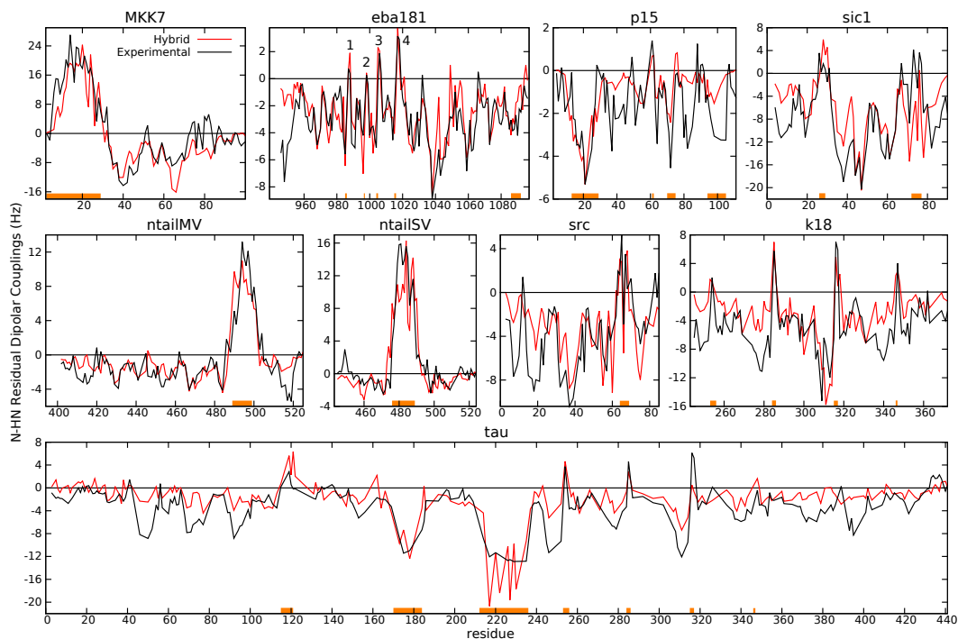
Figure 5.2. Experimental N-HN RDCs (black solid lines) for the nine IDPs studied compared with those computed using the hybrid SRS-TRS sampling strategy (red solid lines). Fragments highlighted in orange correspond to regions considered partially structured, for which the TRS was applied (see Table 5.3 for details).
