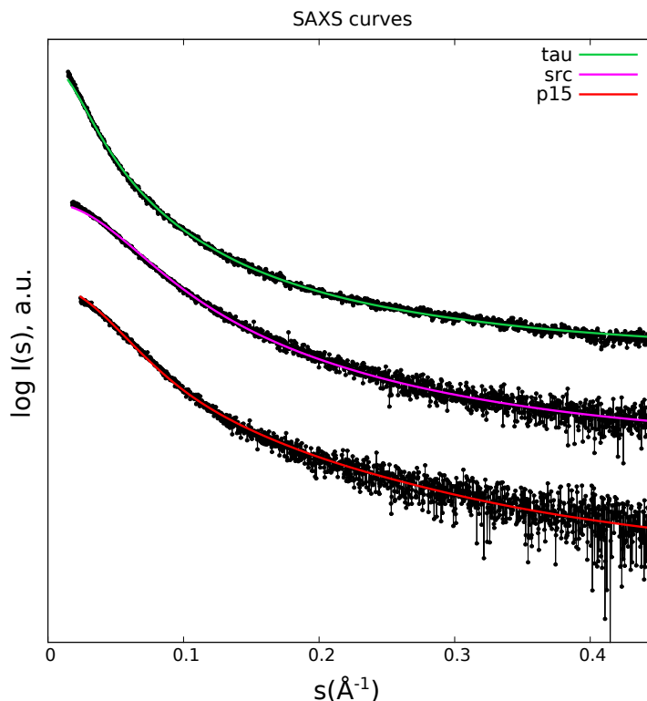
Figure 5.4. Experimental scattering intensity (black dots) in logarithmic scale as a function of the momentum transfer, s , compared with the averaged profiles computed from the hybrid ensemble models for tau (green), USrc (pink), and p15 (red). The profiles have been displaced along the y-axis for a better inspection.
