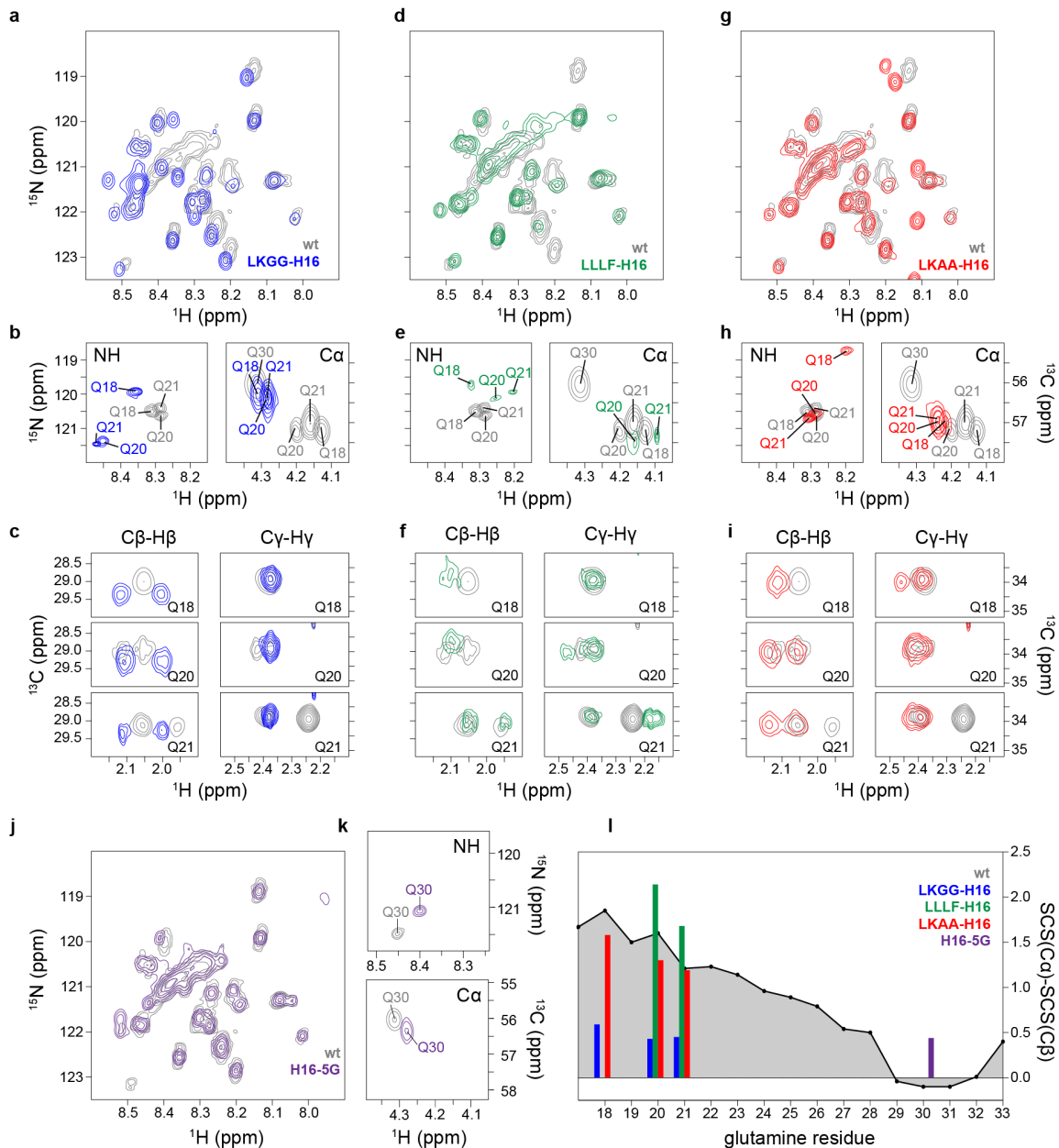
Figure 5. SSIL analyses of the structural effects of the flanking regions on the poly-Q tract of H16. Overlay of the glutamine region of the ^{15}\text{N} -HSQC spectra of fully labeled wild-type H16 (grey) with the N17 mutants LKGG-H16 ( a , blue), LLLF-H16 ( d , green), and LKAA-H16 ( g , red). The same color-code was used throughout the figure. Zoomed overlays of the ^{15}\text{N} - and ^{13}\text{C} -HSQCs for site-specifically labeled Q18, Q20 and Q21 of wild-type H16 (grey) with LKGG-H16 ( b ), LLLF-H16 ( e ) and LKAA-H16 ( h ). \text{C}\beta\text{-H}\beta and \text{C}\gamma\text{-H}\gamma NMR peaks of the Q18, Q20 and Q21 glutamine side chains of the three N17 mutants LKGG-H16 ( c ), LLLF-H16 ( f ) and LKAA-H16 ( i ) compared with those obtained for the wild-type (grey). Zoomed ^{15}\text{N} - and ^{13}\text{C} -HSQC spectra for the H16-5G mutant, which probes the structural perturbation exerted by the poly-P tract, displaying the N-H glutamine region ( j , purple) overlaid with the wild-type (grey), and the SSIL spectra measured for Q30 ( k ). ( l ) Histogram of the SCS analyses for the different SSIL samples of the structural mutants measured: Q18, Q20 and Q21 for the LKGG-H16, LLLF-H16 and LKAA-H16 mutants, and Q30 for the H16-5G mutant. The SSIL-derived SCS values are compared to those obtained for the wild-type (grey area). Note that no SCS value was derived for Q18 in the LLLF-H16 mutant due to the absence of the \text{C}\alpha\text{-H}\alpha peak in the ^{13}\text{C} -HSQC.
