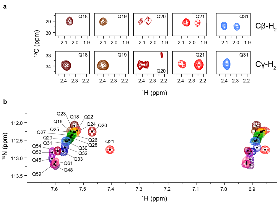
Figure 4. Side chain NMR scanning. (a) C \beta -H 2 and C \gamma -H 2 regions of the 13 C-NMR spectra of glutamines Q18, Q19, Q20, Q21, and Q31. The spectra of Q31 display the standard behavior of disordered glutamines with a doublet and singlet for C \beta -H 2 and C \gamma -H 2 , respectively. (b) Zoom on the N \epsilon 2-H \epsilon 2 side chain region of the 15 N-HSQC spectra measured for all glutamines in H16. Q20 and Q21 do not follow the trend displayed by the other glutamines due to their implication in the formation of hydrogen bonds.
