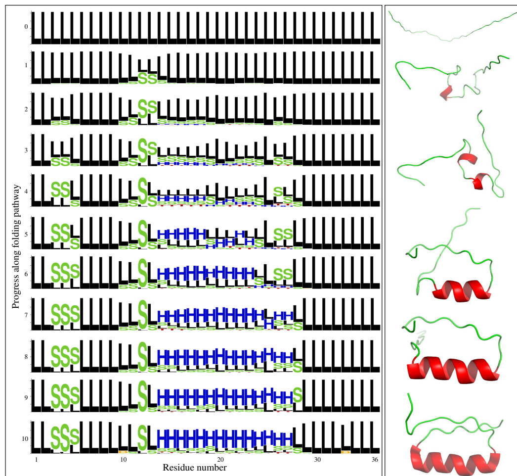
Figure 6.6. The left side panel represents the evolution of the structural propensities at the residue level along DS119 folding pathway. The right side panel shows some intermediate states along one of the computed folding paths. The "cartoon" representation clearly shows the formation of the helix. PyMOL [193] was used for the structural visualization.
