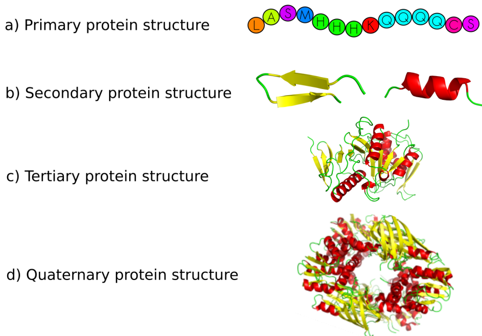
Figure 2.3. Representation of the four levels of protein structure: a) Primary protein structure, b) Secondary protein structure, c) Tertiary protein structure, d) Quaternary protein structure
