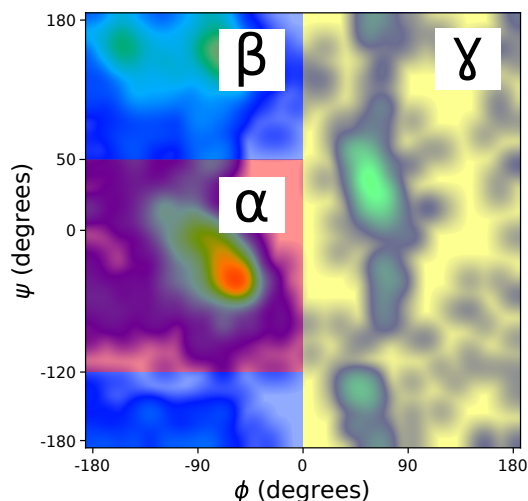
Figure 3.3. The Ramachandran regions were identified using definitions in related work [164]. Concretely, [\alpha : \phi \leq 0^\circ; -120^\circ \leq \psi < 50^\circ] , [\beta : \phi < 0^\circ; 50^\circ < \psi \leq 240^\circ] , [\gamma : \phi > 0] .
