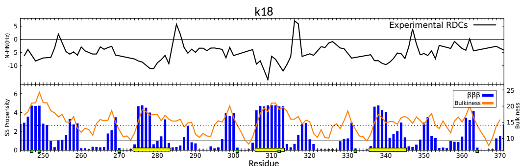
Figure 4.3. RDC profile (top, black line), \beta\beta\beta propensity (bottom, blue bars) and bulkiness profiles (bottom, orange line) for the K18 construct of Tau protein. The prolines are indicated with a green square. The dashed line situated at bulkiness = 14 indicates the threshold above which the amino acids are considered as bulky [29]. The three experimentally-characterized extended regions involving residues 275-282, 307-313 and 338-346 are highlighted in yellow.
