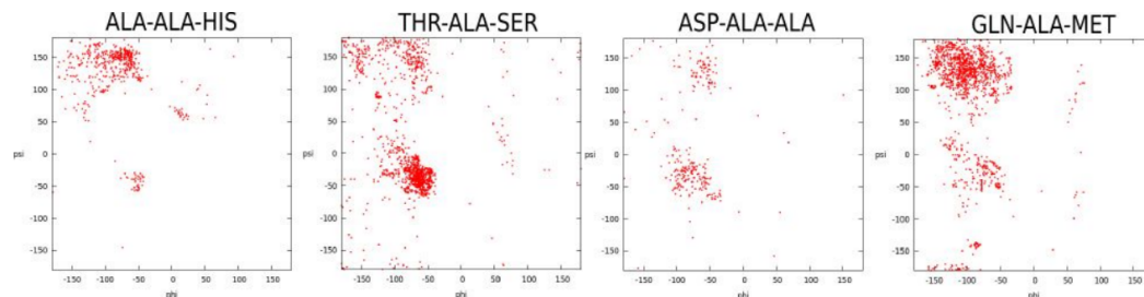
Figure 3.4. Distributions of the \phi - \psi angles of the central residue for four tripeptides having alanine as central residue. (a) Ala-Ala-His. (b) Thr-Ala-Ser. (c) Asp-Ala-Ala. (d) Gln-Ala-Met.
