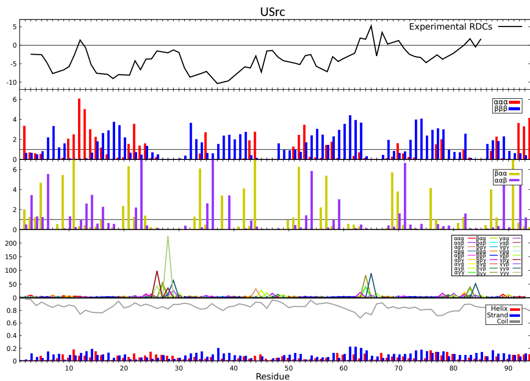
Figure 4.10. 5 panels with results for USrc. From top to bottom: Experimental RDCs; \alpha\alpha\alpha and \beta\beta\beta propensity useful to identify helical and extended regions; \beta\alpha\alpha and \alpha\alpha\beta propensity useful to identify turns; The 27 structural classes propensities; s2D result.
