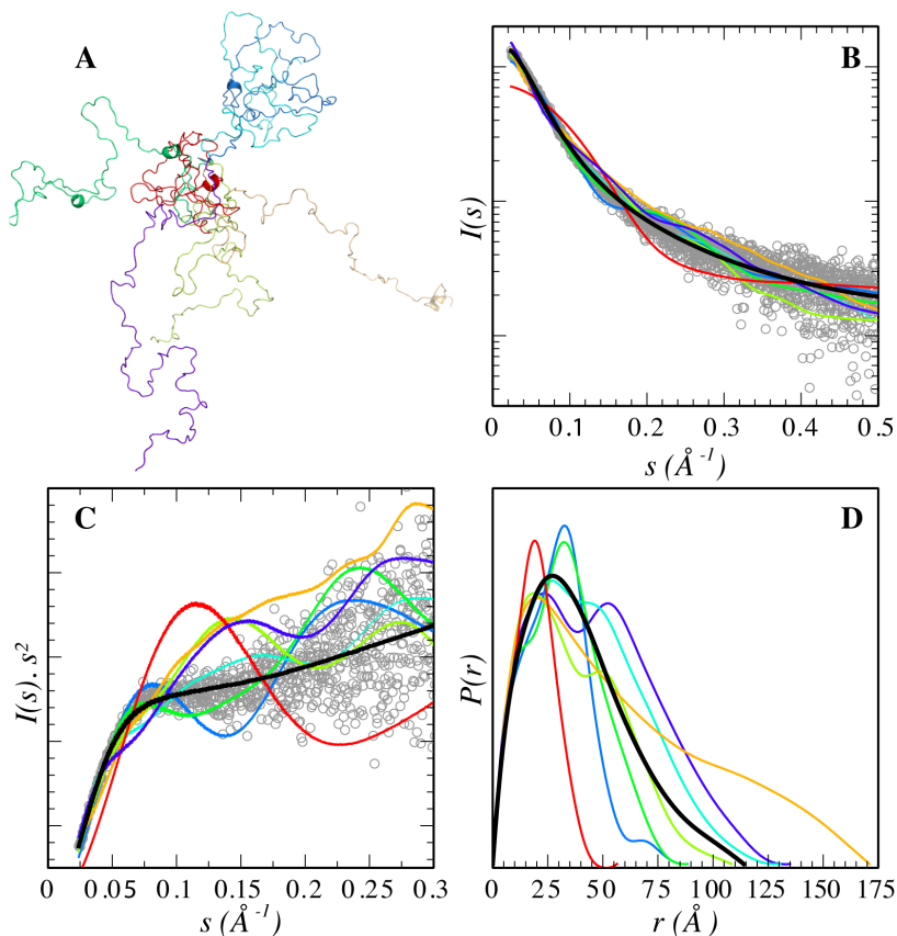
Figure 2.9. (A) Seven representative conformers randomly selected from an ensemble of 5,000 explicit all-atoms models generated for p15PAF [40]. Solid lines correspond to their computed curves (B) and Kratky plots (C) and are colored as in panel A. The average over the ensemble of 5,000 conformations yields a featureless curve that is in very good agreement with the experimental data (gray circles). (D) p(r) functions computed for the 7 conformers and the complete ensembles in the same color code that in panels (A-C). Figure extracted from [32]
