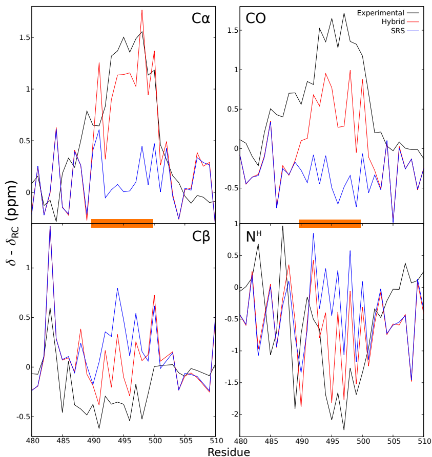
Figure 5.3. Comparison of the experimental (black) C\alpha , C\beta , CO and NH chemical shifts of ntailMV with these obtained from the ensembles built with the SRS (blue) and hybrid (red) strategies. Orange bars indicate these regions defined as structured in the hybrid modeling.
