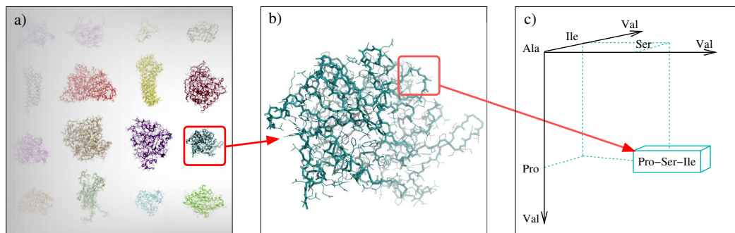
Figure 3.1. Construction of the tripeptide database: (a) A non-redundant set of experimentally determined protein structures is used as input. (b) For each protein, fragments of three consecutive residues (called tripeptides) are analyzed. (c) The structural information is stored in a database containing one record for each tripeptide (8,000 in total).
