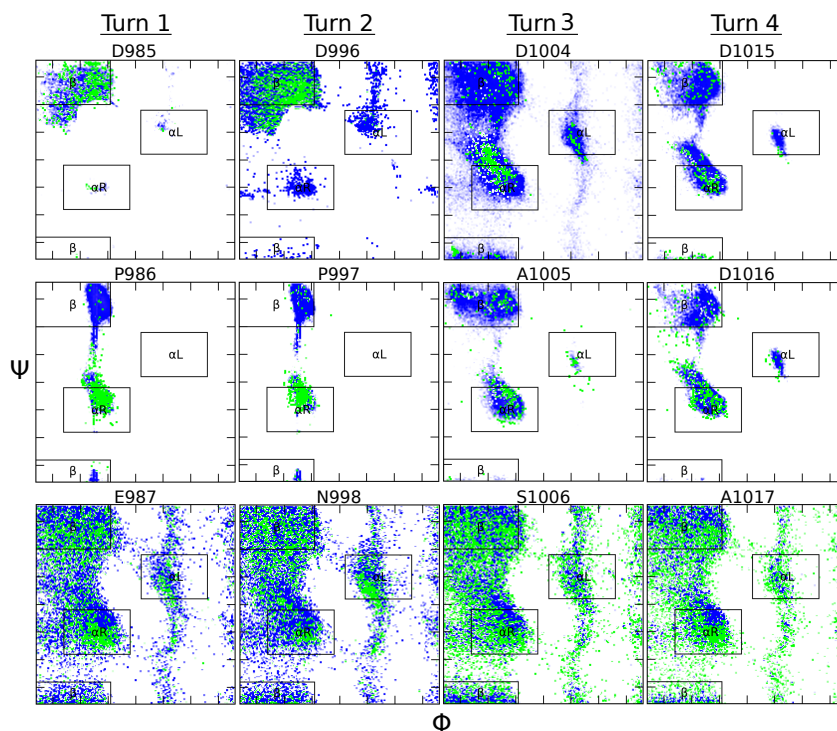
Figure 5.6. Conformational sampling for the four turns identified in eba181. Each column displays the Ramachandran plots for the three first residues in turns 1 to 4 when using the SRS (blue) or the hybrid (green) sampling approaches.
