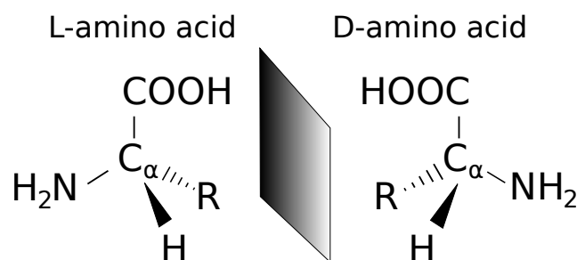
Figure 2.1. L-amino acid and D-amino acid representation with its \alpha -carbon, the amine group, the carboxylic group, the hydrogen and the side chain
