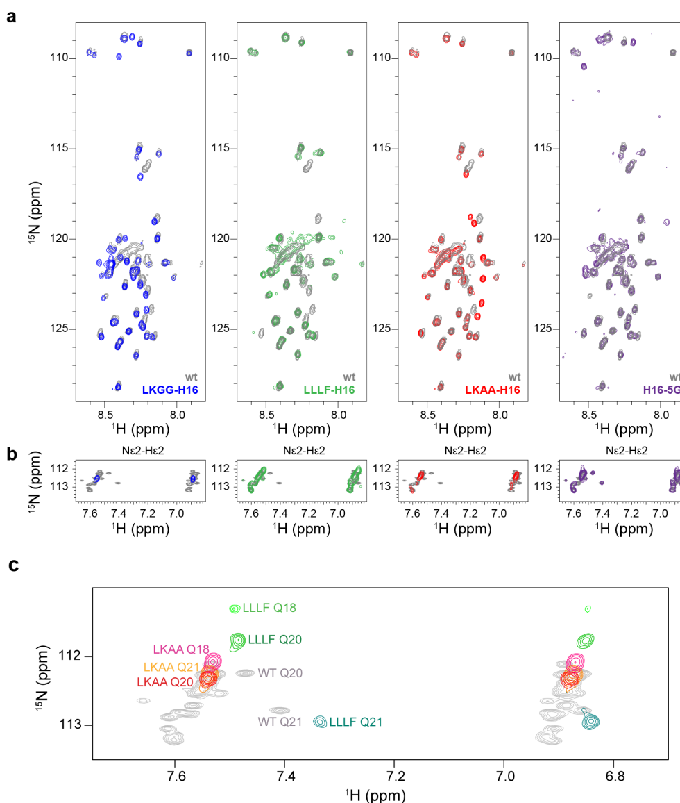
Figure S6: ^{15}\text{N} -HSQC spectra of the structural mutants in comparison with the wild-type. (a) Backbone spectra of wild-type H16 (grey) overlaid with LKGG-H16 (blue), LLLF-H16 (green), LKAA-H16 (red) and H16-5G (purple). (b) Side chain spectra corresponding to the same mutants using the same color code. Note that peaks corresponding to the first glutamines for the LLLF-H16 and LKAA-H16 are not displayed due to the lower intensity (see below). (c) Zoom of the \text{N}\epsilon\text{-H}_2 peaks for residues Q18, Q20 and Q21 of mutants LLLF-H16 and LKAA-H16 obtained from SSIL samples overlaid to the same region for the wild type protein in grey. Their chemical shifts substantiate the hydrogen bond network involving F17 in httex1 (see main text).
