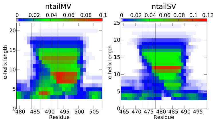
Figure 5.10. SS-map analysis for the helical regions in ntailMV and ntailSV displaying the length and the composing residues of the \alpha -helices found in ensembles generated with the hybrid sampling strategy for both proteins. Color from white to red indicates the population of these helices. Vertical lines indicate aspartic acids and serines in the sequence that act as helix N-capping residues. Concretely, D484, D487, S488, S491, and D493 are highlighted for ntailMV, and D473, D475, S477, and D478 and highlighted for ntailSV.
