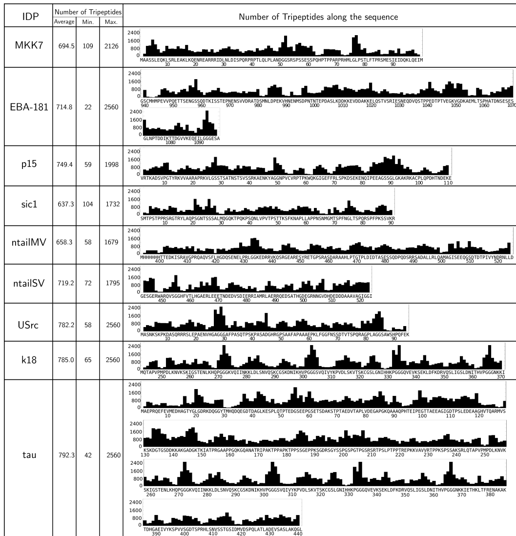
Figure 4.2. Number of structures in the tripeptide database for the tripeptides on the 9 IDPs benchmark. The value for each tripeptide is shown on its central residue.
