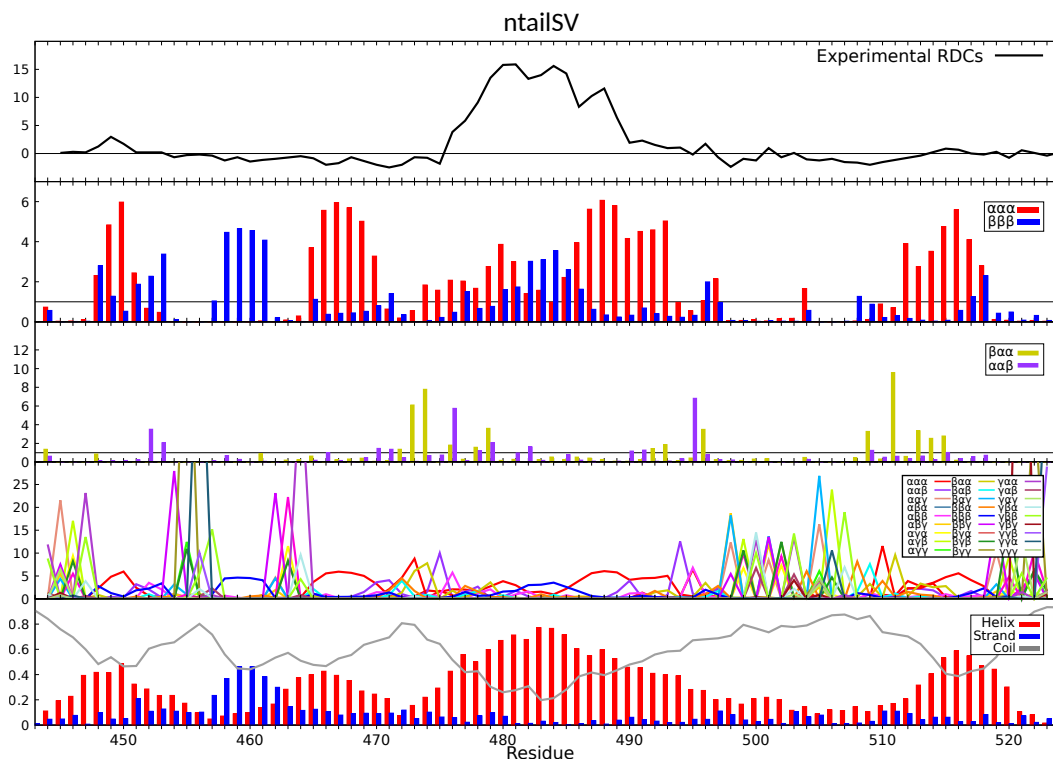
Figure 4.9. 5 panels with results for ntailSV. From top to bottom: Experimental RDCs; \alpha\alpha\alpha and \beta\beta\beta propensity useful to identify helical and extended regions; \beta\alpha\alpha and \alpha\alpha\beta propensity useful to identify turns; The 27 structural classes propensities; s2D result.
