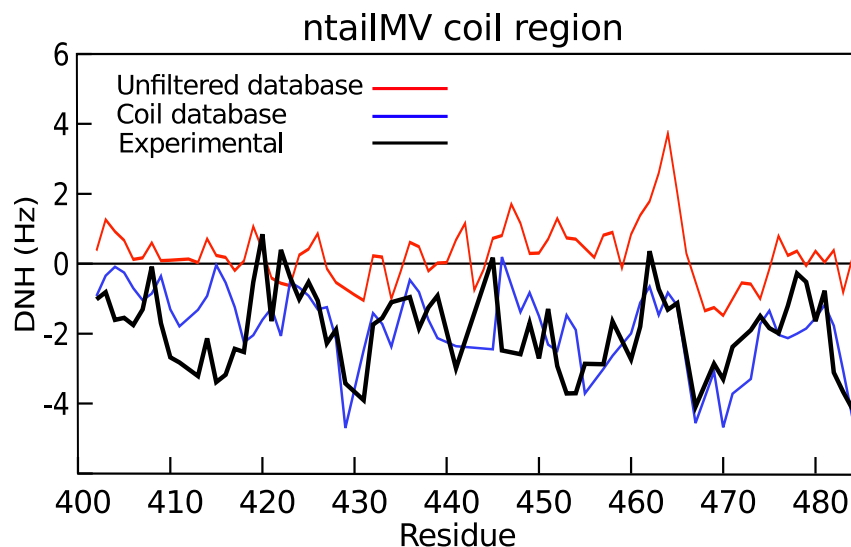
Figure 3.6. For the coil region of ntailMV: Experimental N-HN RDCs (black solid lines) compared with the theoretical RDCs computed from FM-like sampling using the unfiltered database (red solid line) and the coil database (blue solid line).
