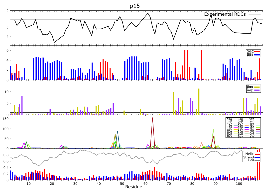
Figure 4.6. 5 panels with results for p15. From top to bottom: Experimental RDCs; \alpha\alpha\alpha and \beta\beta\beta propensity useful to identify helical and extended regions; \beta\alpha\alpha and \alpha\alpha\beta propensity useful to identify turns; The 27 structural classes propensities; s2D result.
