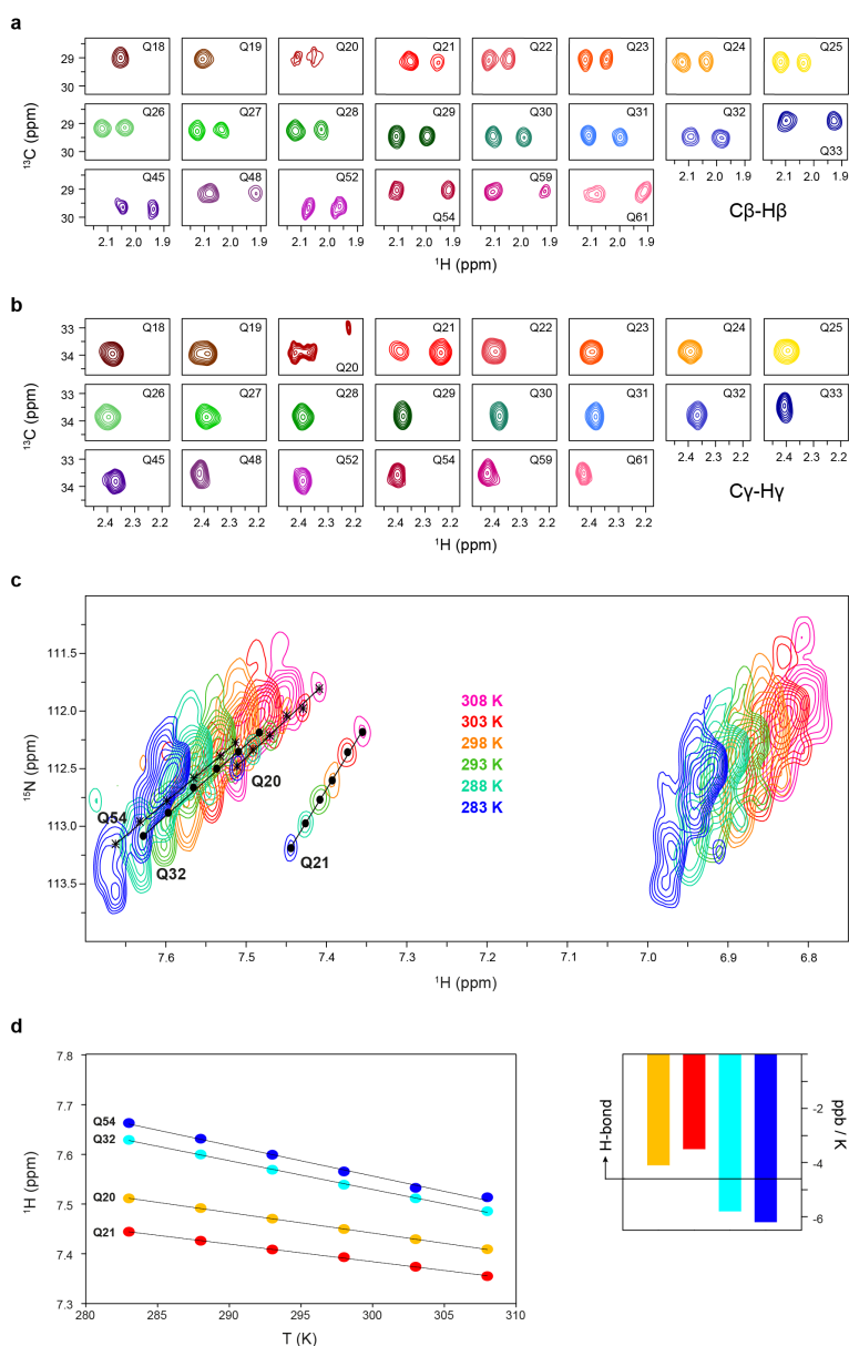
Figure S5: Side chain NMR scanning and temperature factors. (a) \text{C}\beta and (b) \text{C}\gamma ^{13}\text{C} -HSQC spectra for all glutamines in H16. With the exception of the first four glutamines (Q18-Q21), both families of spectra display a canonical behavior where \text{C}\beta - \text{H}_2 and \text{C}\gamma - \text{H}_2 are doublets and singlets, respectively. The color code is equivalent to the one used in Figure 1 in the main text. (c) Zoom of the \text{N}\epsilon - \text{H}_2 region of the ^{15}\text{N} -HSQC of fully labeled H16 measured at different temperatures. Solid lines connect the centers of the peaks for Q20, Q21, Q32 and Q54 at the different temperatures. Other peaks could not be unambiguously identified and therefore were not used in the analysis. (d, left panel) Linear fit of the ^1\text{H} frequency of the \text{N}\epsilon - \text{H}_2 peaks of the four residues plotted against the temperature. The slope of the linear fit (d, right panel) reports on the temperature coefficient and the probability of the atom to be involved in a hydrogen bond. According to these slopes, Q20 and Q21 side chains form a hydrogen bond, while Q32 and Q54 side chains do not.
