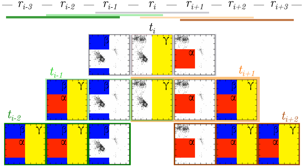
Figure 4.1. Ramachandran plots of residues in t_i , and in the neighboring tripeptides t_{i-2} , t_{i-1} , t_{i+1} and t_{i+2} . Colored regions correspond to the case where t_i is in the structural class \mathcal{S} = \beta\gamma\alpha . Notice that overlapping residues in consecutive tripeptides must be in the same structural class.
