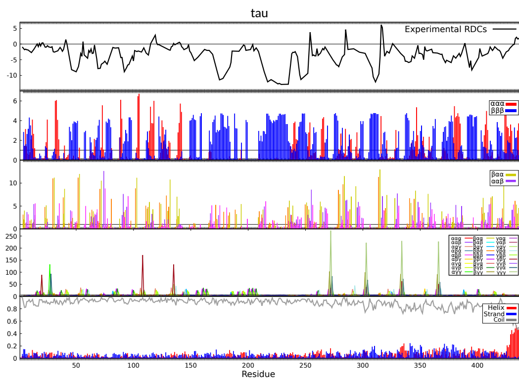
Figure 4.12. 5 panels with results for Tau. From top to bottom: Experimental RDCs; \alpha\alpha\alpha and \beta\beta\beta propensity useful to identify helical and extended regions; \beta\alpha\alpha and \alpha\alpha\beta propensity useful to identify turns; The 27 structural classes propensities; s2D result.
