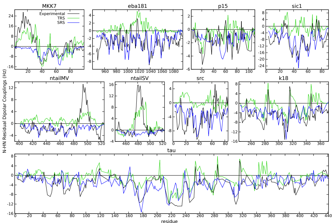
Figure 5.1. Experimental N-HN RDCs (black solid lines) for the nine proteins analyzed compared with the theoretical RDCs computed using the SRS (blue solid line) and TRS (green solid line) sampling strategies. To facilitate visual analysis, RDCs from the SRS method were scaled considering only the regions defined as random coil in the hybrid approach
