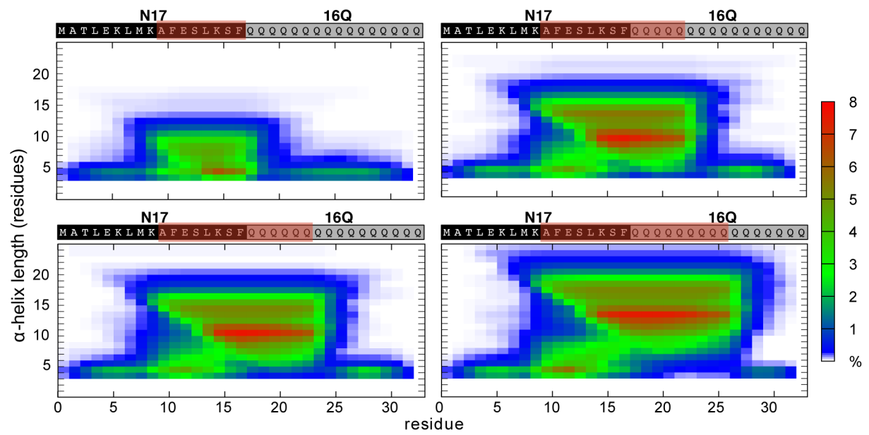
Figure S4. SS-maps for the four ensembles selected using the experimental CSs. Fragments considered as partially structured are highlighted in red on the top of each panel. The percentage of the \alpha -helical fragments is indicated in a color scale from high (red) to low (blue) populations.
