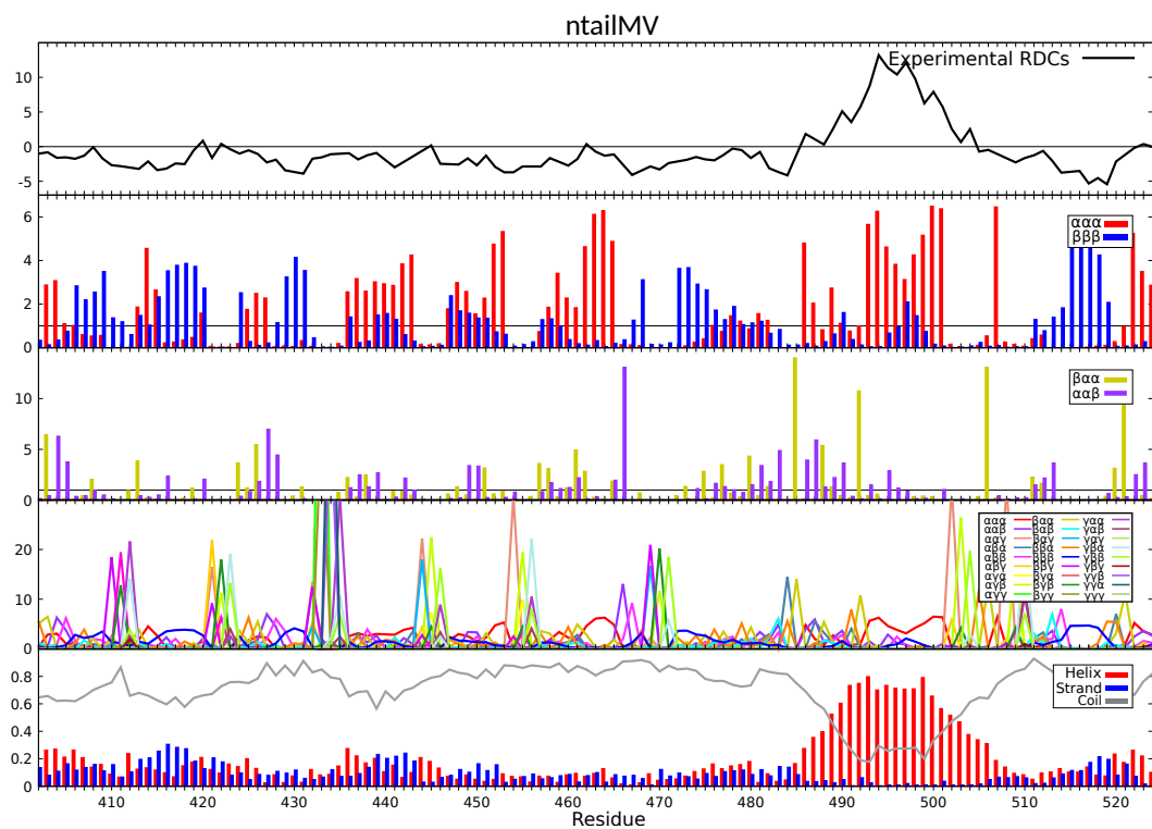
Figure 4.8. 5 panels with results for ntailMV. From top to bottom: Experimental RDCs; \alpha\alpha\alpha and \beta\beta\beta propensity useful to identify helical and extended regions; \beta\alpha\alpha and \alpha\alpha\beta propensity useful to identify turns; The 27 structural classes propensities; s2D result.
