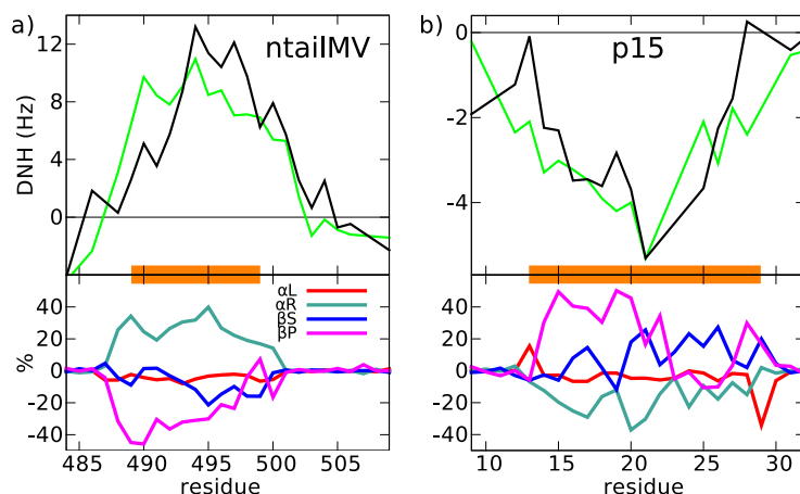
Figure 5.5. Experimental (black) and hybrid building model (green) N-HN RDCs for two fragments of (a top) ntailMV and (b top) p15. Fragments highlighted in orange were considered partially structured and built using the TRS strategy. In bottom panels, the percentage of enrichment of secondary structure classes present in the ensemble built with the hybrid strategy compared with that built with the SRS strategy. Secondary structure classes were identified using definitions in related work [164]. Concretely, [\beta S : -100 > \phi; -120 > \psi > 50] , [\beta P : 0 > \phi > -100; -120 > \psi > 50] , [\alpha R : 0 > \phi; 50 > \psi > -120] , [\alpha L : \phi > 0] .
