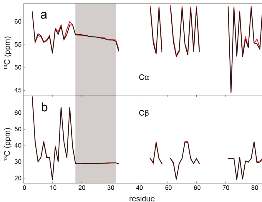
Figure S2. Chemical Shift (CS) based ensemble refinement of H16. Experimental (black) vs. ensemble-optimized (red) for all (a) C \alpha and (b) C \beta CSs measured for H16. The M1-Q28 and the Q29-P83 fragments of the optimized profile were built from those optimized using the N \rightarrow C and N \leftarrow C ensembles, respectively. The poly-Q tract is shaded in gray; gaps are due to proline residues for which we do not have experimental data.
