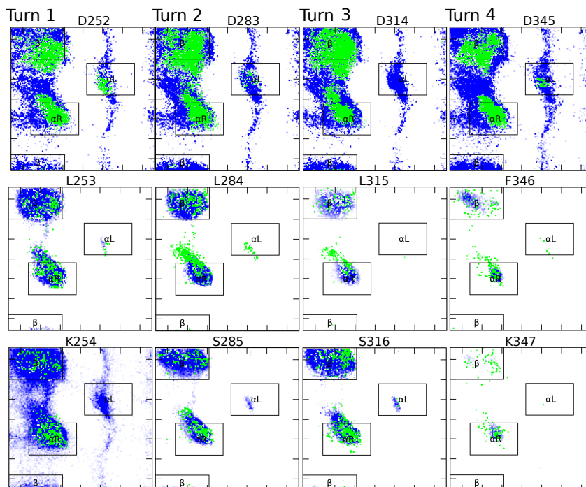
Figure 5.7. Conformational sampling for the four turns identified in K18. Each column displays the Ramachandran plots for the first three residues belonging to turns 1 to 4 when using the SRS (blue) or the hybrid (green) sampling approaches.
