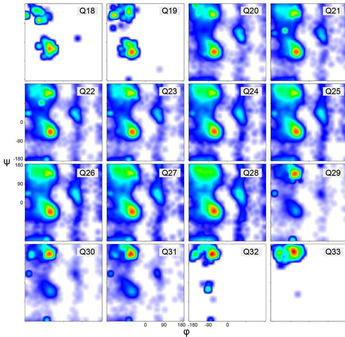
Figure S3. Ramachandran distribution for the glutamine residues of the poly-Q tract of H16 derived from the CS-optimized ensemble of H16. The populations of \alpha -helical ( 0 > \phi; 50 > \psi > -120 ), extended ( 0 > \phi; -120 > \psi > 50 ), and other ( 0 < \phi ) conformations are reported in Figure 3c in the main text. The red color indicates a higher density of conformations.
