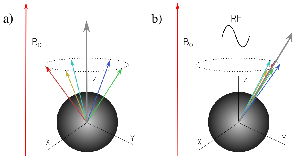
Figure 2.5. Schematic representation of a Nuclear Magnetic Resonance experiment. The applied magnetic field (vertical red vector) orientates the atom spins to precess around the direction of field. a) More nuclei are oriented in the sense of the field represented with vectors of different colors, but because the nuclei are precessing incoherently the resulting bulk magnetization, grey vector, is pointing in the direction of the magnetic field. b) After pulsing the radio frequency, all nuclei precess coherently around the magnetic field direction and a net bulk magnetization appears.
