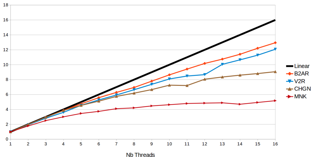
Figure 7.7. Evolution of the speed-up of the parallel algorithm running on a single (multi-core) processor for the four molecules. As a reference, the black line represent the linear speed-up.
