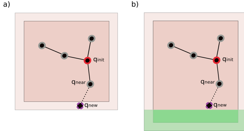
Figure 7.3. Illustration of the concept of a bounding n-polytope of a tree and its growth process. a) A new node is created near the boundary of the n-polytope, represented by the light brown region. b) The n-polytope is extended around the node (new green region).
