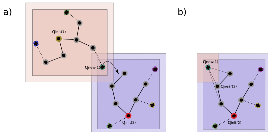
Figure 7.4. Illustration of the tree junction process. a) The extension of \mathcal{T}_1 generates a new node q_{\text{new}(1)} in the intersection of bounding n-polytopes \mathcal{S}_{1,2} . b) The processor in charge of the construction of \mathcal{T}_2 tries to connect q_{\text{new}(1)} to the nearest neighbor.
