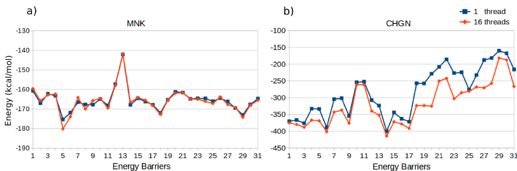
Figure 7.9. Energy profiles along the solution paths obtained using 1 thread and 16 threads for the two peptides: a) MNK, b) CHGN.
