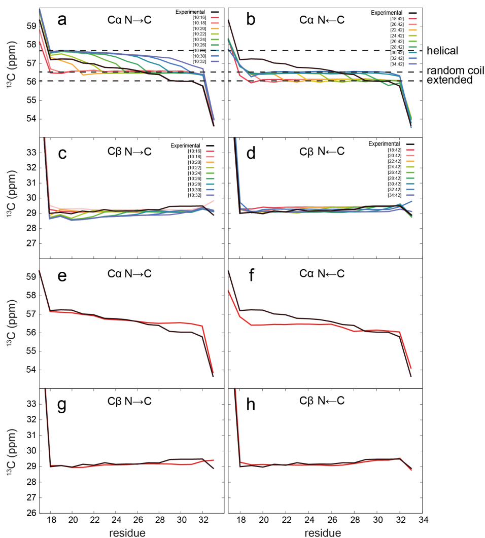
Figure S1. Chemical Shift (CS) based ensemble refinement of H16. (a-d) Overlay of the experimental (black) and theoretical (color) C\alpha (a and b) and C\beta (c and d) CSs of the poly-Q tract computed for the N\rightarrow C (a and c) and the N\leftarrow C (b and d) families of ensembles. The ensembles were built by incrementally incorporating glutamines in the partially structured region from Q18-Q33 ( N\rightarrow C ) and from Q33 to Q18 ( N\leftarrow C ). The boundaries chosen for the partially structured regions for each of the 5,000 conformation ensembles are indicated in the panel. Horizontal dashed lines indicate the three plateaus corresponding to helical, random coil and extended averaged conformations. Experimental (black) vs ensemble-optimized (red) C\alpha (e and f) and C\beta (g and h) CSs exclusively fitted with the N\rightarrow C (e and g) or the N\leftarrow C (f and h) ensembles. For the N\rightarrow C only C\alpha and C\beta experimental CSs from residues Q18-Q28 were used in the optimization. The reweighted model consisted of [10:17; 46.17%], [10:22; 26.93%], [10:23; 5.92%], and [10:26; 20.98%], where [X:Y] refers to the first and last residues considered as partially structured in the model. For the N\leftarrow C only C\alpha and C\beta experimental CSs from residues Q29-Q33 were used in the optimization. The reweighted model consisted of [22:42; 46.05%], [28:42; 0.8%], [29:42; 42.86%], and [34:42; 10.28%].
