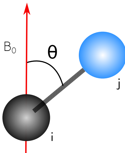
Figure 2.6. Representation of the angle \theta formed between the magnetic field B_0 and the vector connecting the two bonded atoms i and j
