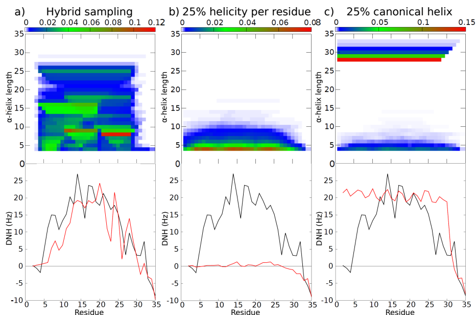
Figure 5.8. Structural analysis of the helical region in MKK7. (Top panels) Length and encompassing residues of the \alpha -helices found in ensembles computed using (a) the hybrid sampling and two theoretical models imposing (b) 25% of enhanced helicity per residue, and (c) 25% population of a canonical \alpha -helix in the 28-residue long segment. Colors from white to red indicate the population of helical segments found in the ensembles. (Bottom panels) Theoretical RDCs calculated from the above described ensembles (red lines) compared with the experimental ones (black lines).
