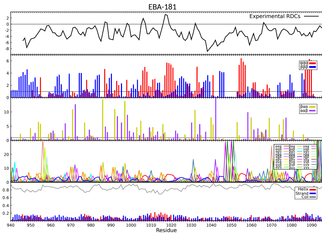
Figure 4.5. 5 panels with results for eba181. From top to bottom: Experimental RDCs; \alpha\alpha\alpha and \beta\beta\beta propensity useful to identify helical and extended regions; \beta\alpha\alpha and \alpha\alpha\beta propensity useful to identify turns; The 27 structural classes propensities; s2D result.
