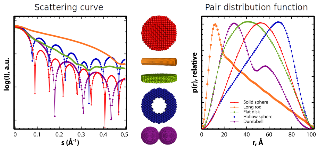
Figure 2.8. Scattering curves and pair-wise distance distribution functions for 5 particles (sphere, long rod, flat disk, hollow sphere, and dumbbell) with the same size and different shapes. From pair distribution functions is easier to intuitively identify the original shapes of the particles than using the scattering curve. Figure inspired from [113]
