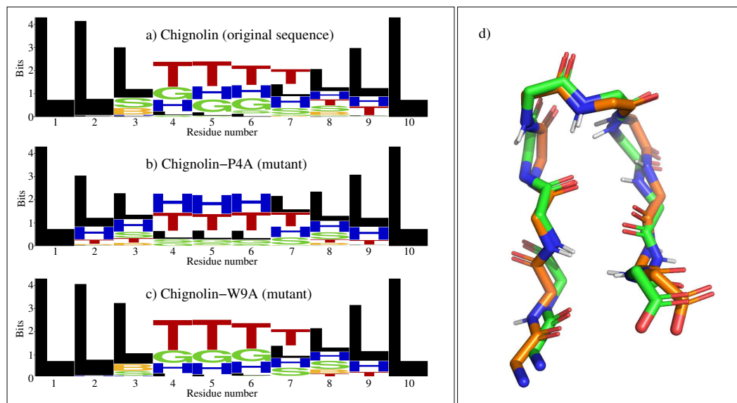
Figure 6.3. The left side panel represents the structural propensities at the residue level observed from a set of 1,000 conformations randomly generated from the structural database. Each plot displays the DSSP structural classes using the WebLogo format for (a) Chignolin, and two mutants: (b) Chignolin-P4A, and (c) Chignolin-W9A. (d) Structural representation of Chignolin: superposition of an experimentally determined structure (with carbon atoms in green) and the closest one in the set of 1,000 sampled conformations (with carbon atoms in orange). For clarity, only the protein backbone is represented, using PyMOL [193].
