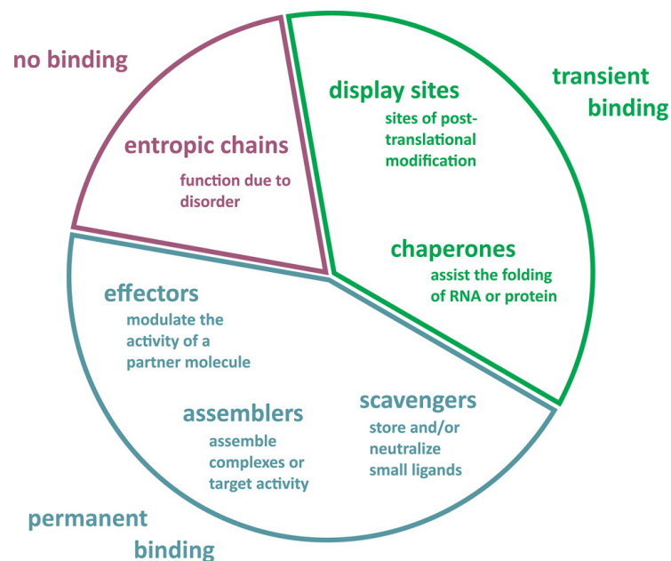
Figure 2.4. Functional classification of IDRs. Figure obtained from reference [231]
