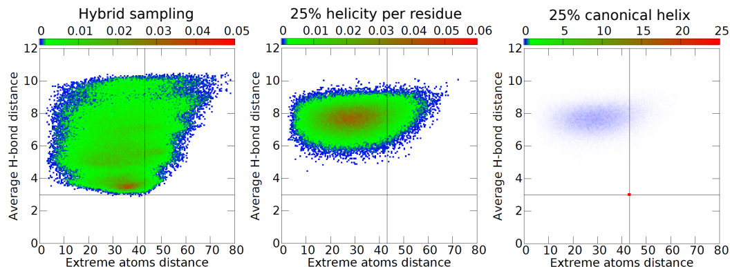
Figure 5.9. Deviation with respect to a canonical helix of conformations of the N-terminal region of MKK7 generated using different sampling strategies. The abscissa axis corresponds to the distance between the first N and last C backbone atoms of the 28-residue long structured region of MKK7. The ordinate axis corresponds to the average distance between H-bond donor and acceptor atoms. For a canonical 28-residue long helix these values are 3 Å and 43.5 Å, respectively.
