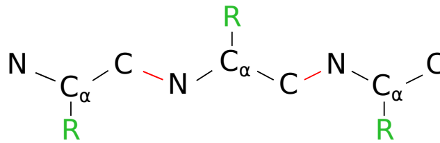
Figure 2.2. Simplified representation of a protein. In red the peptidic bonds, in black the backbone atoms and in green the residue side chains
