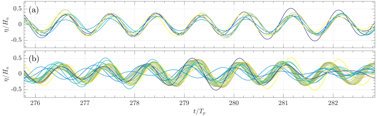
Figure V.16: Normalized surface elevations (a) at the location of gauge 22 for cases A to H, and (b) for case A at the locations of probes 1 to 22. Components of frequency higher than 1.4f_p have been removed using a low-pass filter.
