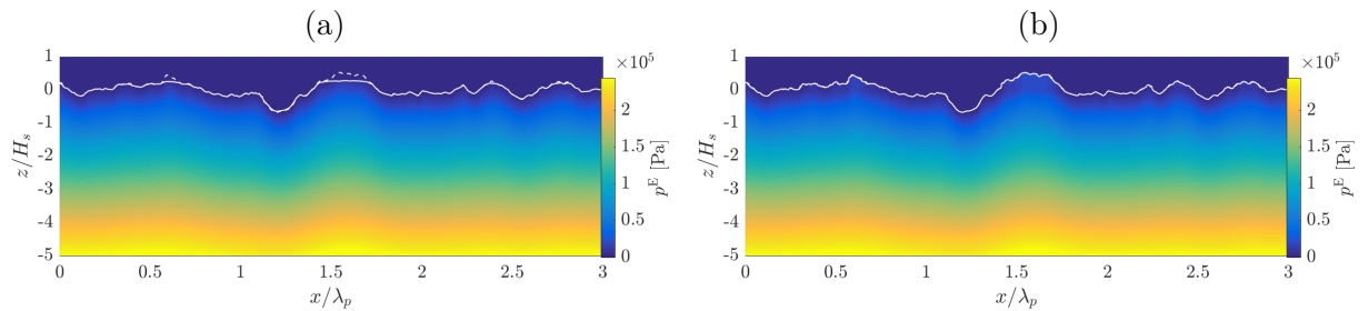
Figure II.22: Eulerian approximate of the second-order Lagrangian pressure field for a JONSWAP spectrum ( H_s = 5 m, T_p = 10 s, \gamma = 3.3 ) at t = 0 using (a) equation (II.25) and (b) a convergence scheme. The dashed lines on correspond to the surface elevation, while the continuous line is the pressure contour line p = p_a = 0 .
