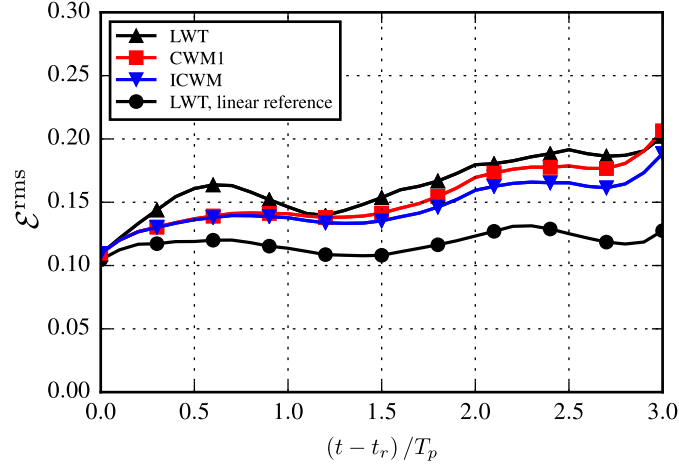
Figure IV.3: Prediction error of a nonlinear ocean surface as a function of time, for different wave models, using a uniform observation grid for K = 1 (i.e., only spatial observations).
