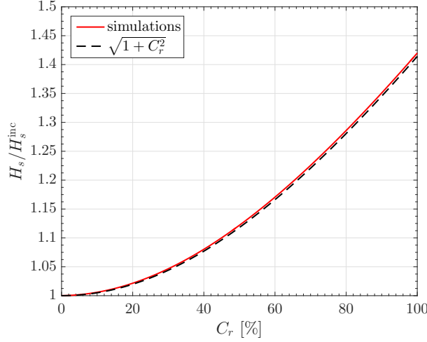
Figure V.12: Contribution of reflected waves on the estimated significant wave height as a function of the reflection coefficient. Results from Matlab simulations based on a linear JONSWAP spectrum and from the theoretical formula (V.3) are plotted.
