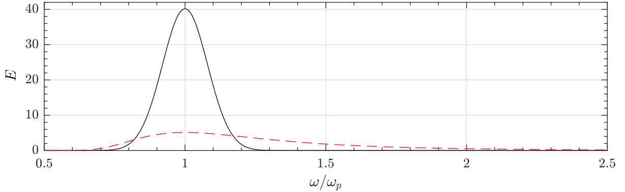
Figure II.10: Energy density spectrum as a function of the dimensionless angular frequency \omega/\omega_p , for a narrow (Gauss, solid line) or broad-banded (JONSWAP, dashed line) spectrum. The characteristic steepness is H_s/\lambda_p \approx 6\% and 4\% for each case, respectively.
