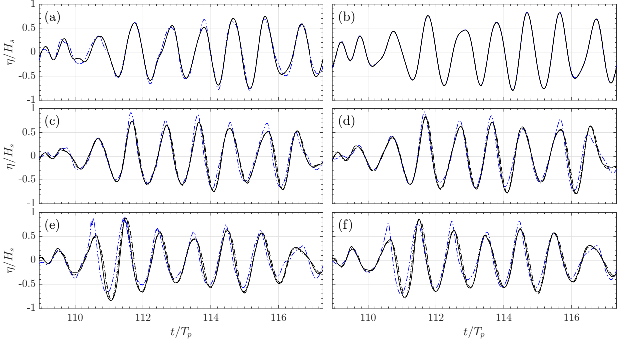
Figure V.23: Time series of surface elevations measured/simulated at probe 22 for a group of 8 waves (---) for cases: (a, b) A, (c, d) E and (e, f) H, of increasing nonlinearity. Predicted surface elevations are shown for the: linear (LWT, ----), corrected linear (LWT-CDR, .....), and nonlinear (ICWM, —) models. Left (a, c, e): experiments; right (b, d, f): simulations.
