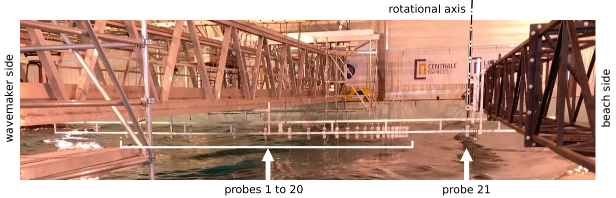
Figure V.3: Photo of the ladder upon which the wave probes are mounted. The whole ladder can be rotated around a vertical axis located at the horizontal location of the probe 21.
