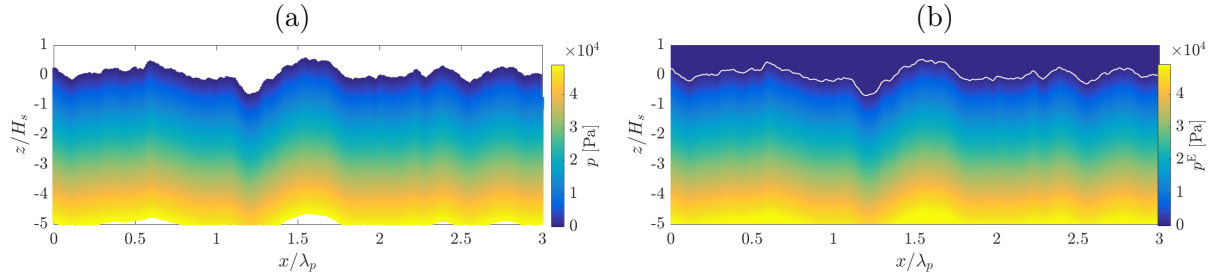
Figure II.21: (a) Lagrangian pressure field up to the second-order and (b) its approximate in the Eulerian framework for a JONSWAP spectrum ( H_s = 1 m, T_p = 10 s, \gamma = 3.3 ) at t = 0 . The dashed line on (b) corresponds to the surface elevation, while the continuous line is the pressure contour line p = p_a = 0 .
