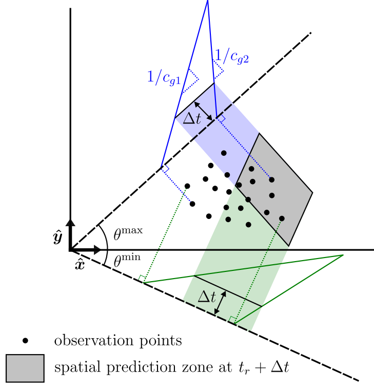
Figure III.9: Location of the prediction zone for a two-dimensional set of observations after a propagation time of t = t_r + \Delta t . It is approximated by the intersection of the one-dimensional prediction zones calculated at two extreme directions.
