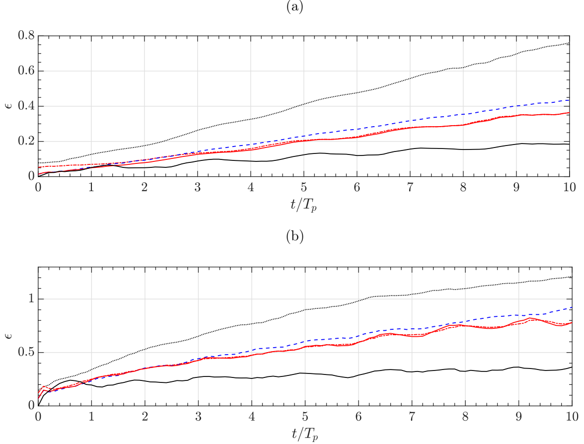
Figure II.12: Time evolution of relative errors (equation (II.21)) for the two cases of figure II.11 (a and b), for the linear (.....), CWM2 (---), ICWM (-.-.-) and ICWM with interaction terms (—) model results. The black solid line shows the relative change (equation (II.22)) of the prescribed spectrum during the HOS time evolution.
