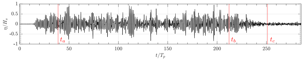
Figure V.13: Time series of surface elevation measured in experiments at probe 22 for case E (table V.2). Three characteristic times are marked on the record, t_a : all the generated wave components have been measured at all probes; t_b : shutdown of the wavemaker; t_c : all the generated wave components have propagated past all probes.
