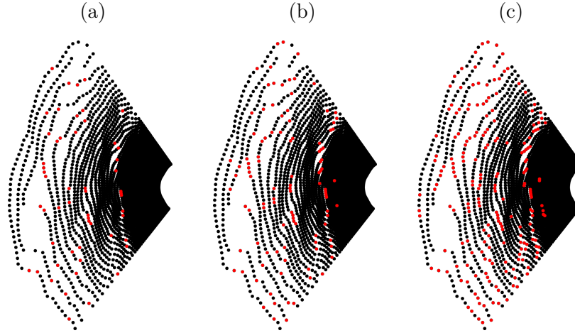
Figure III.5: Distribution of the discriminated points (●) over a set of spatial measurements (●) for three different limiting ray angles of incidence with respect to the surface, \alpha_i^{\text{lim}} = (a) 3^\circ , (b) 4^\circ and (c) 5^\circ . Sea state and optical sensor parameters are the same as in figure III.4.
