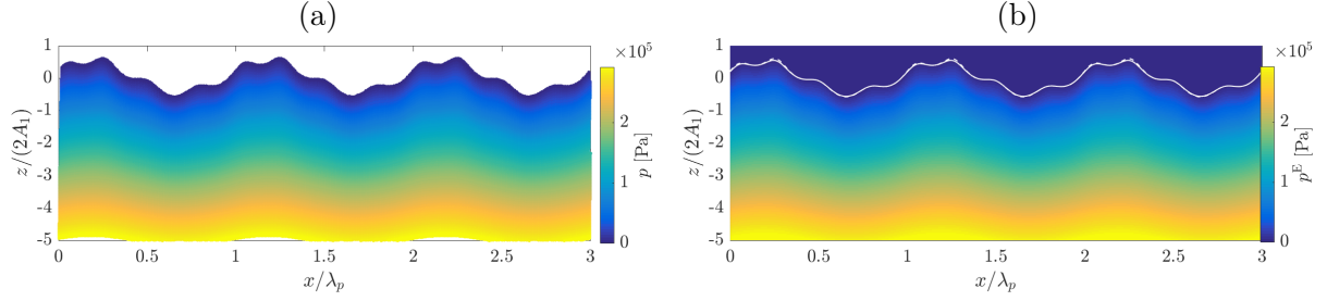
Figure II.20: (a) Lagrangian pressure field up to the second-order and (b) its approximate in the Eulerian framework for a bichromatic wave field at t = 0 . The dashed line on (b) corresponds to the surface elevation, while the continuous line is the pressure contour line p = p_a = 0 . ( A_1 = 3 m, A_2 = 0.75 m, T_1 = 10 s, T_2 = 5 s)
