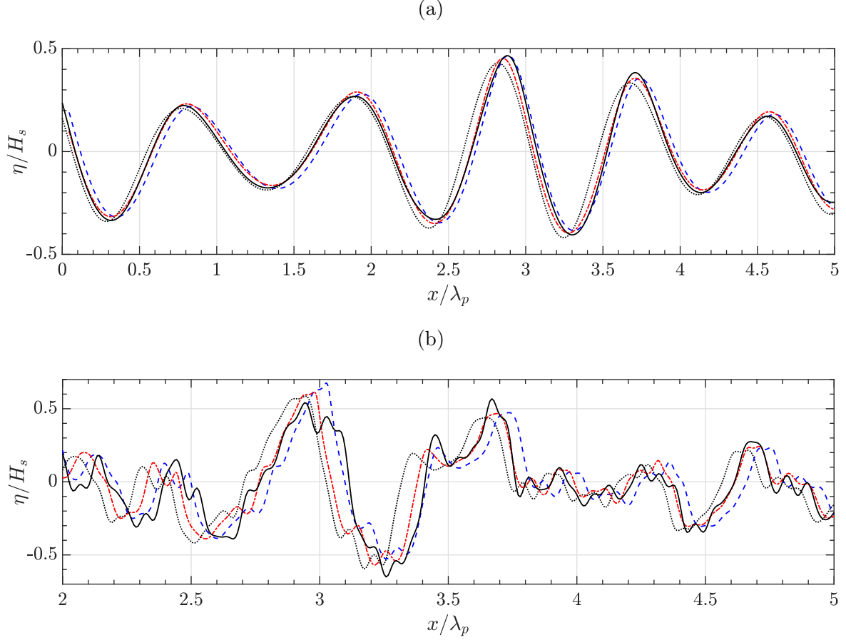
Figure II.11: Normalized surface elevations computed with: HOS (—), linear (.....), CWM2 (---), and ICWM (-.-.-) models, after t = 4T_p of propagation, for irregular wave trains with T_p = 10 s extracted from a: (a) Gaussian spectrum with standard deviation \sigma/\omega_p \approx 0.08 , H_s = 9 m and characteristic steepness H_s/\lambda_p \approx 6\% , and (b) a JONSWAP spectrum with peakedness parameter \gamma = 1 (similar to a PM spectrum), H_s = 6 m, and H_s/\lambda_p \approx 4\% . See figure II.10 for spectral shapes.
