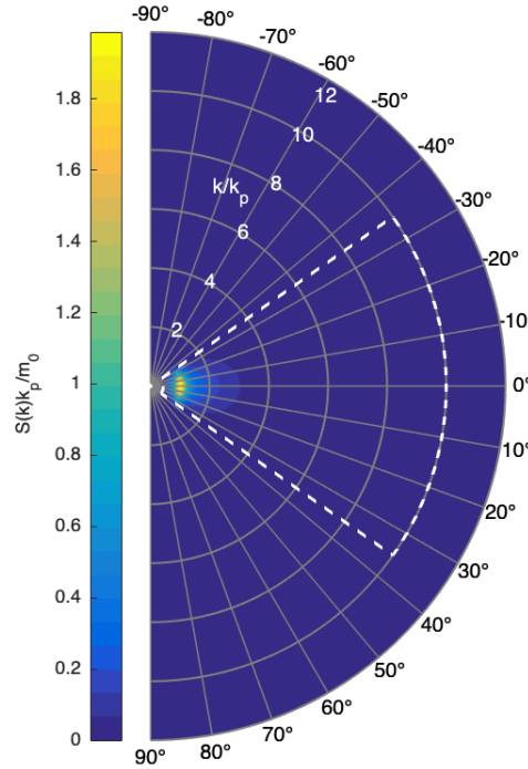
Figure IV.7: Directional wavenumber spectrum of the generated short-crested wave field. The dashed lines mark the spectral boundaries used in the wave model to perform the predictions.
