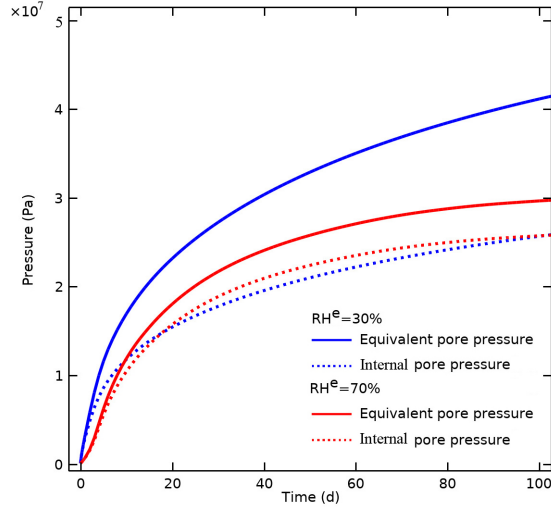
Figure 4.7: Comparison of internal pore pressure with equivalent pore pressure
