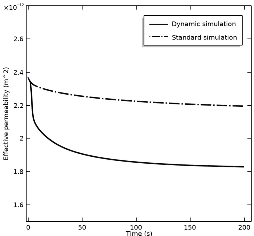
Figure 2.12: Evolution of average permeability with E = 1 \times 10^4 Pa
