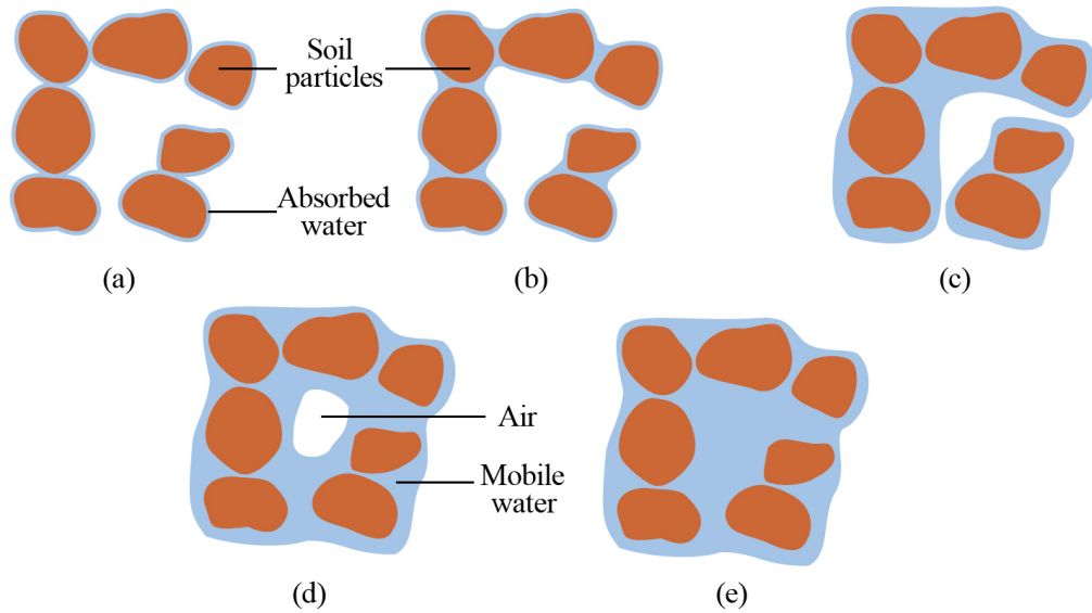
Figure 1.2: Configurations of water and air in soil (sand): (a) absorbed regime, (b) capillary pendular regime, (c) capillary funicular regime, (d) occluded air bubble regime, (e) fully saturated regime (taken from [2])
