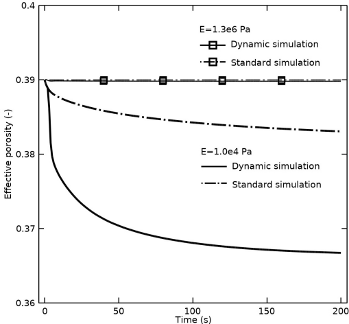
Figure 2.11: Comparison of average effective porosity with E = 1.3 \times 10^6 Pa and E = 1 \times 10^4 Pa
