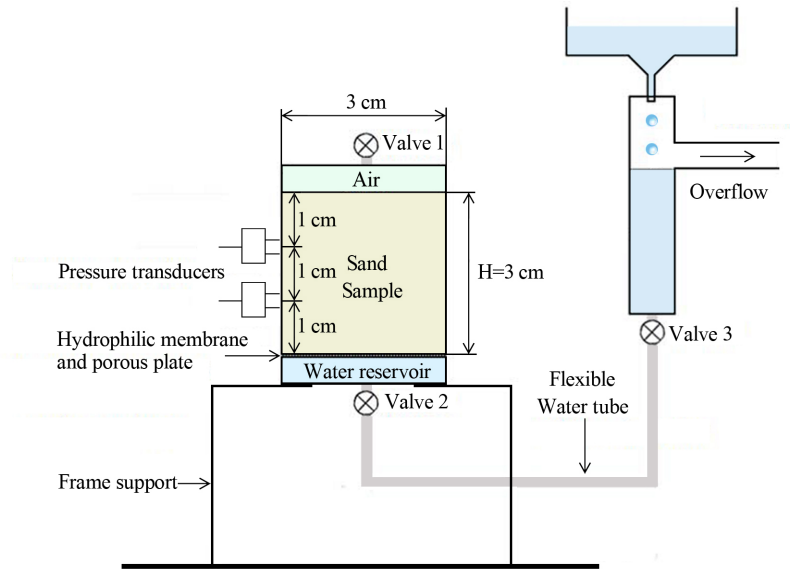
Figure 2.2: Schematic representation of sand drainage [10]
