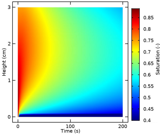
Figure 2.8: Water saturation as a function of height and time
