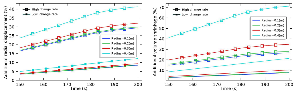
(a) Percentage of additional radial displacement (b) Percentage of additional volume shrinkage
