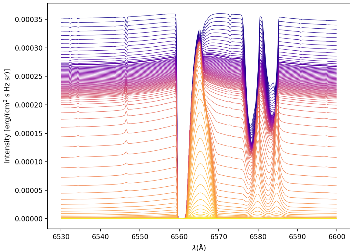
Figure 4.4 – Intensity profiles, as a function of the wavelength ( \sim 6530 – 6600 Å, around H\alpha ), calculated by myself using CMFGEN with the following stellar and wind parameters: \log L_*/L_\odot = 5.73 , T_{\text{eff}} = 18700 K, \log g = 2.3 , R_* = 70.6 R_\odot , \dot{M} = 1.0 \times 10^{-5} M_\odot \text{ yr}^{-1} , and v_\infty = 185 \text{ km s}^{-1} . Intensity profiles are shown for each value of distance from the center of the star (in total, 115 points). Lighter (toward yellow) I versus \lambda profiles come from larger distances through the wind region (extension of 50 R_* ). See text for discussion.
