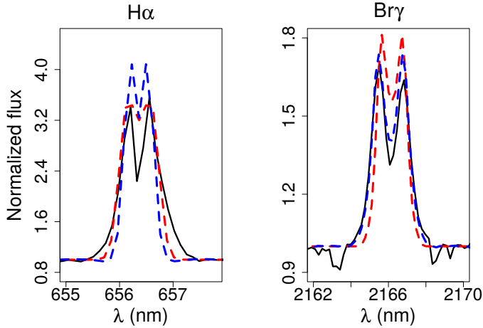
Fig. 12. Comparison between our best-fit kinematic models (dashed red; Table 2) and HDUST model (dashed blue, Table 5) in the H\alpha and Bry line profiles. Mean observed line profiles of H\alpha (BeSOS) and Bry (AMBER) are shown in black line. Our best-fit kinematic and HDUST models provide reasonable synthetic profiles to the observed ones in both H\alpha and B\gamma .
