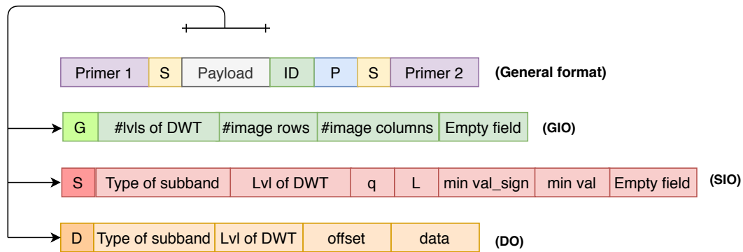
Figure 6.2: Proposed oligo formatting for a compression workflow that uses a DWT and a Uniform Scalar Quantizer
