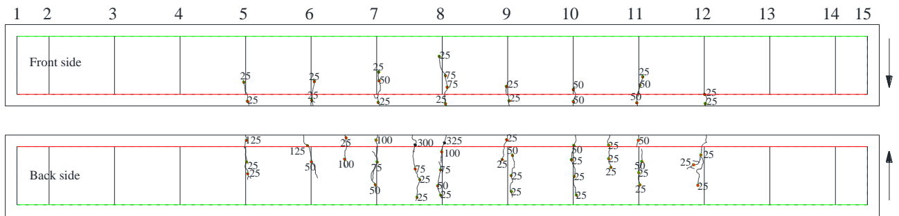
(a) Cracking situation on As01 beam at 28 days
