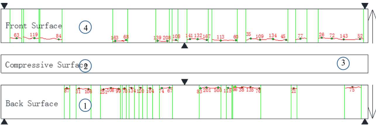
Figure IV-54.2 Cracking maps of beam C2 after 38 months
