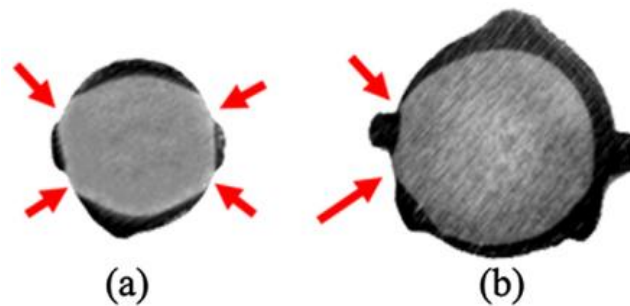
Figure II-20 Poor quality rebars exhibiting (a) discontinuities and (b) eccentric TM phase[122]
