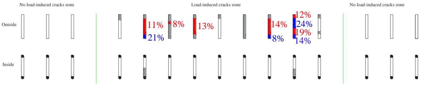
(b) Horizontal legs in tensile zone of beam As02
