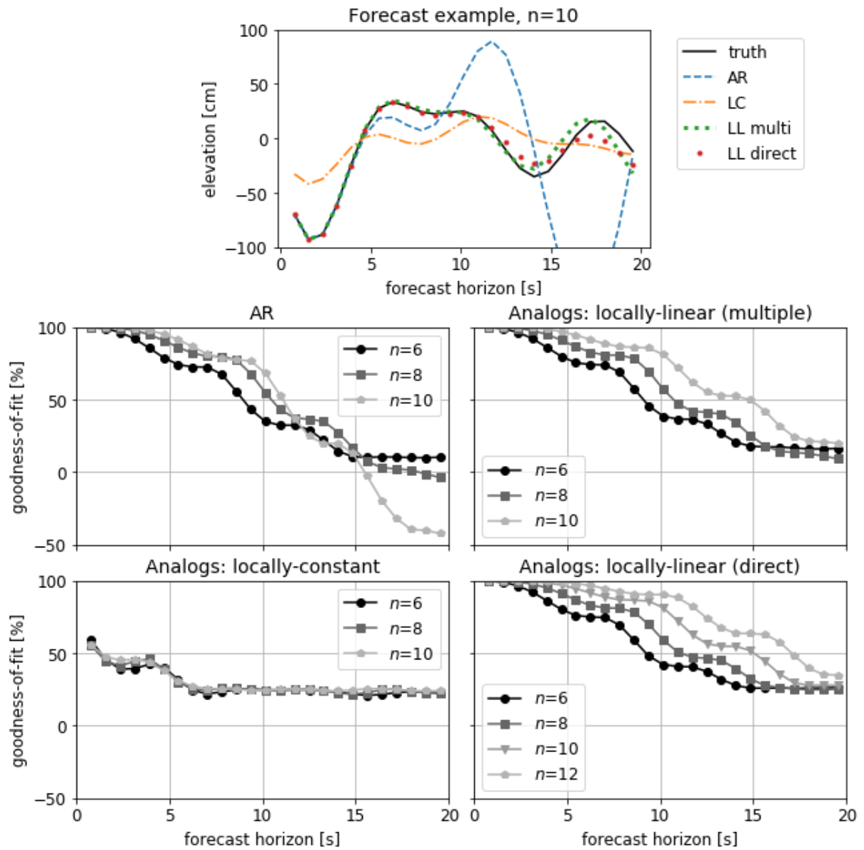
Figure III.12: Results of different forecasting strategy on ocean wave point-measurements from 30-minutes buoy sample described in Fig. III.11. The number of time-delays (or length of time-window) is n .
