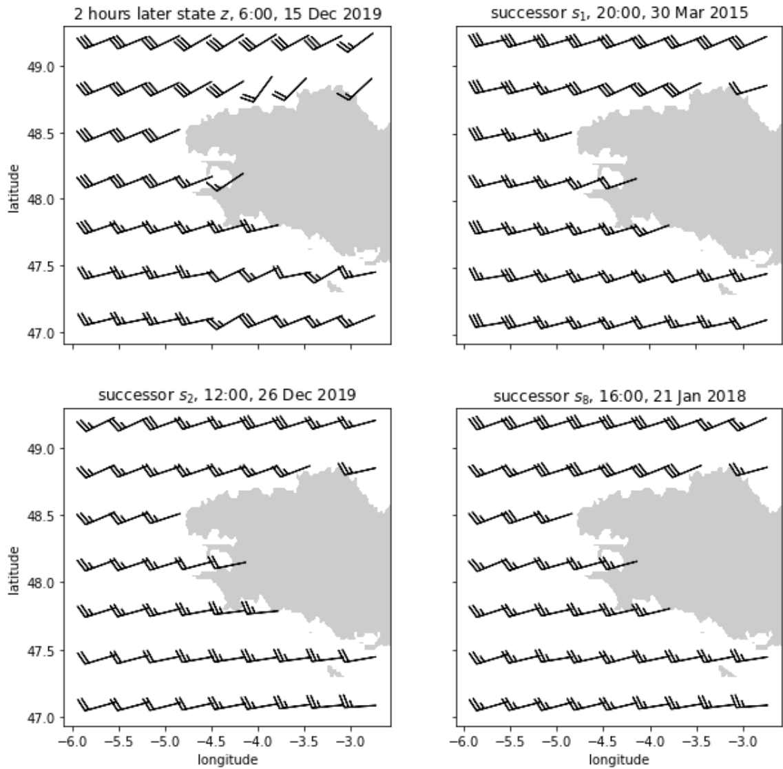
Figure II.10: Wind maps from Fig. II.6, two hours later. The target state is replaced by a "future state". Analogs are replaced by "successors" that can help estimate the "future state".
