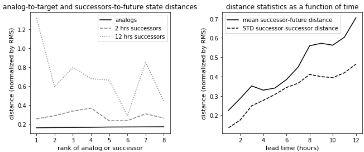
Figure II.12: All quantities plotted here correspond only to the example shown in Fig. II.6, Fig. II.10 and Fig. II.11, and not to statistics over many points. Left: distance from target wind map (respectively, future wind map) to analog wind map (respectively, successor wind map) as a function of analog rank (ordered of analog-to-target initial distances) for the lead times of two and twelve hours. Right: statistics of analog-to-target and successor-to-future state distances (full), and statistics of analog-to-analog and successor-to-successor distances (dashed).
