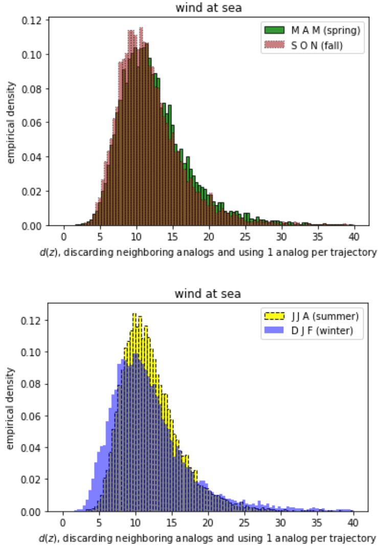
Figure II.5: Empirical probability density functions of local dimensions from 10m-wind data in the Iroise sea. We use the method of Caby et al. (2019), just like in Fig. II.1. The distributions of spring, fall (top panel) and winter (bottom panel) are similar. A small difference is seen in summer (bottom panel) with a more peaked distribution of dimensions, and a mean dimension slightly higher.
