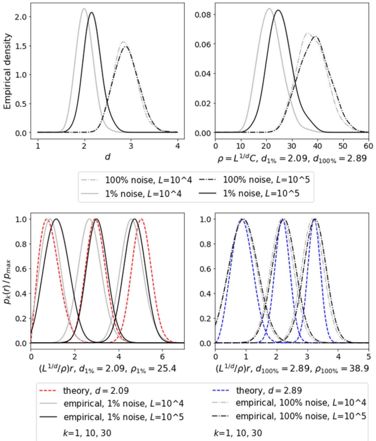
Figure II.9: Applying the aforementioned methodology to noisy catalogs of Lorenz's attractor (1963).
