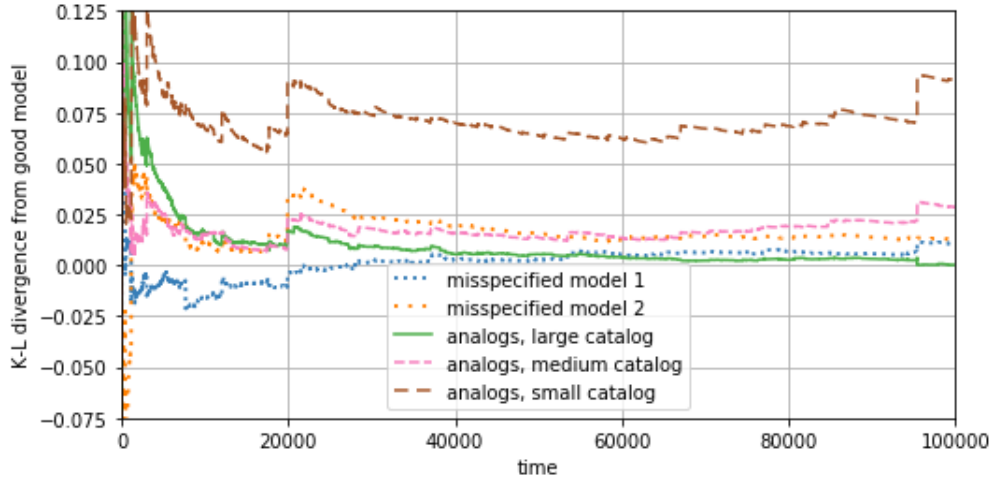
Figure V.3: Difference of forecast score between several methods, all using particle filters, and the reference classical particle filtering technique using the real model equation (V.2), averaged over t forecasts.
