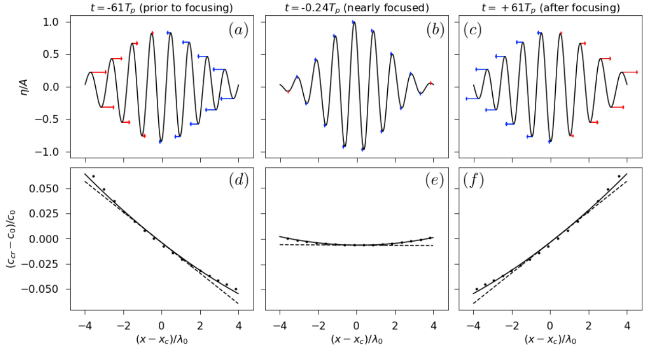
Figure IV.1: Crest and trough velocities of a Gaussian wave packet (GWP) at different times under linear evolution. The GWP is moving from left to right, and we assume the dispersion relation of deep-water gravity waves. The peak phase velocity is noted c_0 . Extracted from the numerical experiments described in Sect. 2.4, with L_f k_0 = 10 . Abscissa : position relative to the center of the GWP normalized by the peak wavelength \lambda_0 = 2\pi/k_0 . Black curves in (a – c) are a numerical approximation of \eta_G calculated using Eq. (IV.1). Arrows in (a – c) have lengths proportional to c_{cr} - c_0 , red when c_{cr} > c_0 and blue when c_{cr} < c_0 . Black dashed lines in (d – f) are a first-order approximation of the analytical prediction c_{sp}^a . Black curves in (d – f) are second-order approximation. Black dots in (d – f) are crest velocities c_{cr} extracted from numerical experiment. Shown are the situations prior to focusing (a and d), nearly focused (b and e), after focusing (c and f).
