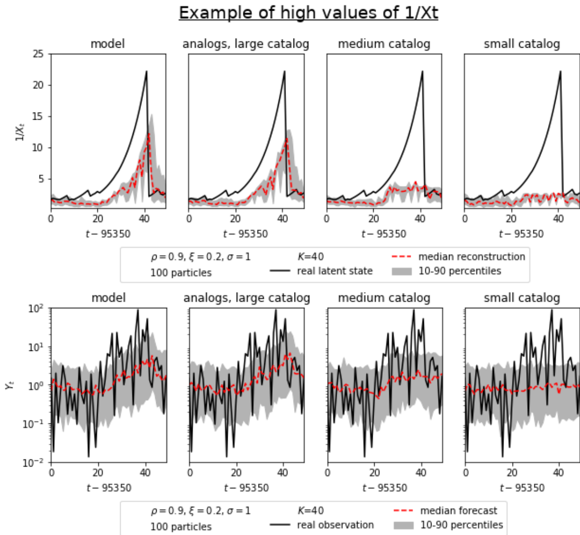
Figure V.4: Same as Fig. V.2 but for large values of the inverse latent state 1/X_t that cause average scores of different methods to jump (see Fig. V.3 around t \approx 95000 ).
