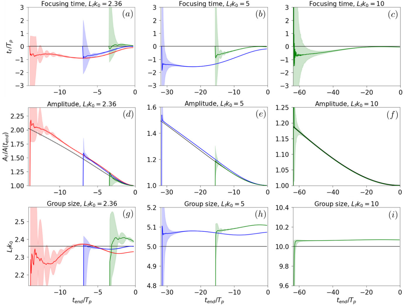
Figure IV.5: Estimation of focusing time t_f (a – c), ratio of focusing amplitude and instantaneous amplitude A_f/A(t_{end}) (d – f), and group focusing size L_f (g – i), following the methodology described in Sect. 2.4.4. The objective (truth) is represented in each subplot by a black line. Estimations are based on approximate measurements of \partial_x c_{sp}|_{x=x_c} between t_{start} and t_{end} , with t_{start} = -4|\tau| (red) or t_{start} = -2|\tau| (blue) or t_{start} = -|\tau| (green). Experiments are repeated with different values of the phase \Phi drawn randomly between -\pi and \pi . The medians of predictions are shown in full lines and points between the 2.5 and 97.5 percentiles are shown in light shading. L_fk_0 = 2.36 for (a), (d) and (g); L_fk_0 = 5 for (b), (e) and (h); and L_fk_0 = 10 for (c), (f) and (i). Vertical scales of (g – i) are proportional to the value of Lfk_0 .
