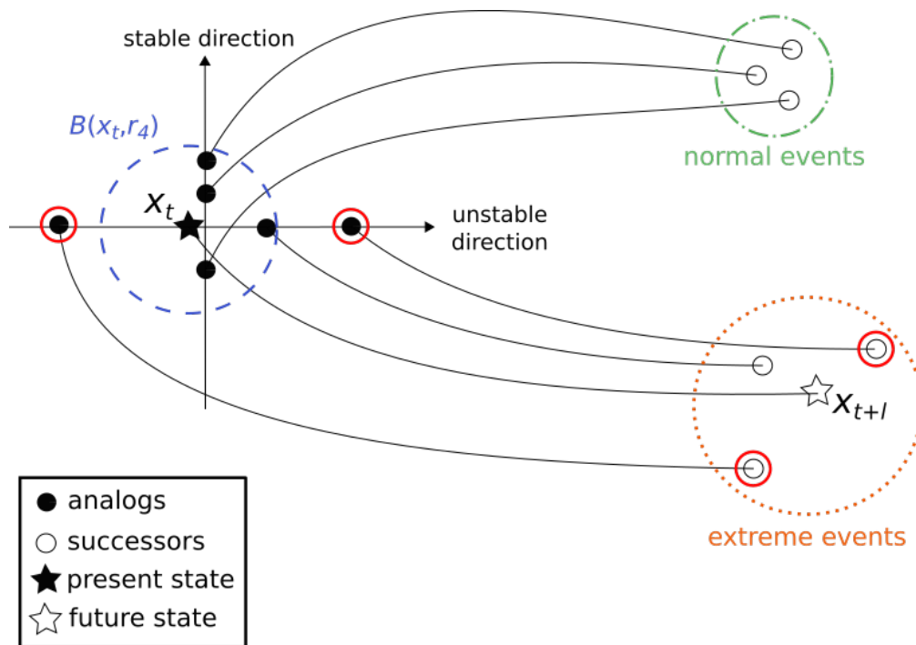
Figure V.7: A situation where classical sampling of analogs (with respect to distance) is suboptimal for the forecast of extremes. The two analogs circled in red are not taken into account if K = 4 , while they would have provided relevant information on the probability of encountering an extreme event.
