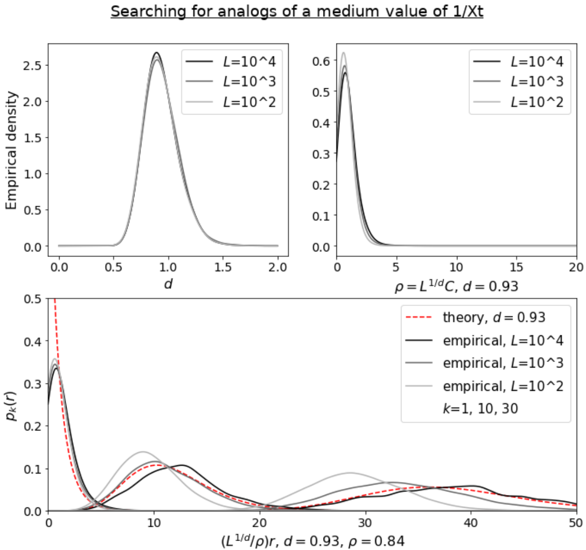
Figure V.5: Applying the methodology of Chapter II to heavy-tailed random variables. When searching analogs of values that are not in the tail of the distribution, the methodology seems to be applicable. In this figure, \rho is the scaling factor introduced in Chapter II, not the correlation parameter introduced in Chapter 5.
