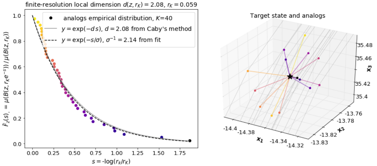
Figure II.1: Computing the finite-resolution local dimension d_{z,r_K} at a point z of the three-variable Lorenz (1963) system. Following from Caby et al. (2019), we evaluate d by taking the mean of the empirical cumulative distribution function shown in left panel. For this example, fitting the empirical CDF with an exponential \exp(-s/\sigma) and taking the inverse of \sigma would have given approximately the same value for d . The right panel shows the target z as a black star, and (one in three) analogs as colored dots (colors match the left panel). The trajectories from which the analogs are taken are in gray. In this example, the typical analog-to-successor distance is much larger than the typical analog-to-target distance.
