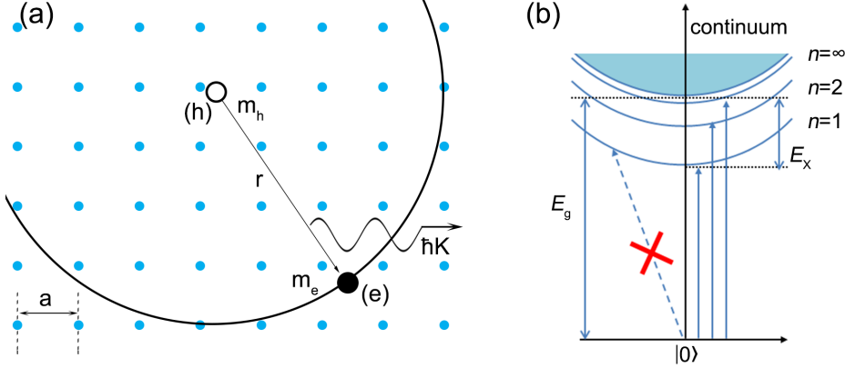
Figure 1.5: (a) Schematic showing a Wannier exciton in a crystal with lattice constant a . (b) The exciton dispersion relations E = E(K) for the ground and excited excitonic states. [Pelant 2012]
