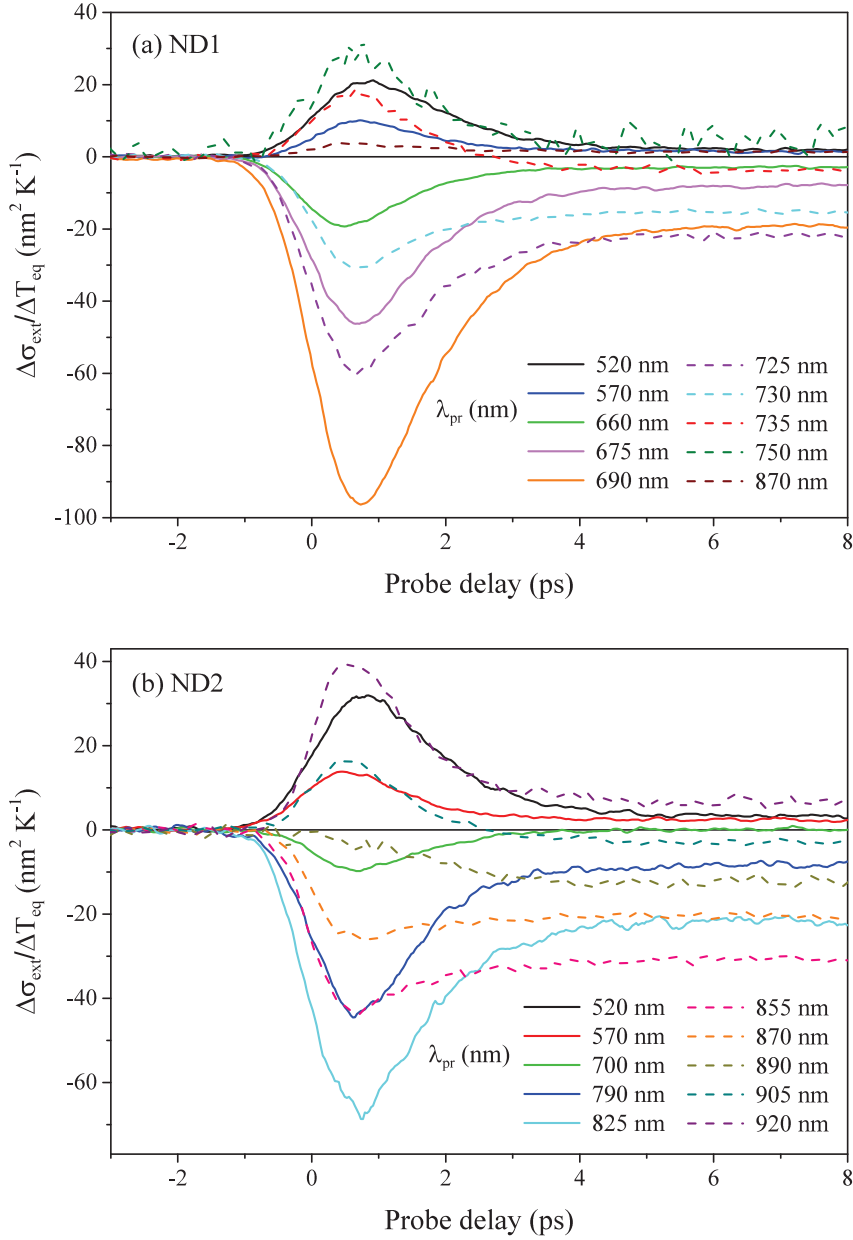
Figure 4.11 – Short-timescale time-resolved signals measured on gold nanodisks ND1 (a) and ND2 (b) at several probe wavelengths, as indicated in the legend. The extinction spectra of these NDs may be found in figure 3.9. The LSPR positions are \sim 715 nm and \sim 860 nm for ND1 and ND2, respectively.
